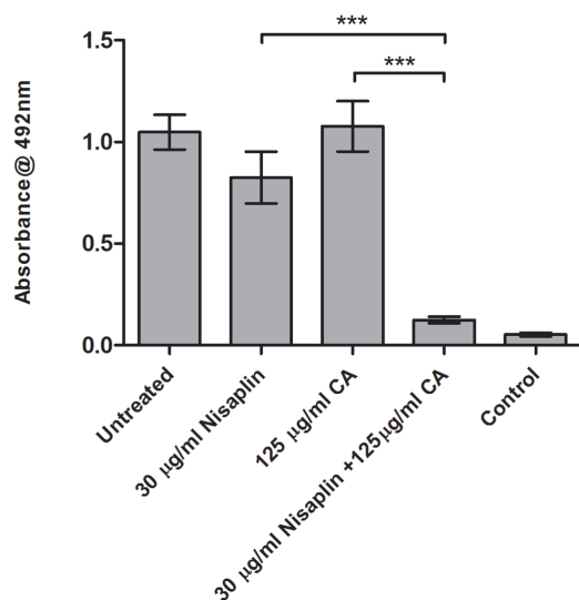
FIGURE 6 | Treatment of an established F6854 biofilm – Nisaplin® and cinnamaldehyde. Treatment of established (48 h) biofilms of L. monocytogenes F6854 with Nisaplin® and cinnamaldehyde (CN) alone and in combination. Treatment was over 24 h and performed in triplicate. Graph indicates the level of metabolically viable cells remaining following treatment as determined through XTT assay. *** P -value \leq 0.001 .
