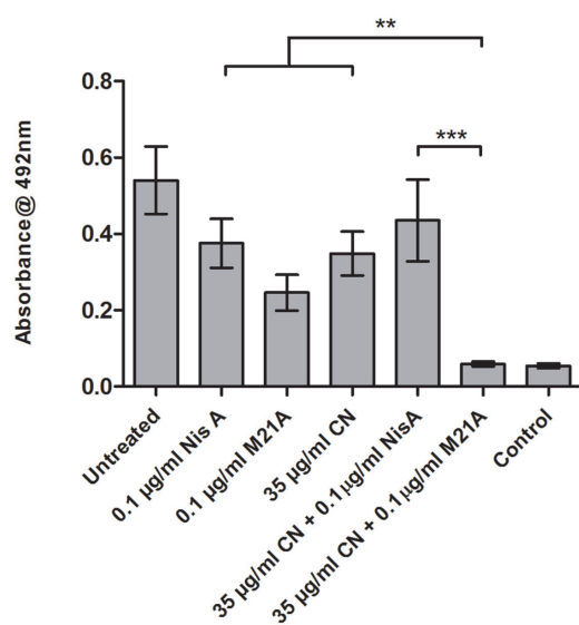
FIGURE 4 | Treatment of an established F6854 biofilm – NisA and M21A in combination with cinnamaldehyde. Treatment of established (48 h) biofilms of L. monocytogenes F6854 with M21A, nisin A (Nis A) and cinnamaldehyde (CN) alone and in combination. Treatment was performed in triplicate over 24 h. Graph indicates the level of metabolically viable cells remaining following treatment as determined through XTT assay. ** P -value ≤ 0.01; *** P -value ≤ 0.001.
