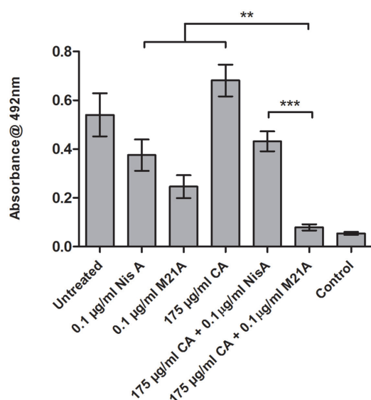
FIGURE 5 | Treatment of an established F6854 biofilm – NisA and M21A in combination with citric acid. Treatment of established (48 h) biofilms of L. monocytogenes F6854 with M21A, nisin A (Nis A) and citric acid (CA) alone and in combination. Treatment was performed in triplicate over 24 h. Graph indicates the level of metabolically viable cells remaining following treatment as determined via XTT assay. ** P -value \leq 0.01 ; *** P -value \leq 0.001 .
