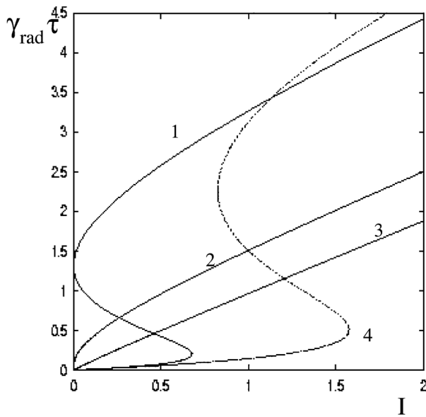
FIG. 7. Radiation rate from a silver nanoparticle on a substrate which provides optical gain, as a function of the normalized intensity of the external field for (curve 1): \kappa/\kappa_{th}=4 , (2): 1; (3): 0.1; and (4): for \kappa/\kappa_{th}=6 but n_m=3.1 , when the conditions for dipole lasing are not fulfilled.
