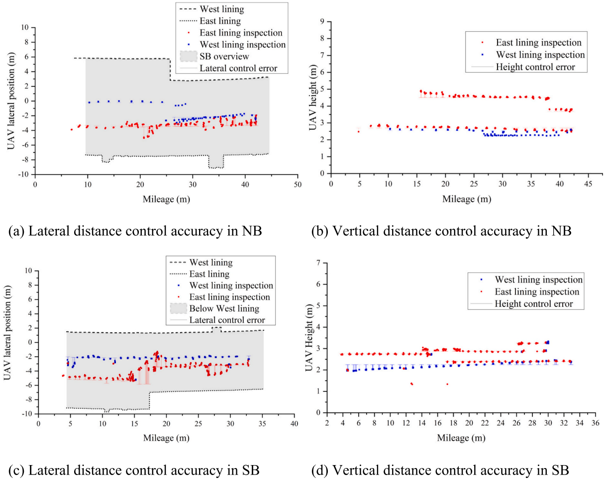
Fig. 13. UAV flying routes and control errors in the twin tunnels under coordinate system S' .
