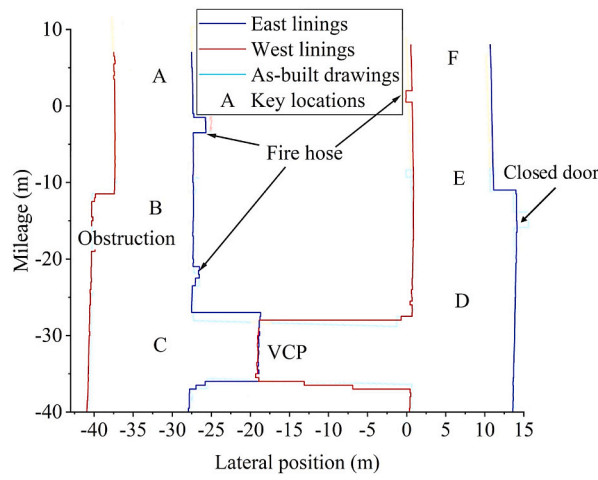
(b) Comparison of tunnel top view from DSM and as-built drawing
