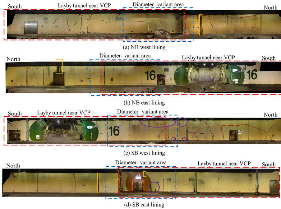
Fig. 19. Defect identification in the DSM from UAV images
