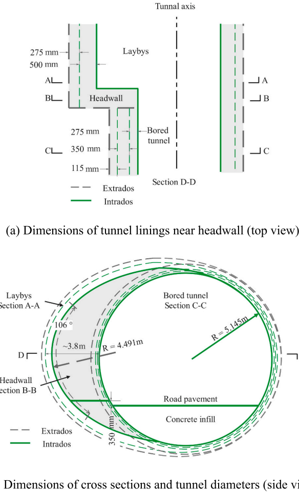
Fig. 16. Schematic of layby and bored tunnel geometry
