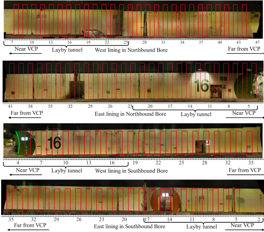
(b) Data extraction in four linings (tunnel mileage starts from VCP and is in the unit m)
