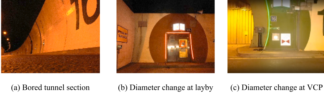
Fig. 2. Illustration of complex engineering geometry of the DPT section.
