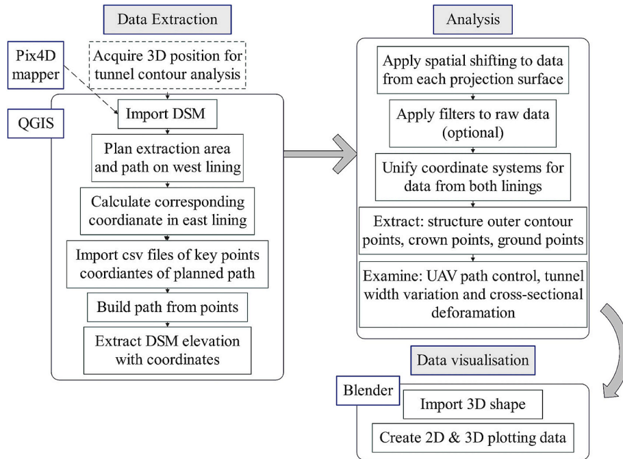
Fig. 10. Step-by-step workflow of data extraction and analysis from 3D tunnel models and software.
