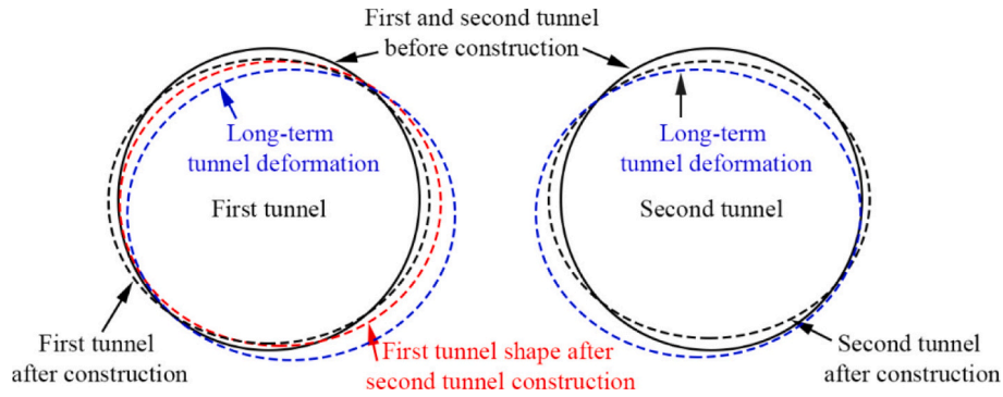
(a) Tunnel deformation under twin tunnel effect ([20])
