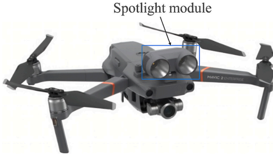
Fig. 4. UAV M2ED installed with DJI spotlight module.
