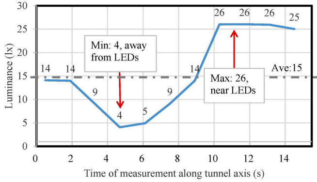
Fig. 3. Intensity variation of reflective light on tunnel side wall along DPT alignment.
