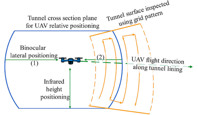
Fig. 5. Schematic of PMPP-SDI in tunnel surface information acquisition.
