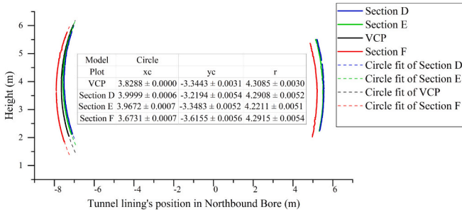
(c) Layby tunnels cross section comparison in NB
