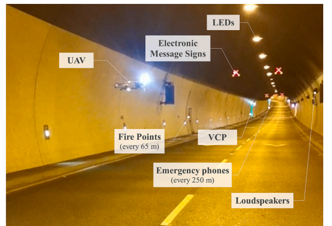
Fig. 6. Automatic UAV inspection of DPT.
