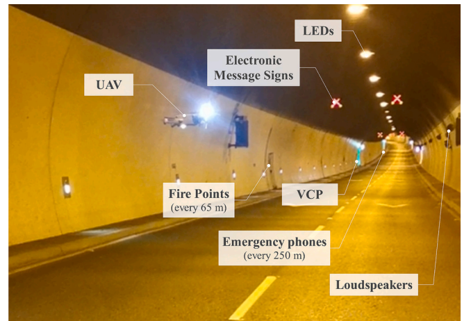
Fig. 6. Automatic UAV inspection of DPT.
