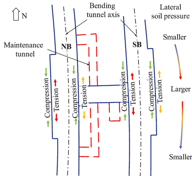
Fig. 20. Schematic of the tunnel construction plan
