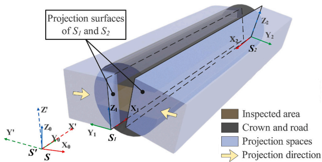
Fig. 11. Schematic of coordinate system unification ( S' ) from DSM data ( S_1, S_2 ) and software local ( S ) coordinate systems (by using the direction of S_1 and origin of S ).
