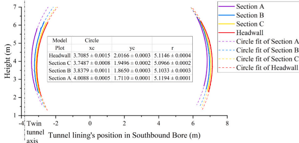
(b) Circular tunnels cross section comparison in SB
