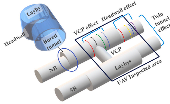
(a) Overview of data extraction at the cross-passage twin tunnel section
