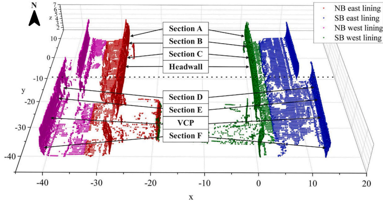
(a) 3D overview of extracted coordinates (m) with key cross section extraction locations
