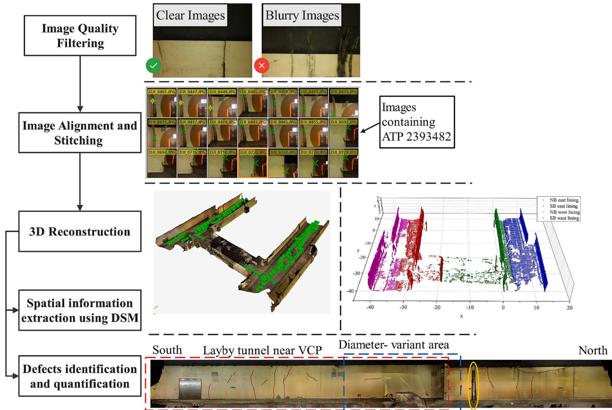
Fig. 8. Image processing workflow for DPT field test.
