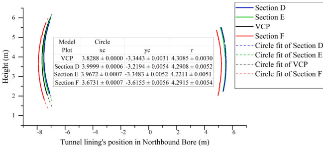
(c) Layby tunnels cross section comparison in NB
