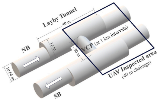
(b) Illustration of the cross-passage twin tunnel section
