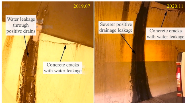
(a) Tunnel surface defects at VCP 16 [20]
