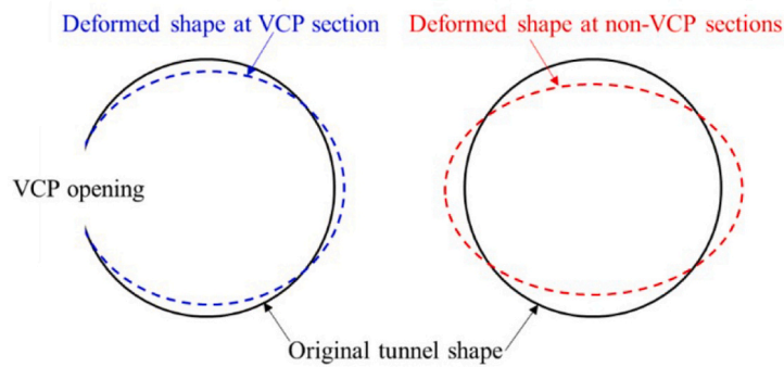
(b) Tunnel deformation under VCP effect (modified from [24])
