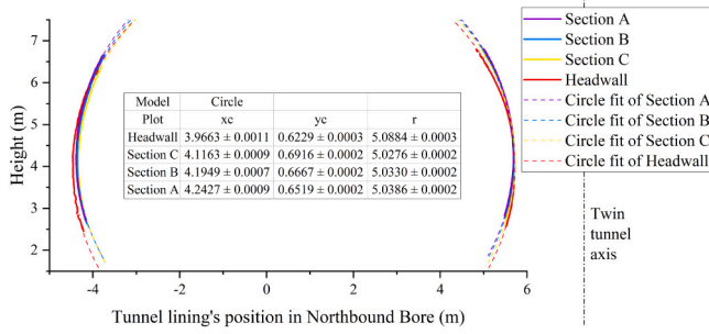
(a) Circular tunnels cross section comparison in NB
