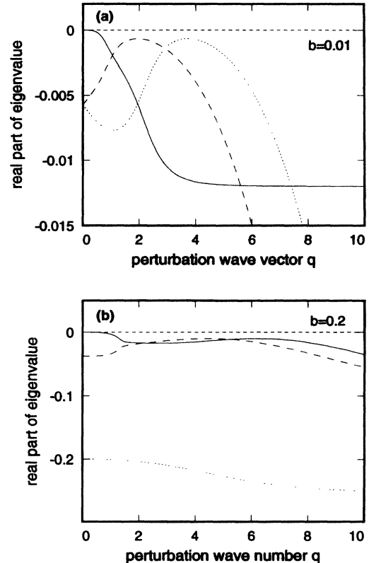
FIG. 3. Real parts of the three biggest eigenvalues obtained from the linearized MB equations about the traveling wave solution at k = 0.9 and r = 1.2 . (a) Stiff limit ( b = 0.01 ). (b) Nonstiff limit ( b = 0.2 ). The other parameters are unchanged. The two eigenvalues which are not shown have a real part close to -1 .
