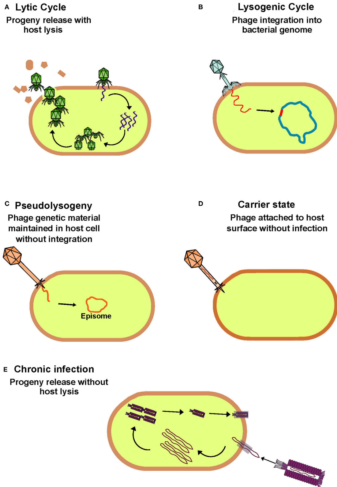
FIGURE 1 | Overview of bacteriophage lifecycles. (A) Lytic phages hijack host cell machinery to replicate, assemble and produce progeny which are released from the cytoplasm on host cell lysis to initiation further rounds of infection. This phage lifecycle is thought to be the most prevalent in the healthy human gut. (B) Lysogenic (Continued)
