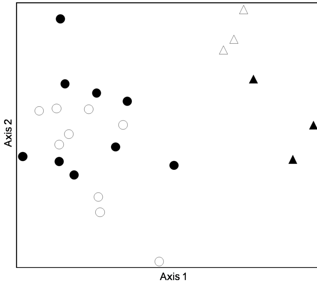
Figure 2. NMDS ordination of species assemblages at each treatment x woodland type plot. Oak (●), yew (▲). Unfilled = ungrazed plots, filled = grazed plots. Axis 1 = 66%, P = 0.02 . Axis 2 = 18%, P = 0.02 .
