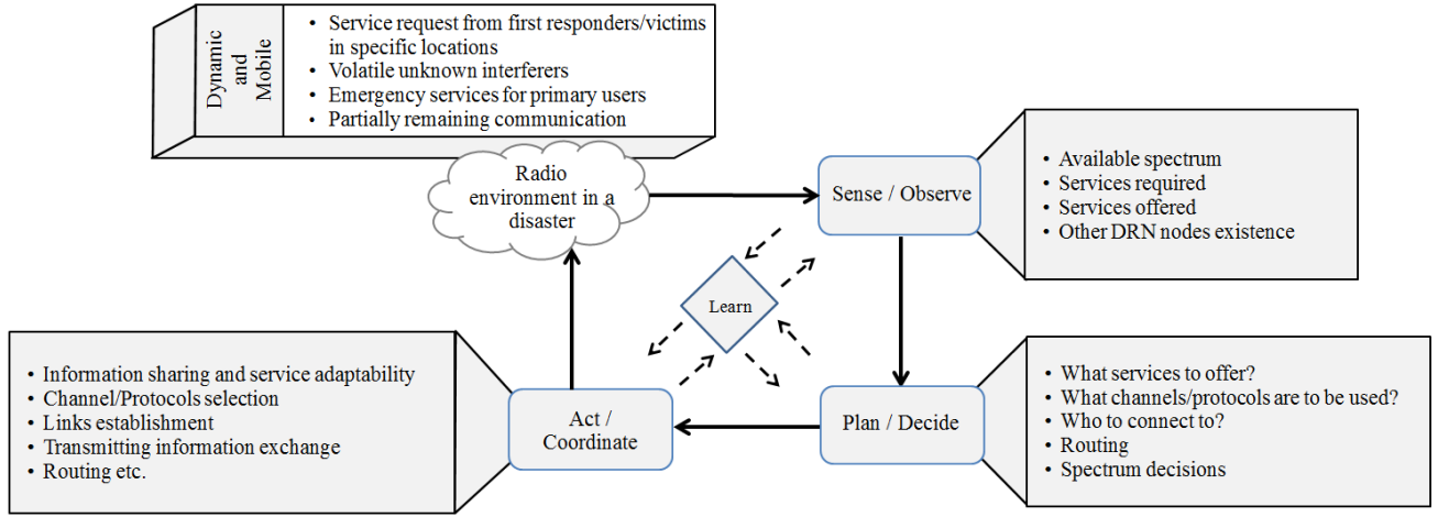
Fig. 1: Key cognitive radio mechanisms for disaster response network
