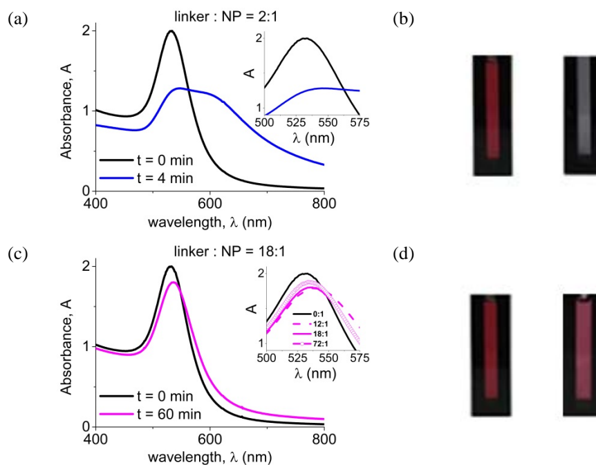
Figure 2.3: UV-visible absorption spectra of C-reactive protein (CRP) antibody functionalized 40 nm diameter gold nanoparticle solution to which (a) CRP antigen linker molecule-nanoparticle ratio = 2:1 and (c) CRP antigen linker molecule-nanoparticle ratio = 18:1. Corresponding photographs of C-reactive protein antibody functionalized 40 nm diameter gold nanoparticle solution taken (b) prior to addition of CRP antigen and 5 minutes following addition of CRP antigen solution (2:1), (d) prior to addition of CRP antigen and 5 days following addition of CRP antigen solution (18:1).
