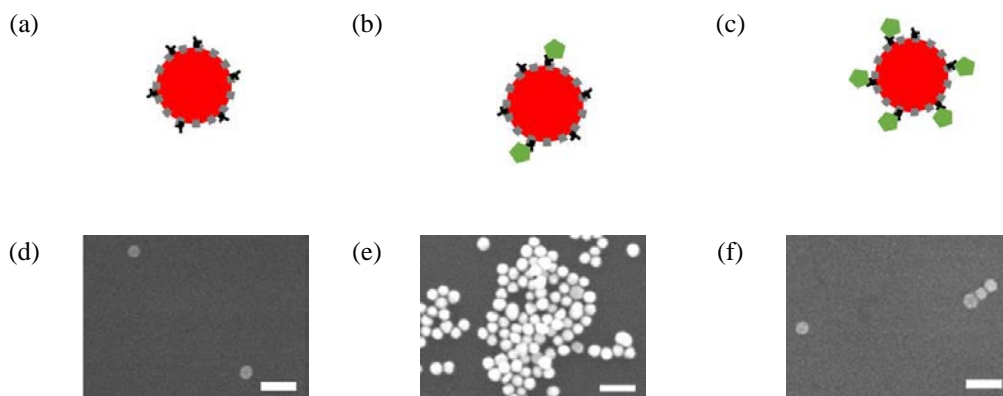
Figure 2.4: Schematics depicting the relative coverage of the antiCRP NPs with CRP antigen (a) antigen molecule-NP ratio = 0:1, (b) antigen molecule-NP ratio = 2:1 (c) antigen molecule-NP ratio = 18:1 and corresponding SEM images in (d), (e) and (f). SEM image scalebars = 120 nm.
