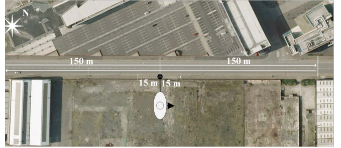
Fig. 3. Satellite view of the measurement environment showing the vehicle trajectories (white continuous lines with arrow heads) and pedestrian trajectory (white dashed line with arrow head) for the walking scenarios (note: image courtesy of Google Maps).
