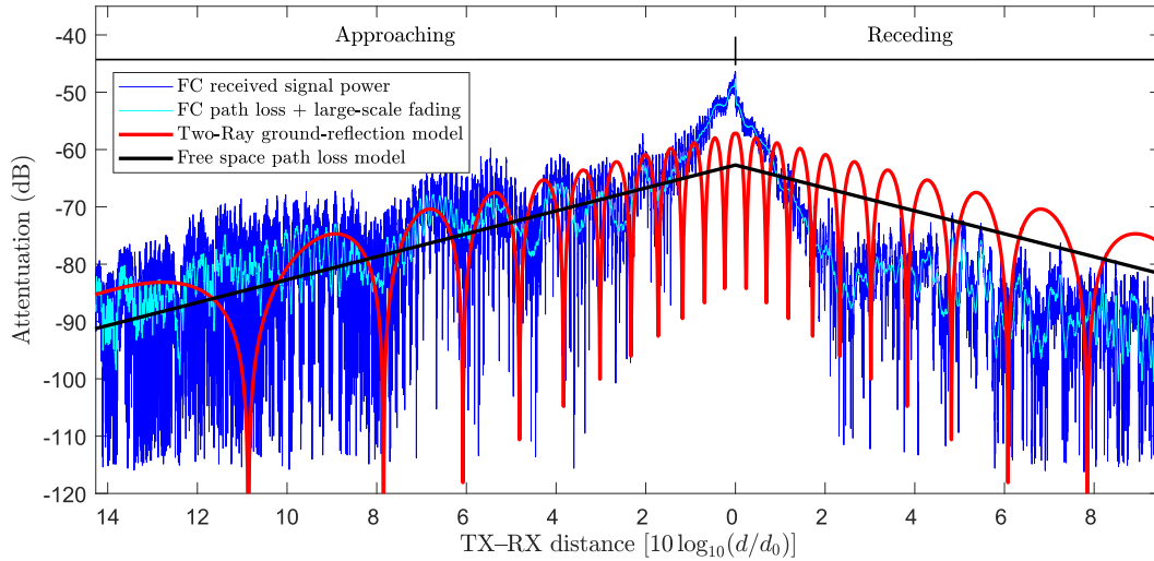
Fig. 6. Attenuation, extracted PL, and large-scale fading alongside the free-space path and two-ray ground-reflection PL models ( P_t = 0 dBm, G_t = G_r = 1 , h_t = h_C = 1.2 m, h_r = h_{FC} = 1.5 m, and \epsilon_g = 0.34 ) for the FC channel in Scenario A.
