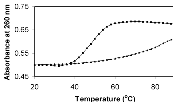
Figure 3. Normalized thermal dissociation curves for (black triangle) unmodified antiparallel triplexes formed from the hairpin \text{h}_{26}5'\text{-SH} and the oligonucleotide Hoog-GA5'-SH and for (black square) antiparallel triplex-nanoparticle aggregates formed using oligonucleotide-nanoparticle conjugates based on the same sequences.
