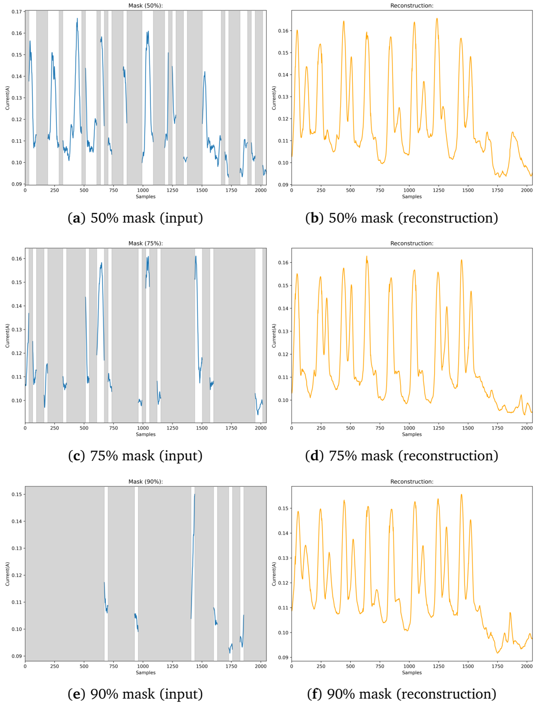
Figure 6.12: Reconstruction of the same normal Bluetooth segment under varying inference masking ratios (rows: 50%, 75%, 90%). Left: masked inputs. Right: corresponding reconstructions.
