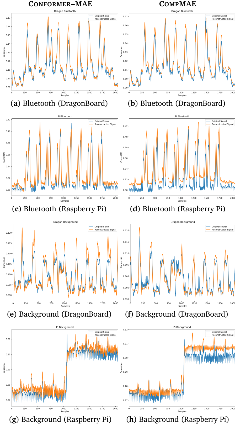
Figure 6.13: Reconstruction of normal power behaviour across devices and activities. Left column: CONFORMER-MAE baseline. Right column: COMPMMAE.
