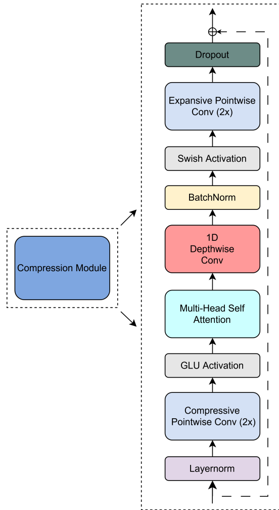
Figure 6.8: Compression module used in COMPMAE. Note the similarities to the convolutional module, albeit inverted in key areas.
