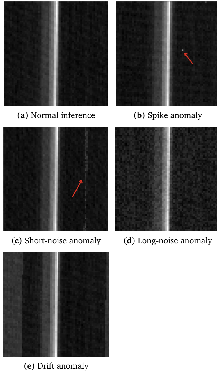
Figure 3.7: Road-sign CNN inference represented as grayscale images. The normal inference (top-left) is shown alongside injected anomaly types: spike, short-noise, long-noise, and drift. Distortions introduced by each anomaly are visually apparent in the corresponding panels.
