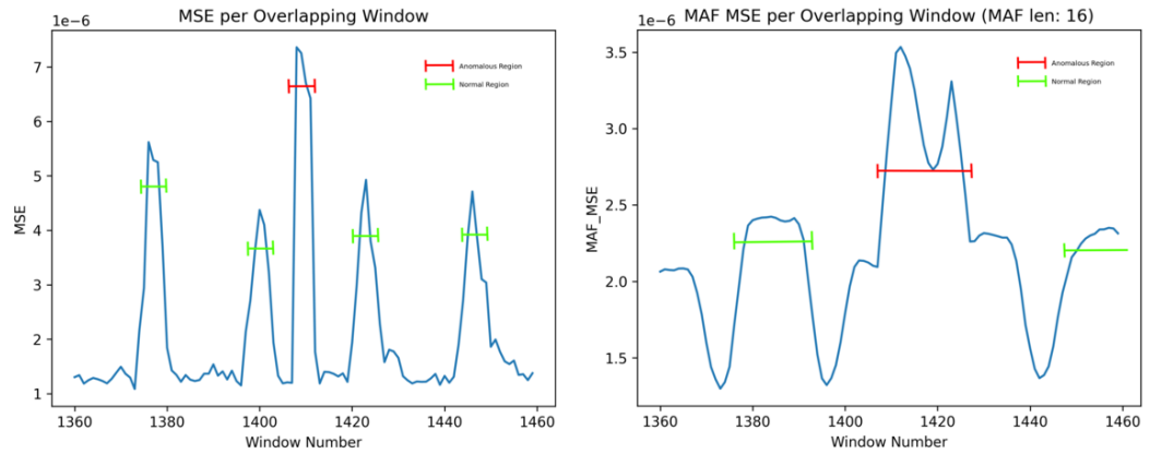
Figure 5.6: Effect of the Moving Average Filter (MAF) on the mean squared error (MSE) signal. MAF smoothing broadens anomaly responses and reduces false positives in normal regions.
