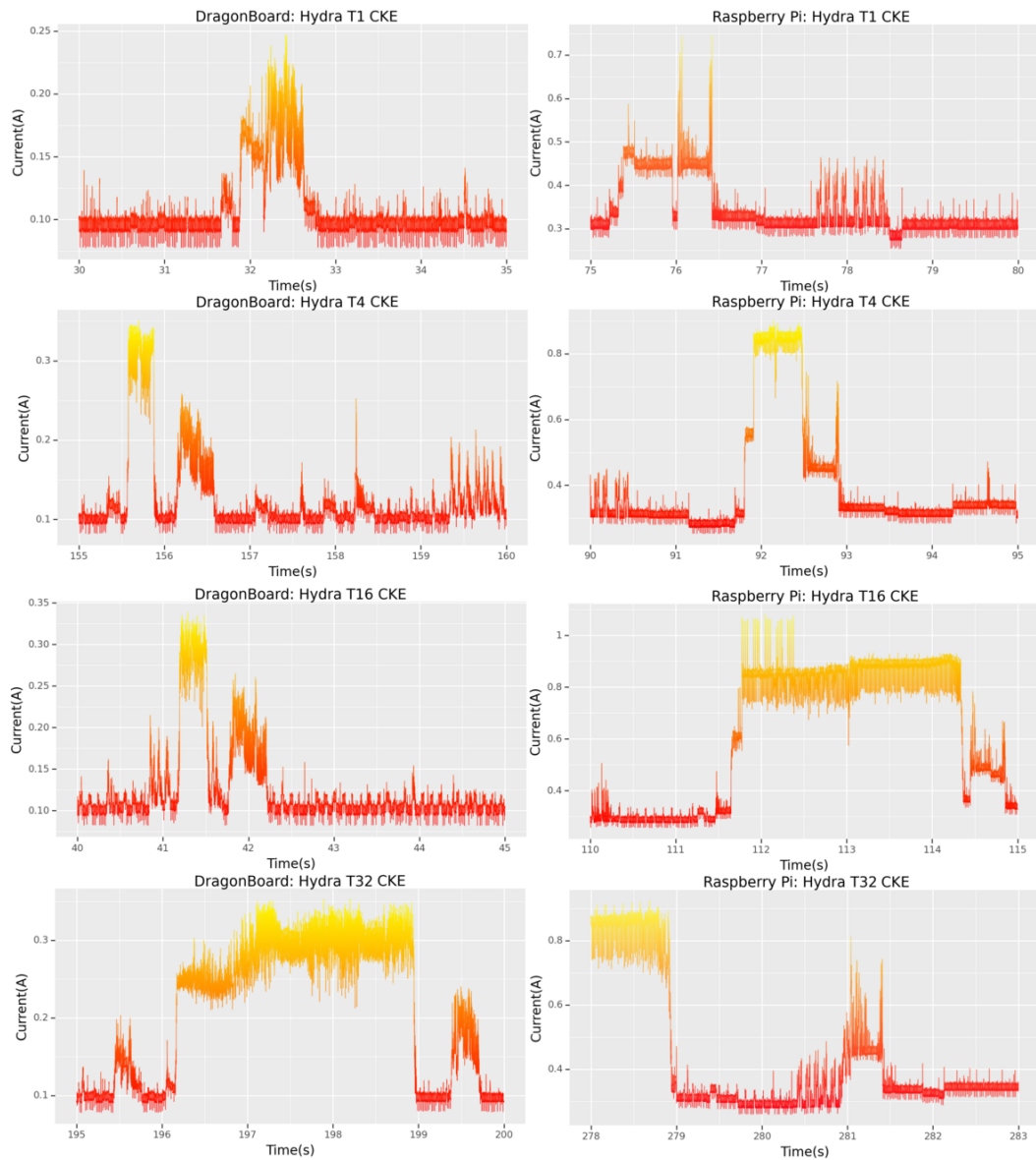
Figure 4.5: Correct Key Events (CKE) across all Hydra t -switch configurations for the DragonBoard and Raspberry Pi (data visualised using the “autumn” colormap [119]).
