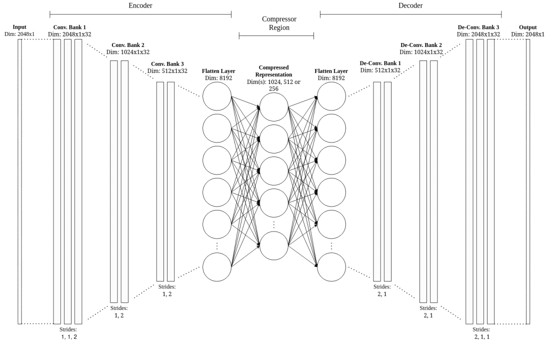
Figure 5.4: Convolutional Autoencoder (CAE) architecture used in this Chapter.
