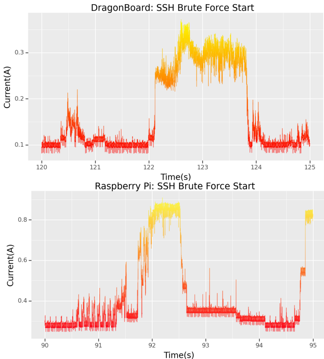
Figure 4.9: Start of the SSH brute-force phase during the CTF, comparing DragonBoard and Raspberry Pi (data visualised using the “autumn” colormap [119]).
