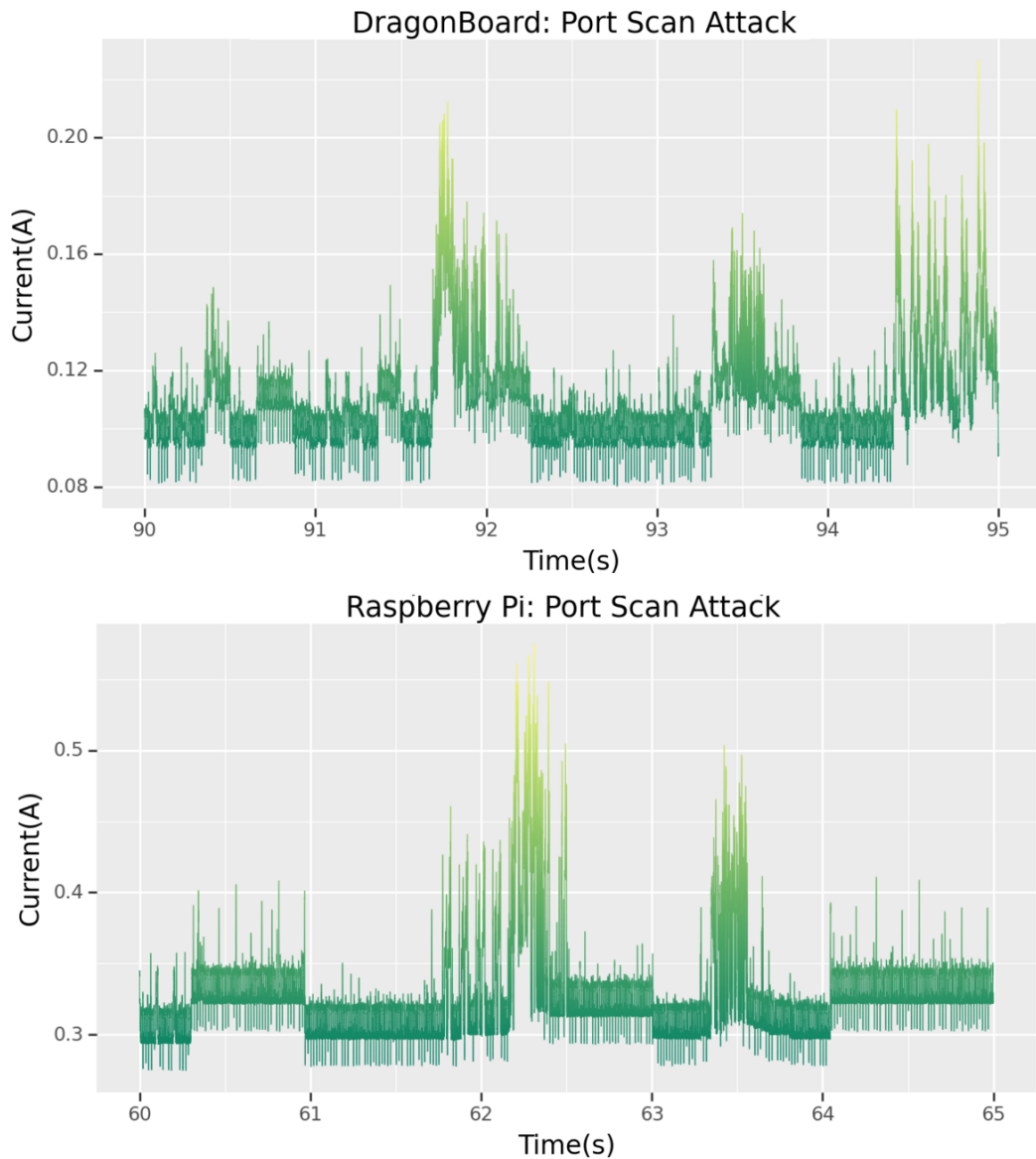
Figure 4.8: Comparison of Nmap behaviour during the CTF between the DragonBoard and Raspberry Pi (data visualised using the “summer” colormap [119]).
