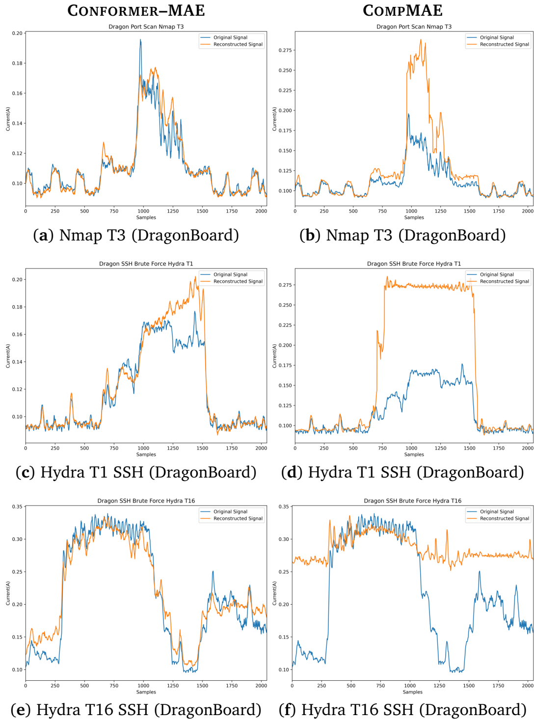
Figure 6.14: Reconstruction behaviour of CONFORMER-MAE (left column) and COMPMMAE (right column) on selected anomalous DragonBoard events from the DRAGON_PI dataset.
