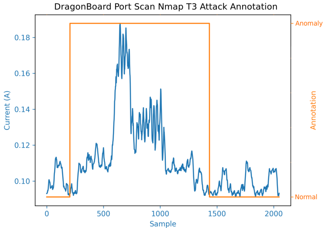
Figure 4.16: Example of annotation accuracy from the dataset.
