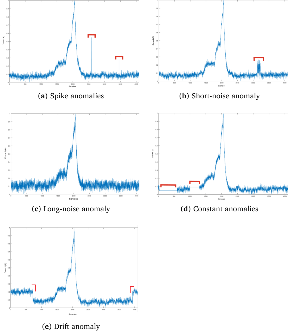
Figure 3.6: Road-sign CNN inference traces with injected anomalies. Spike, short-noise, and long-noise disturbances are shown alongside constant and drift anomalies. Red annotations indicate injected regions.
