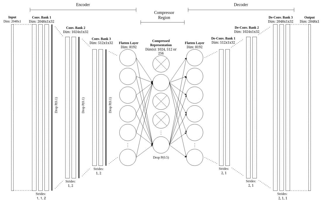
Figure 5.9: Revised CAE architecture incorporating dropout regularisation. Dropout is applied after GELU activations in both convolutional and dense layers, with dropout probabilities of 0.1 and 0.5, respectively.
