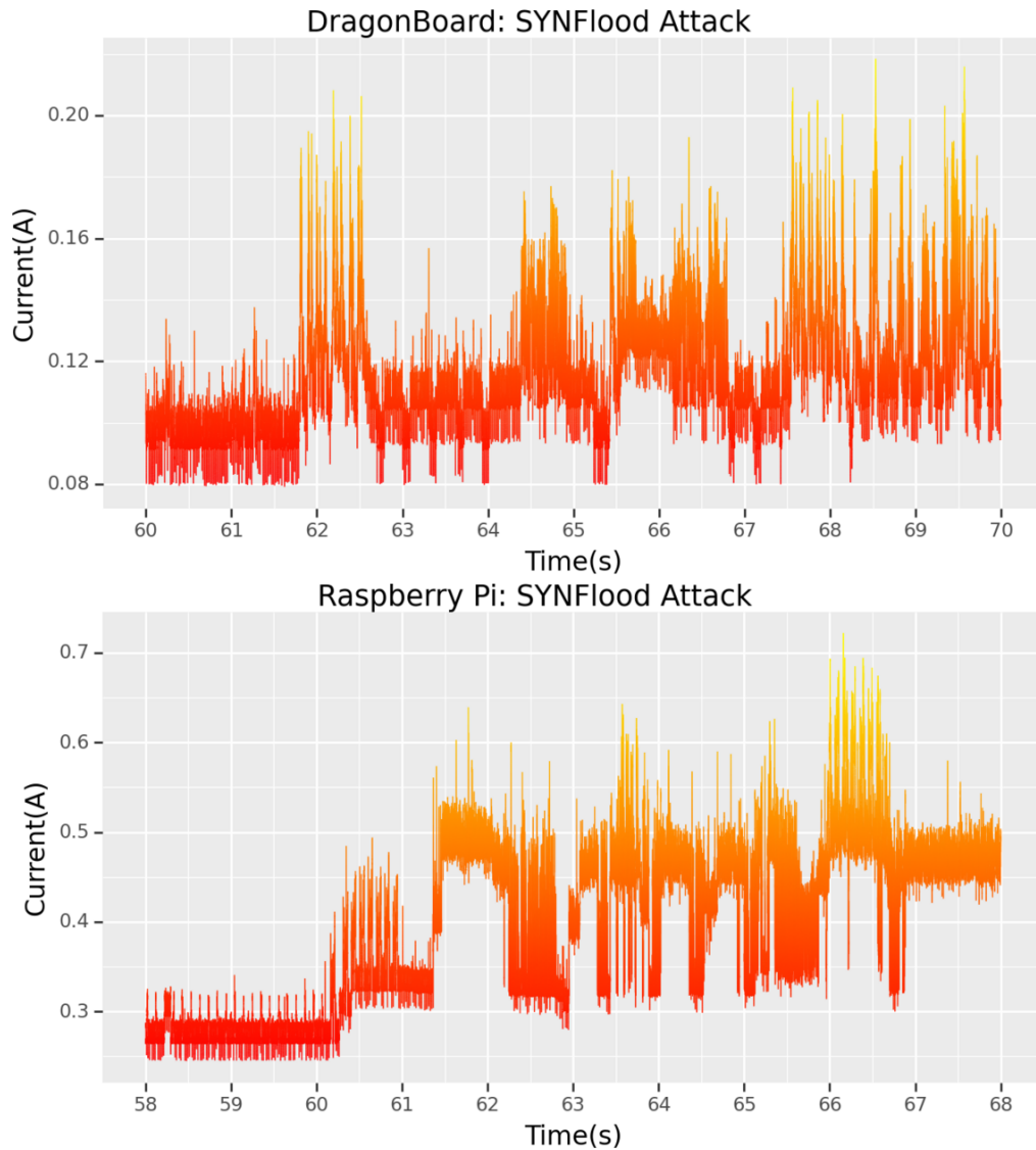
Figure 4.6: Comparison of SYN flood attacks on the DragonBoard and Raspberry Pi (data visualised using the “autumn” colormap [119]).
