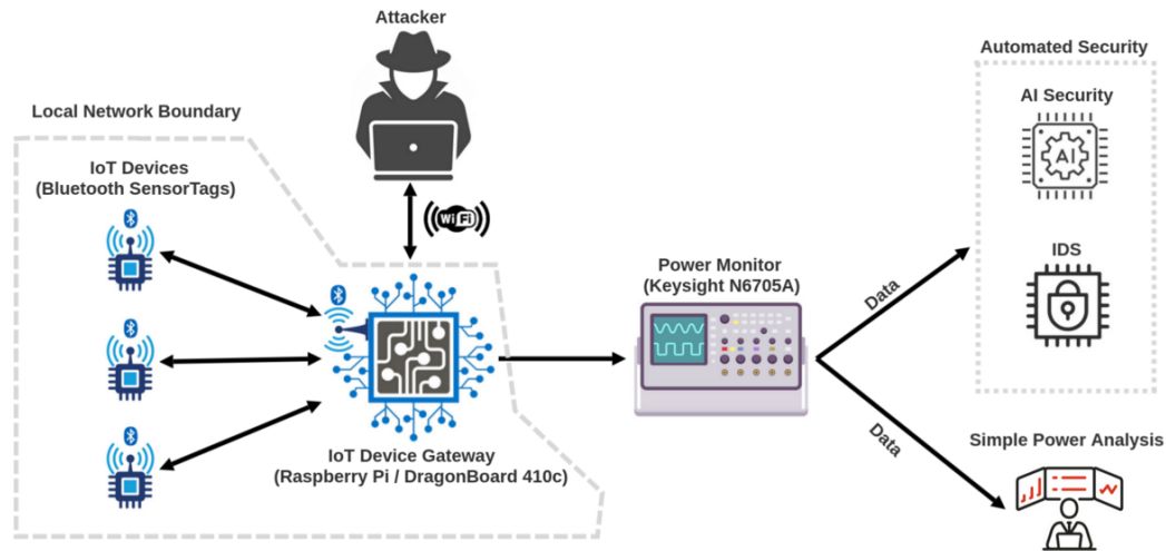
Figure 4.1: IoT power data acquisition framework used in this Chapter, illustrating the balance between human-in-the-loop oversight and automated (AI-driven) security analysis.
