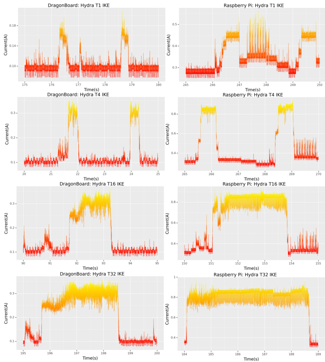
Figure 4.4: Incorrect Key Events (IKE) across Hydra t -switch settings for the DragonBoard and Raspberry Pi (data visualised using the “autumn” colormap [119]).
