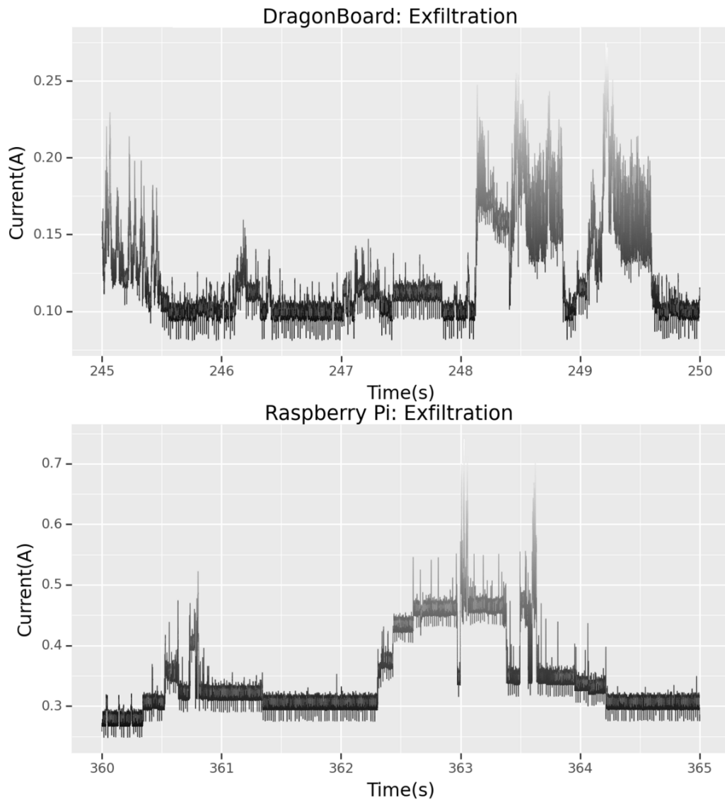
Figure 4.13: Exfiltration during the CTF for the DragonBoard and Raspberry Pi (data visualised using the “gist_gray” colormap [119]).
