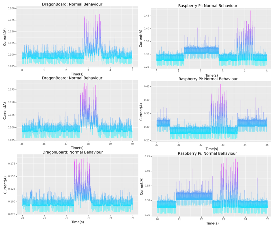
Figure 4.2: Normal power signatures for the DragonBoard and Raspberry Pi. Note the strong similarity in signature shape between the two devices despite the amplitude difference.
