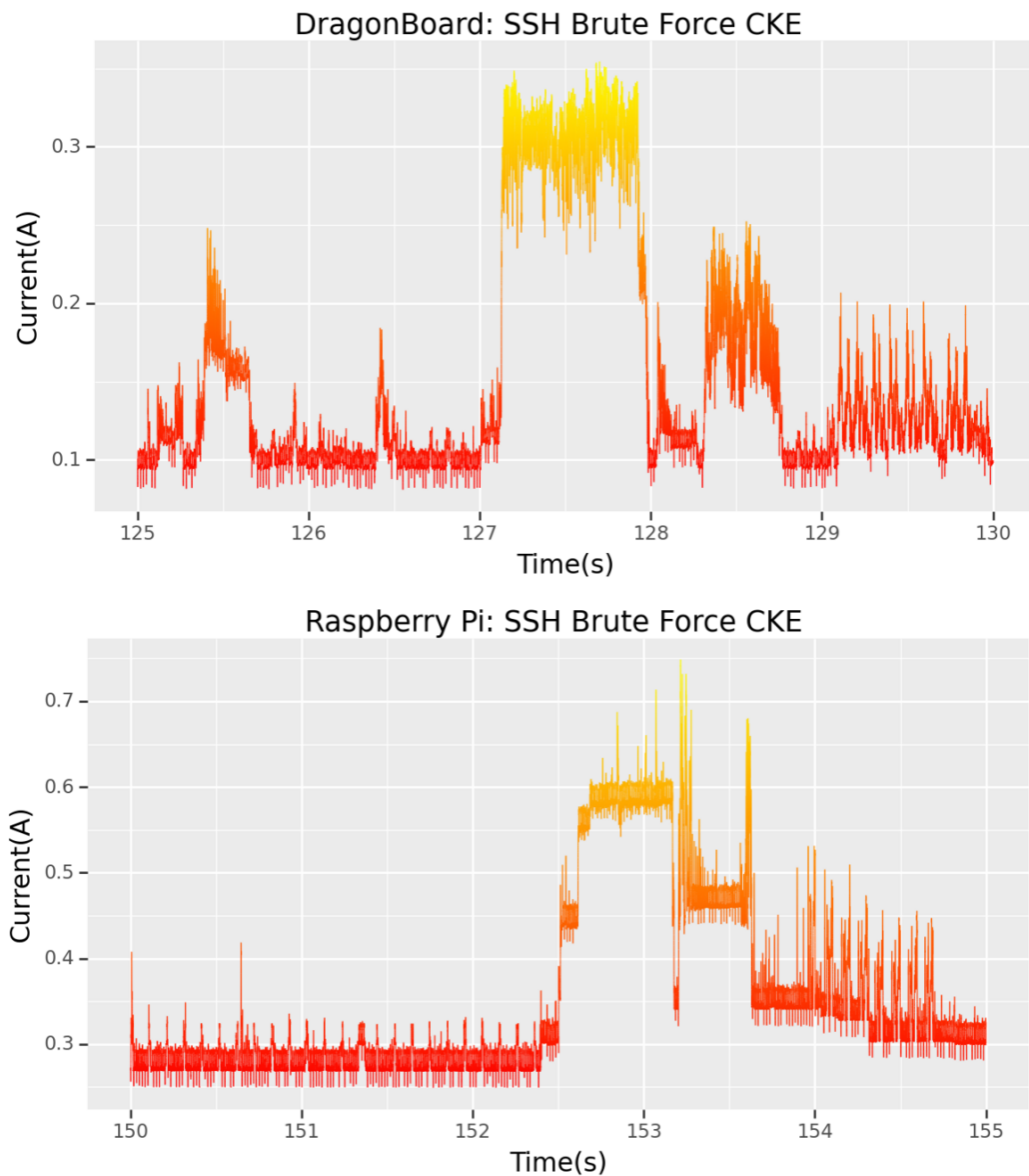
Figure 4.10: Comparison of Correct-Key Events during the CTF for the DragonBoard and Raspberry Pi (data visualised using the “autumn” colormap [119]).
