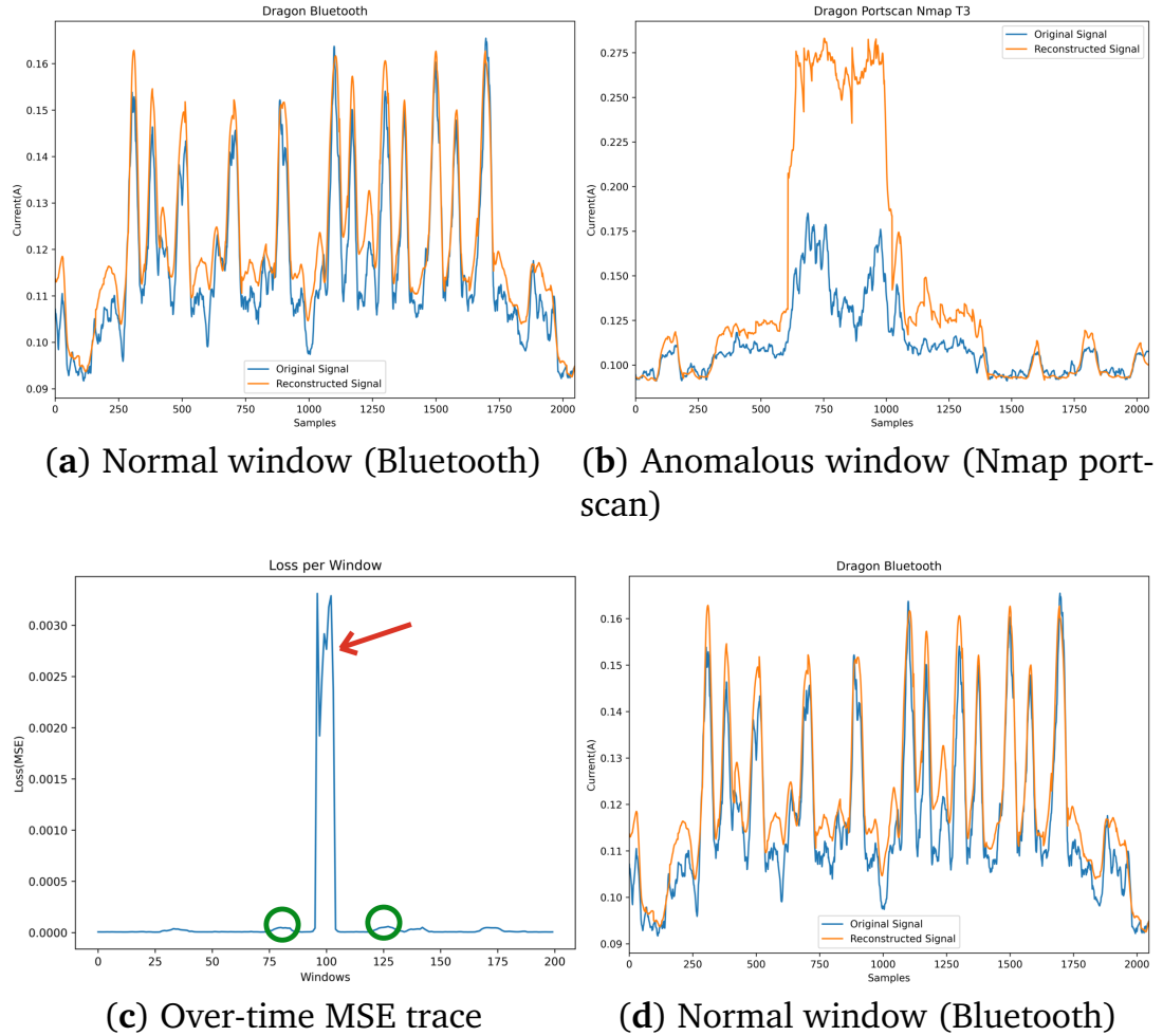
Figure 6.17: Reconstruction behaviour of COMPMAE across 200 windows. Normal windows are reconstructed with high consistency and consequently low error, as seen in adjacent normal windows A and D (highlighted in green), whereas the Nmap anomaly produces a strong divergence and a large, easily identifiable peak in the MSE trace (annotated by the red arrow).
