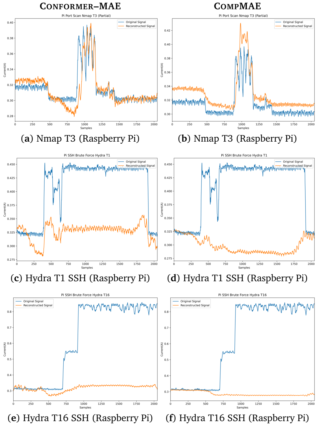
Figure 6.15: Reconstruction behaviour of CONFORMER-MAE (left column) and COMPMMAE (right column) on selected anomalous Raspberry Pi events from the DRAGON_PI dataset.
