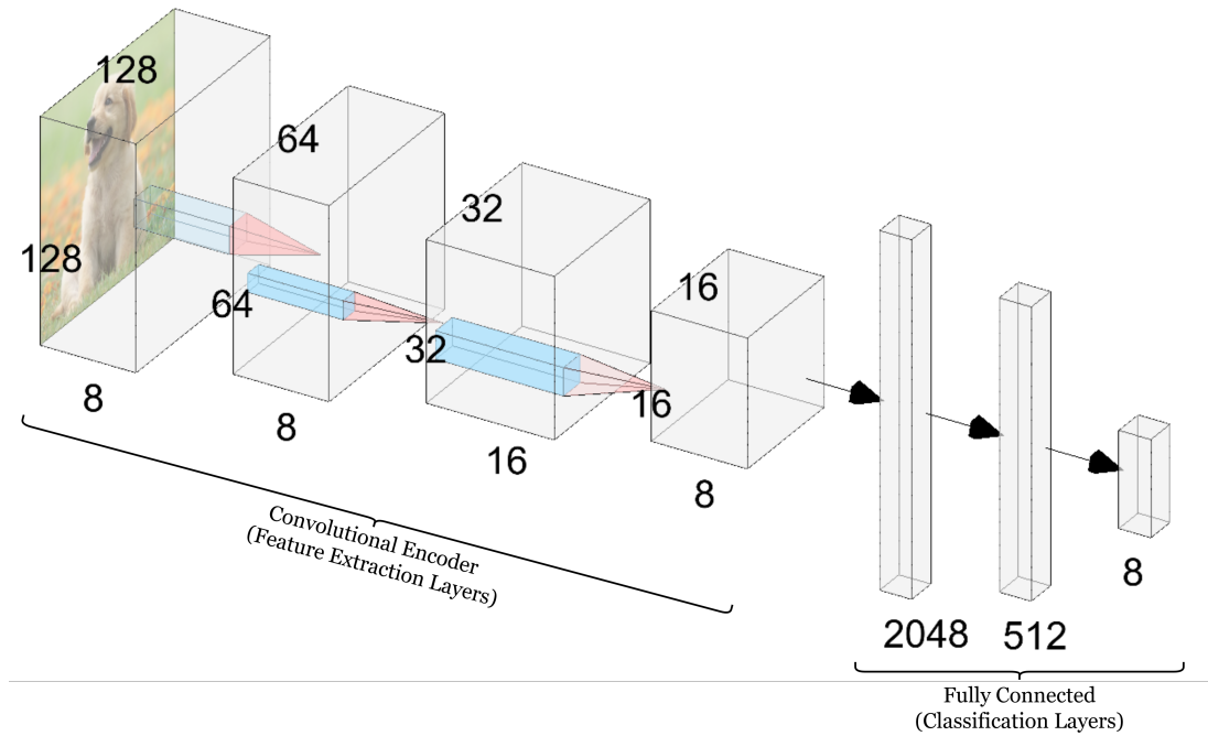
Figure 3.2: Illustration of a convolutional neural network (CNN) operating on an image input. As the network deepens, the spatial resolution is progressively reduced through convolutions and pooling before the resulting features are passed to a fully connected classifier.
