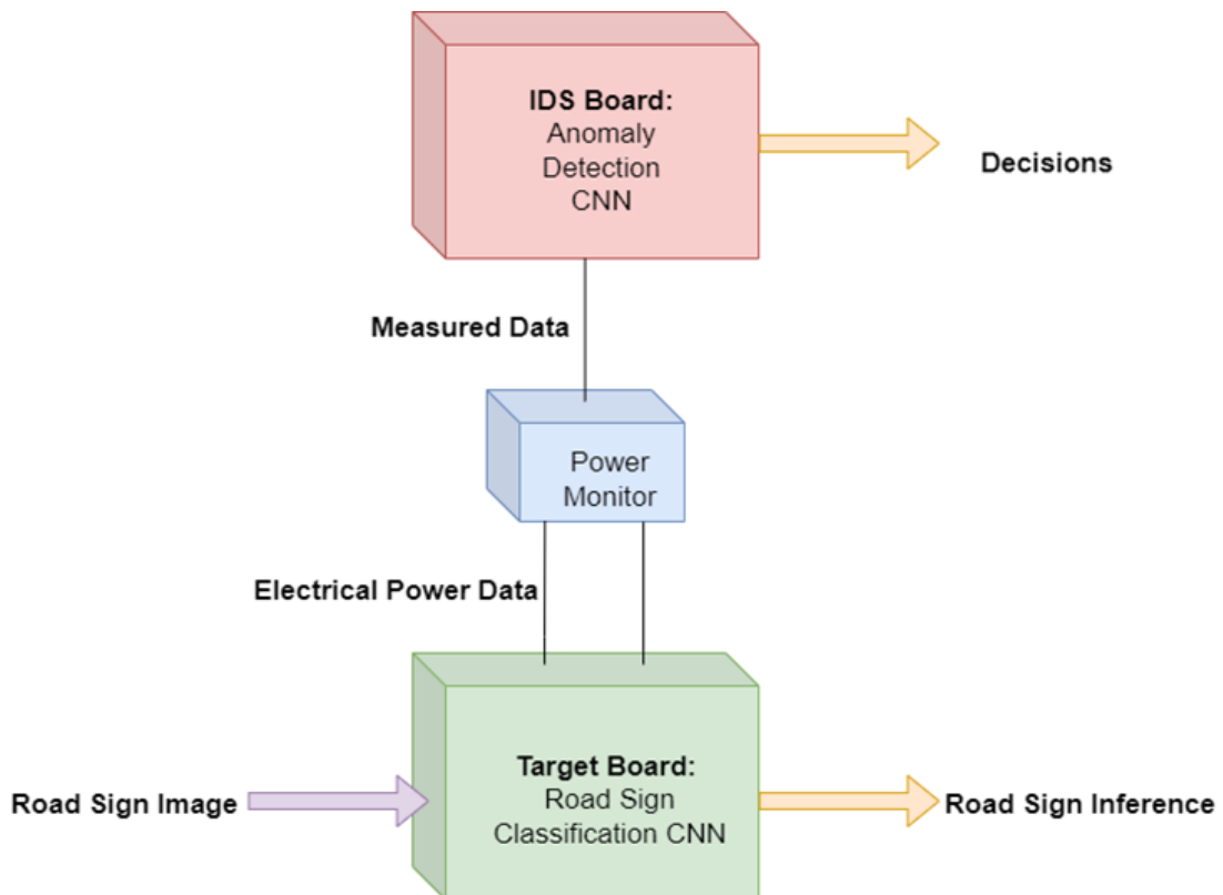
Figure 3.3: High-level framework showing the device to be protected and the IDS board monitoring its power usage.
