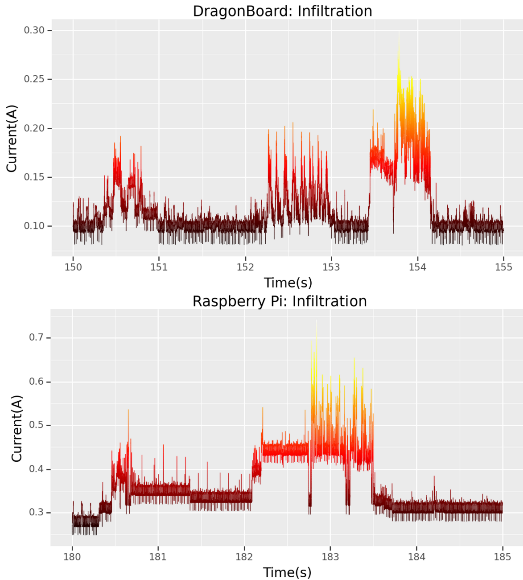
Figure 4.11: Infiltration during the CTF for the DragonBoard and Raspberry Pi (data visualised using the “hot” colormap [119]).
