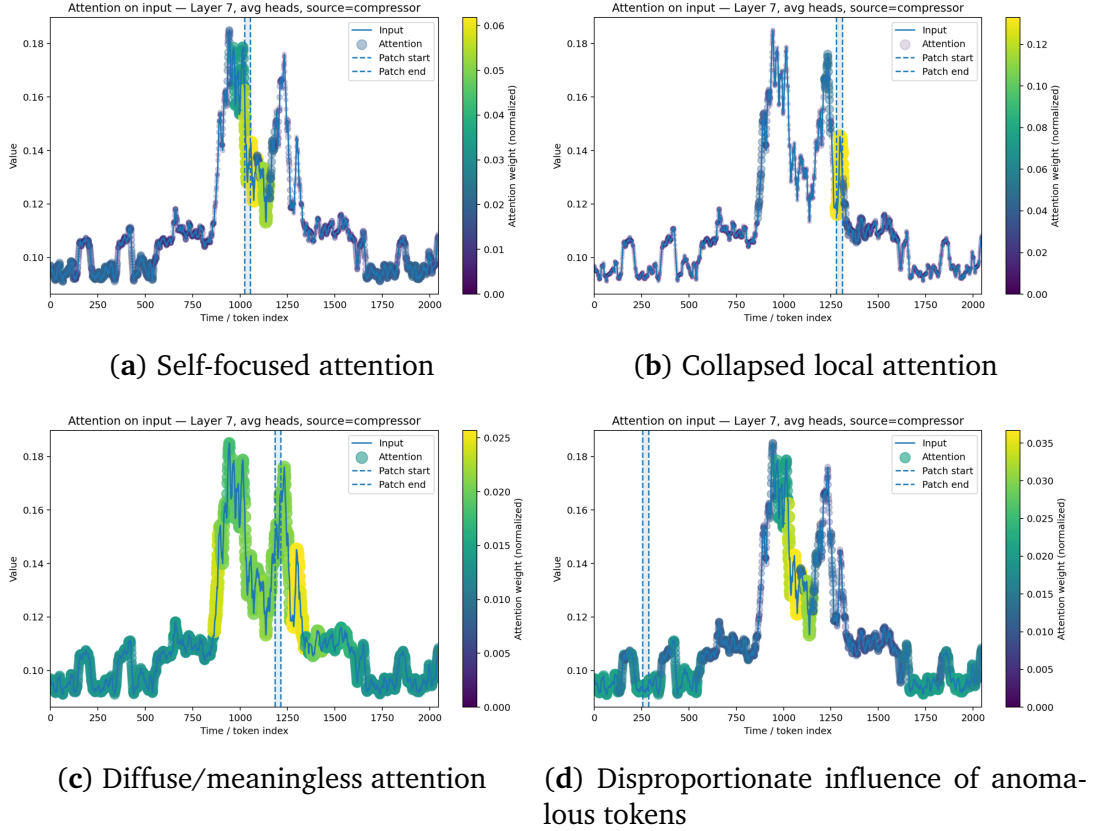
Figure 6.9: Examples of disrupted attention patterns under anomalous inputs within the compressed latent space (attention for a specific token).
