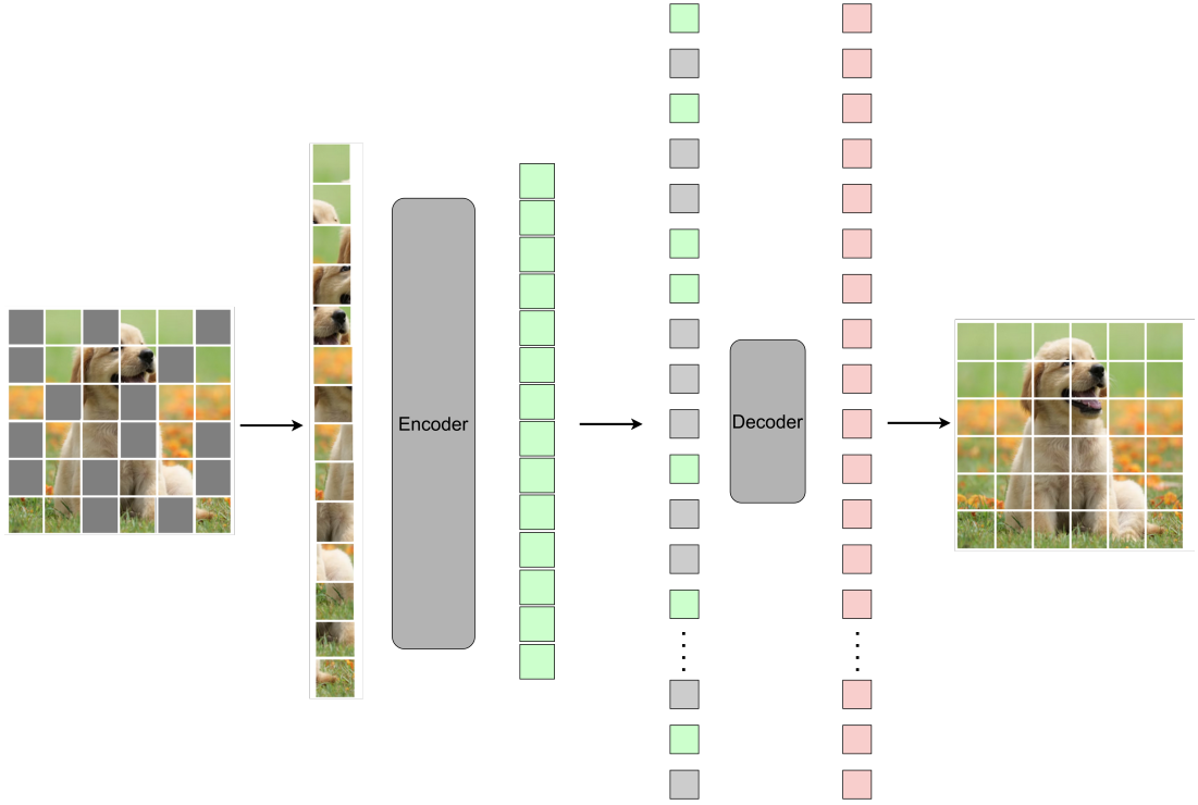
Figure 6.4: Illustration of an MAE with an asymmetric encoder-decoder design.
