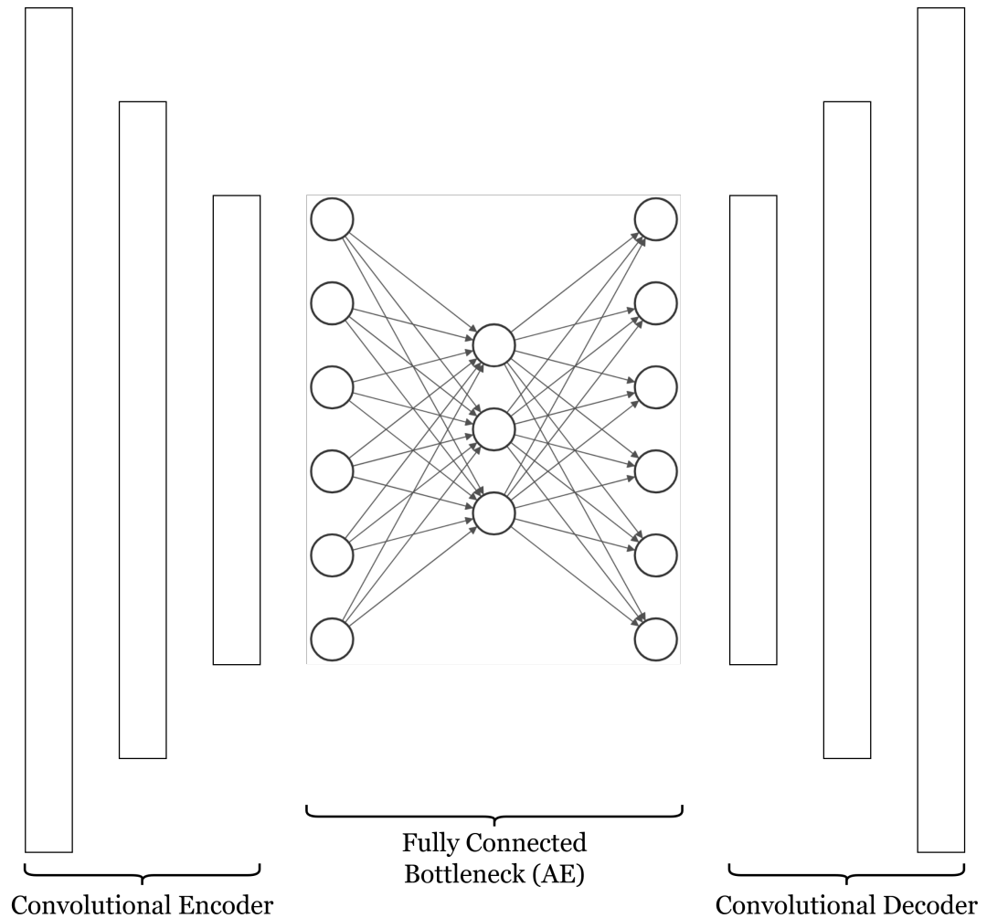
Figure 5.2: Convolutional autoencoder (CAE) with a convolutional encoder, a fully connected AE bottleneck, and a convolutional decoder.
