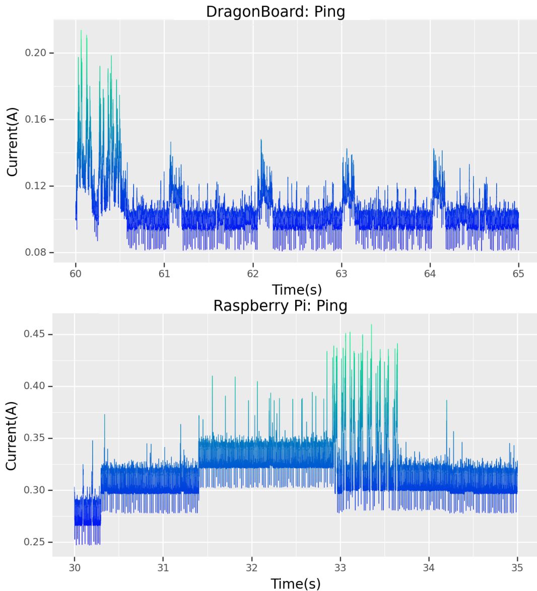
Figure 4.7: Comparison of ping behaviour for the DragonBoard and Raspberry Pi (data visualised using the “winter” colormap [119]).
