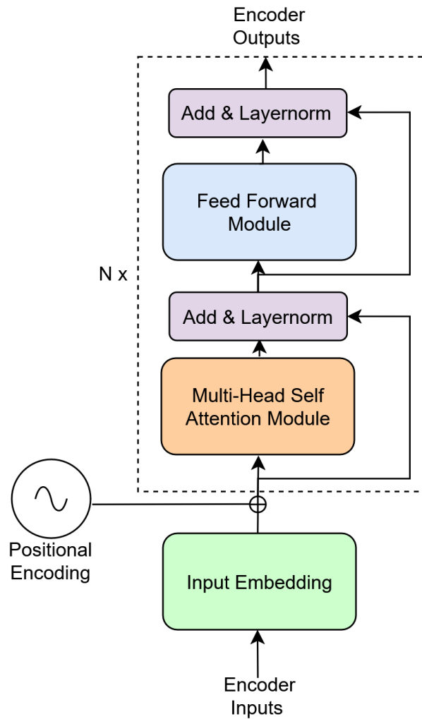
Figure 6.2: Overview of an encoder-only Transformer architecture composed of stacked self-attention and position-wise feed-forward layers.
