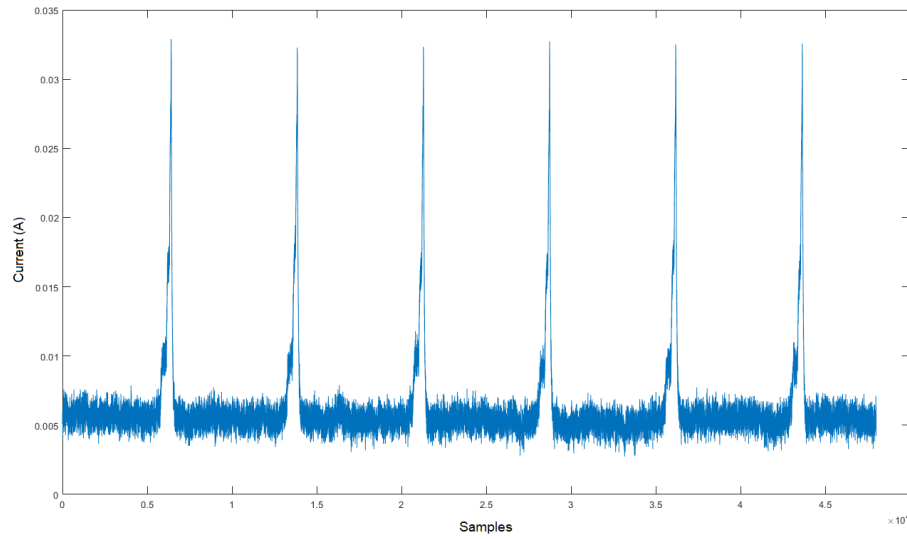
Figure 3.4: Normal power data sampled from the MAX78000 during six consecutive inferences of the road-sign classification model. Each peak corresponds to combined CPU and NPU activity.
