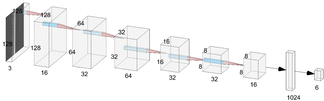
Figure 3.8: Kaggle Cats vs Dogs CNN architecture, supplied with the MAX78000.
