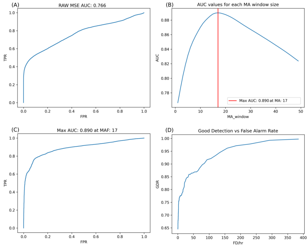
Figure 5.10: Performance of the dropout-based CAE (1024) model. (A) Raw MSE AUC; (B) AUC versus MAF window length; (C) ROC curve at optimal MAF length; and (D) GDR performance showing detection versus false-alarm rate.
