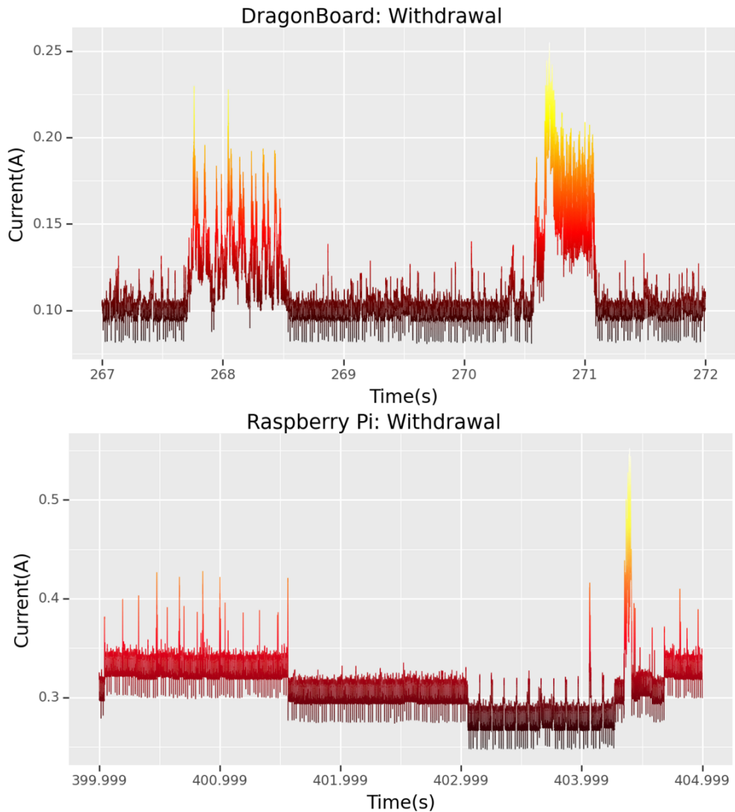
Figure 4.14: Withdrawal of the attacker following CTF completion for the DragonBoard and Raspberry Pi (data visualised using the “hot” colormap [119]).
