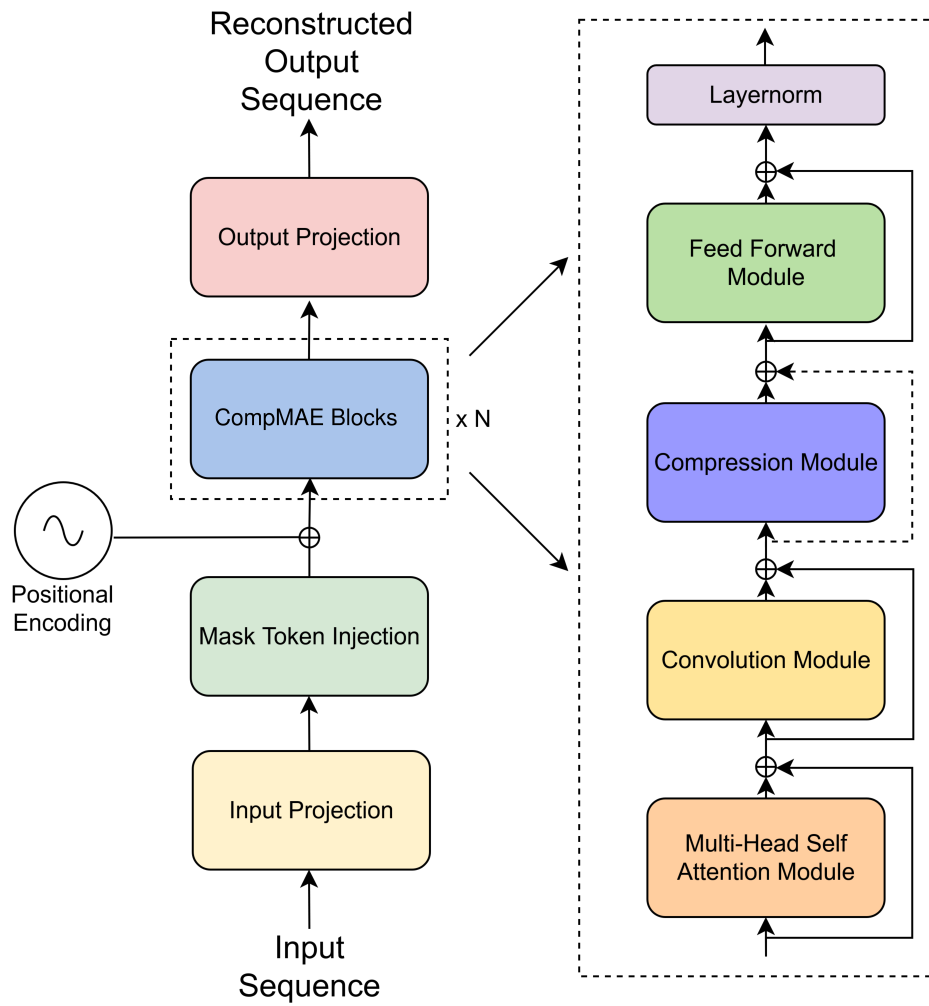
Figure 6.5: Overview of the COMPMAE encoder architecture.
