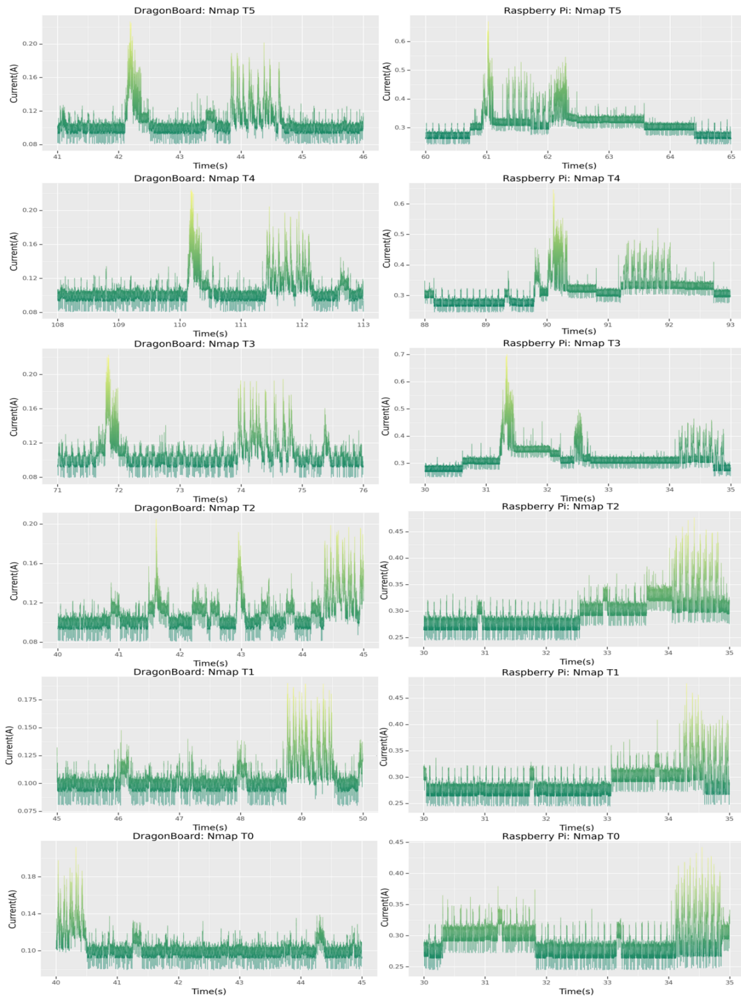
Figure 4.3: Each Nmap T-Switch behaviour for DragonBoard versus Raspberry Pi (data represented using the “summer” colormap [119]).
