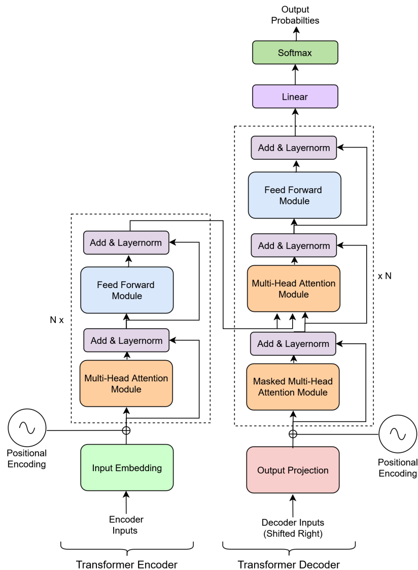
Figure 6.1: Overview of a standard encoder–decoder Transformer architecture as presented in [139]. A classification head attached to the decoder outputs can be used for tasks such as sentence classification.
