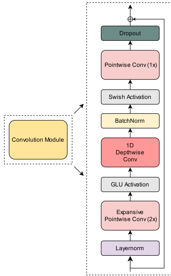
Figure 6.7: Conformer-style convolution module used in both CONFORMER-MAE and COMPMMAE.
