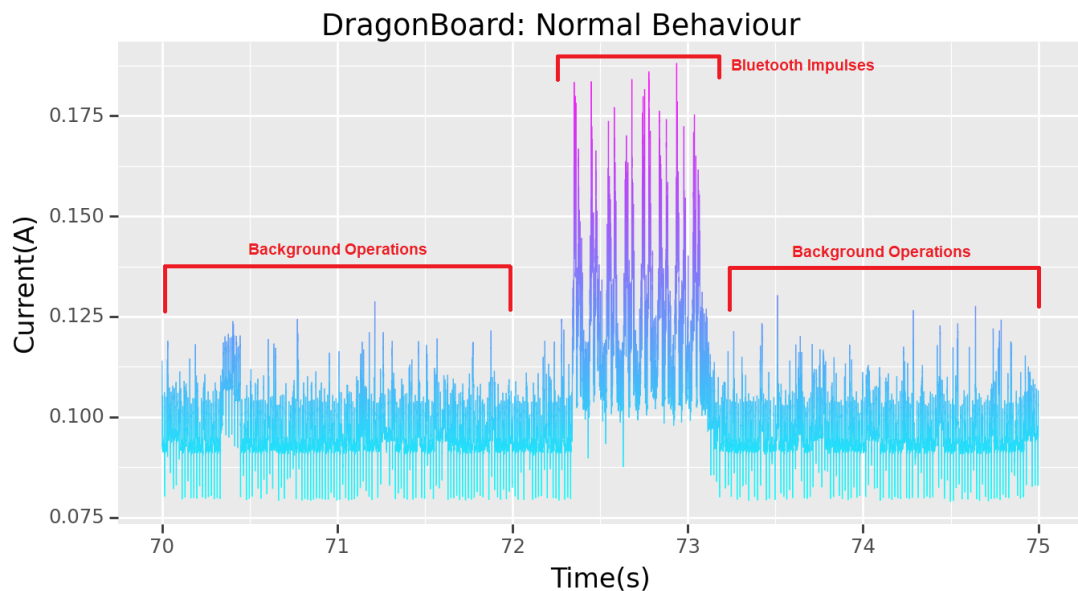
Figure 2.4: Example time series power segment of normal data. Specifically of a burst of Bluetooth communication on the DragonBoard 410c (seen around 72.1s to 73.1s).
