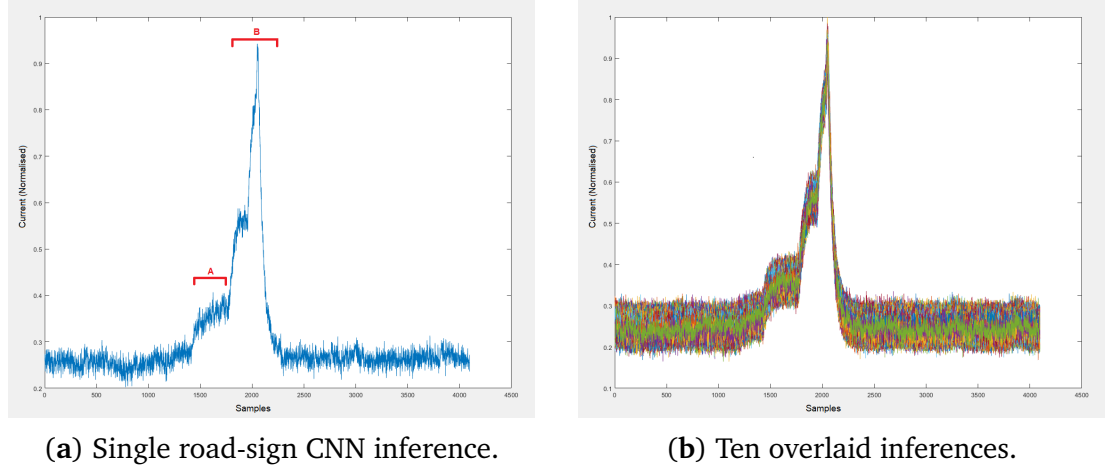
Figure 3.5: Road-sign CNN inference power traces. (Left) Single inference showing CPU loading (A) and NPU spike (B). (Right) Ten overlaid inferences demonstrating high repeatability.
