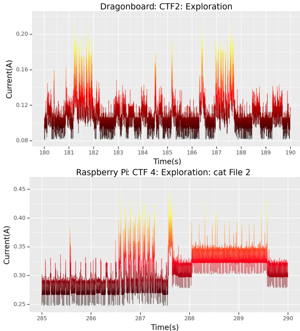
Figure 4.12: Comparison of attacker exploration activity on the DragonBoard and Raspberry Pi (data visualised using the “hot” colormap [119]).
