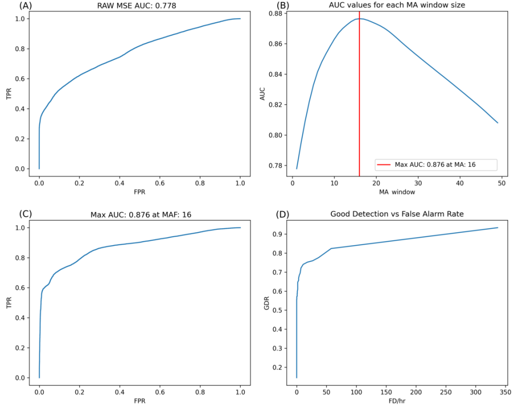
Figure 5.5: Performance of the CAE (1024) model: (A) raw AUC without smoothing; (B) AUC versus MAF window length; (C) ROC curve at optimal MAF 16; and (D) event-based anomaly detection rate (GDR) versus false alarms per hour.
