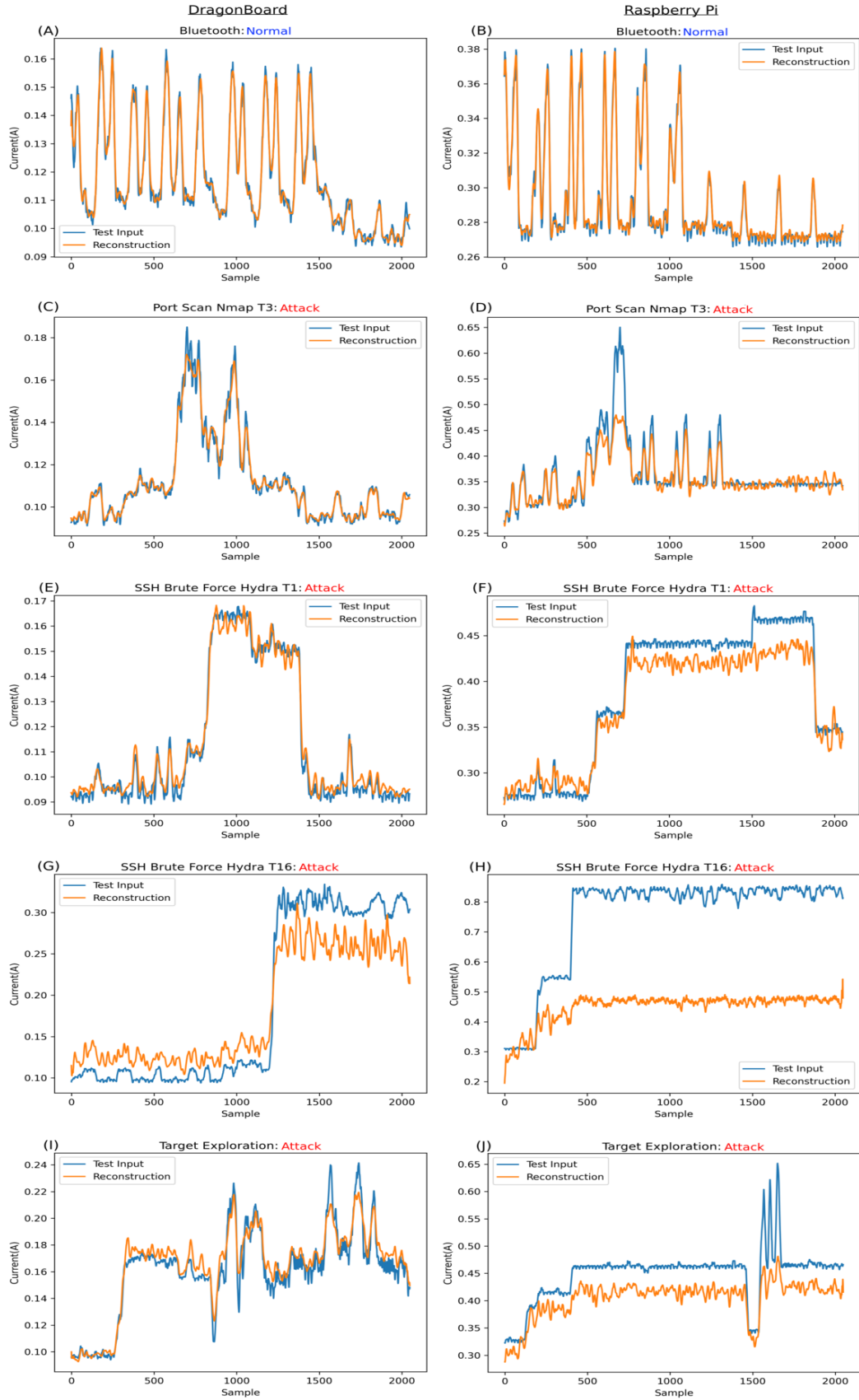
Figure 5.7: Reconstructions using the CAE (1024) model (DragonBoard (left) vs. Raspberry Pi (right)). (A,B) normal behaviour; (C,D) Nmap_T3 anomalies; (E,F) Hydra_T1 anomalies; (G,H) Hydra_T16 anomalies; (I,J) infiltration traces.
