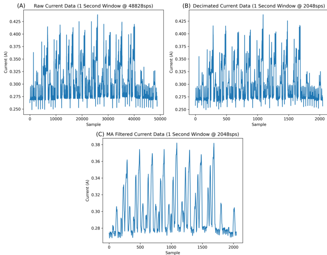
Figure 5.3: Preprocessing pipeline: (A) raw data at 48,828 Hz, (B) resampled data at 2,048 Hz, and (C) MAF-filtered data at 2,048 Hz with MAF size 15.
