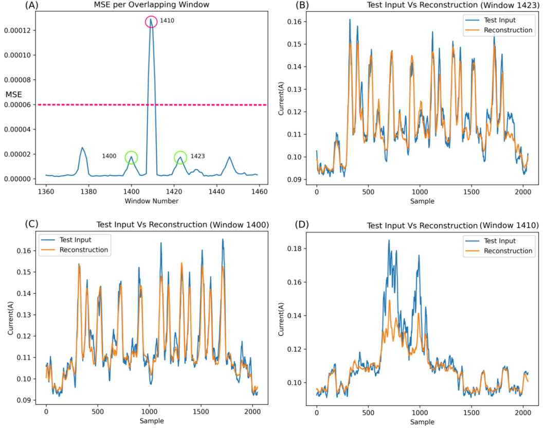
Figure 5.12: MSE analysis of the dropout-based CAE (1024) model. (A) Overall MSE sequence; (B,C) Bluetooth behaviour segments; and (D) Nmap_T3 anomaly. The dropout model produces a distinct separation between normal and anomalous error magnitudes, enhancing robustness.
