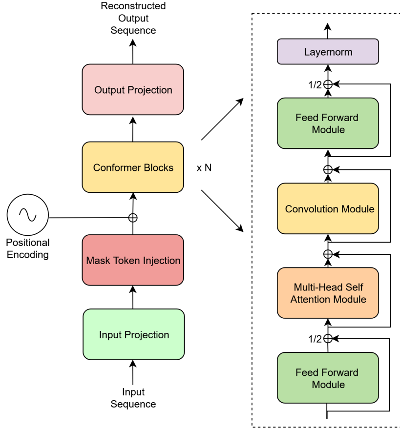
Figure 6.3: Diagram of a standard Conformer block combining macaron-style FFNs, MHSA, and a convolutional module within a residual and LayerNorm framework.
