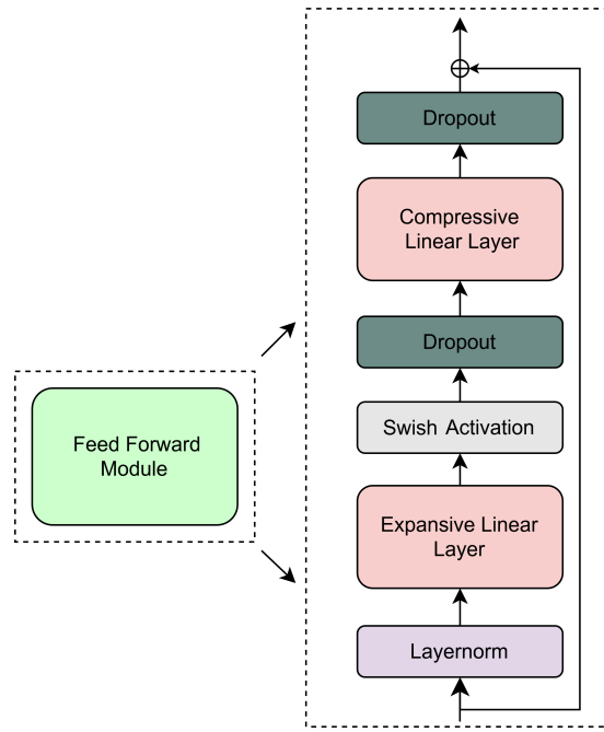
Figure 6.10: Feed-forward module used in COMPMAE, comprising a linear expansion, Swish (SiLU) activation, dropout, and linear compression.
