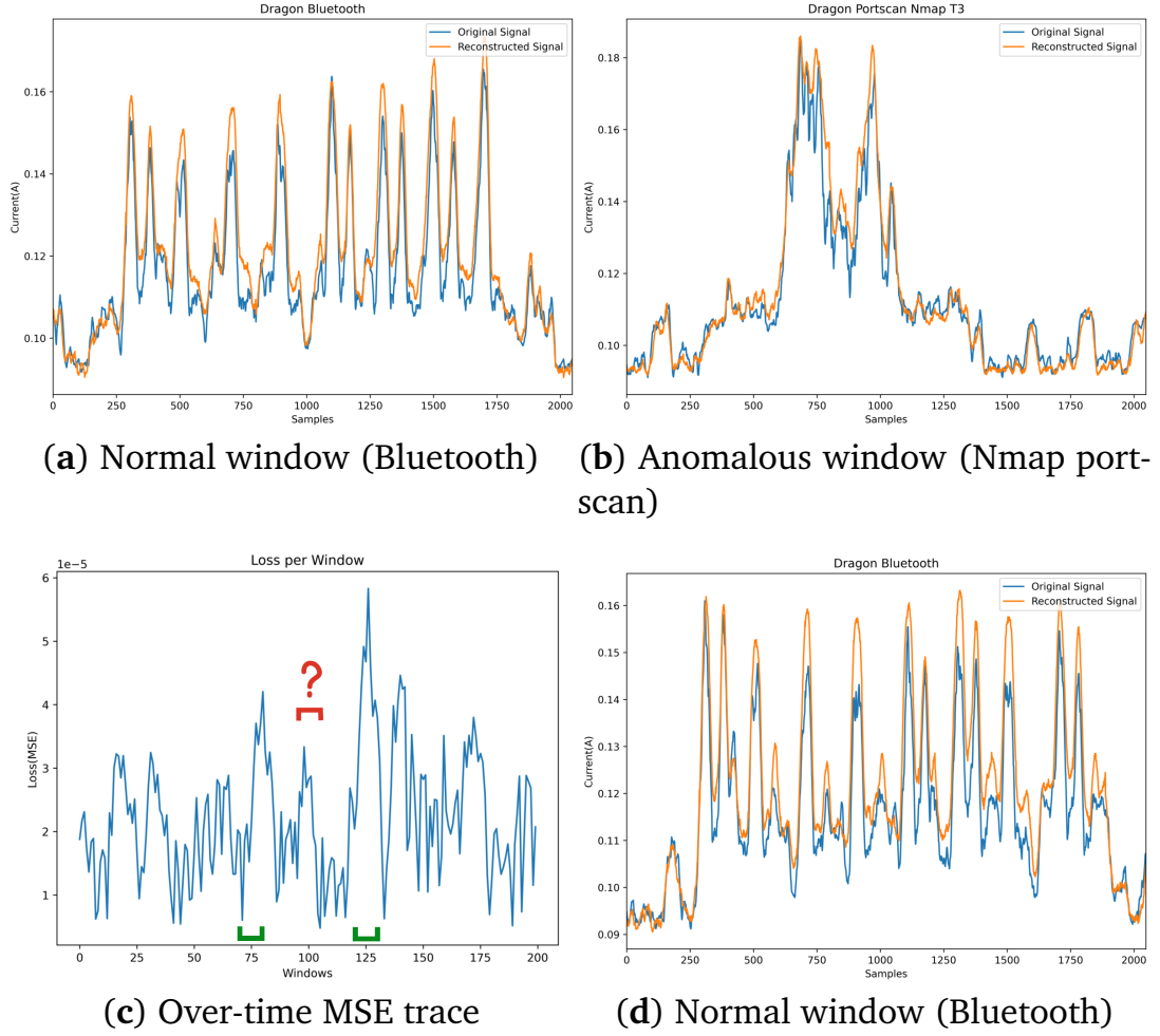
Figure 6.16: Reconstruction behaviour of the CONFORMER-MAE baseline over 200 windows. Normal windows are reconstructed accurately, but the Nmap port-scan anomaly is also reproduced with high fidelity, yielding an MSE trace in which the anomalous response is almost indistinguishable from normal operation (the anomaly lies within the region marked in red, while normal Bluetooth activity appears in the regions highlighted in green).
