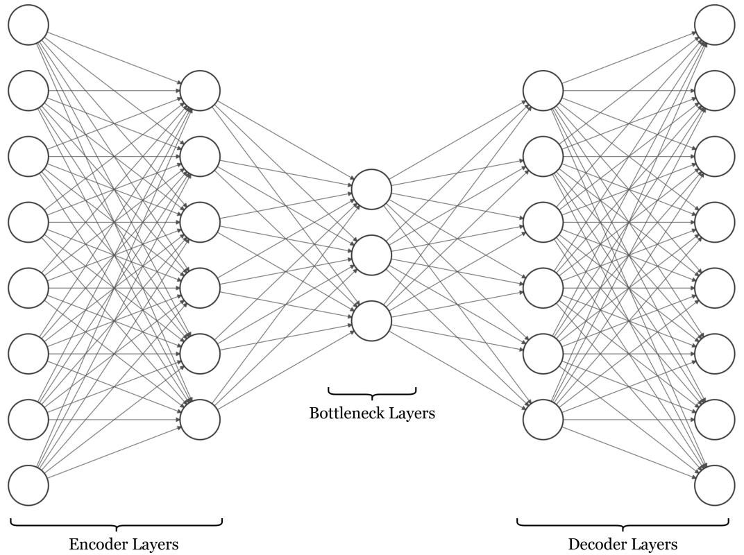
Figure 5.1: Simple AE architecture comprising an encoder, a low-dimensional bottleneck (latent representation), and a decoder. Note the compression of the latent space.
