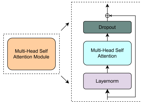
Figure 6.6: Schematic of MHA within a COMPMAE block. Each head models contextual dependencies across masked and unmasked tokens before convolutional refinement.
