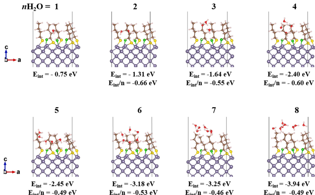
Fig. 12. Calculated adsorption energies and optimized structures of Ge(100) with 62.5% butanethiol coverage, with n (1, ..., 8) water molecules.
