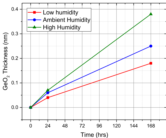
Fig. 5. GeO 2 thicknesses of HT-passivated Ge exposed to low, ambient, and high RH for 0, 24 and 168 h.
