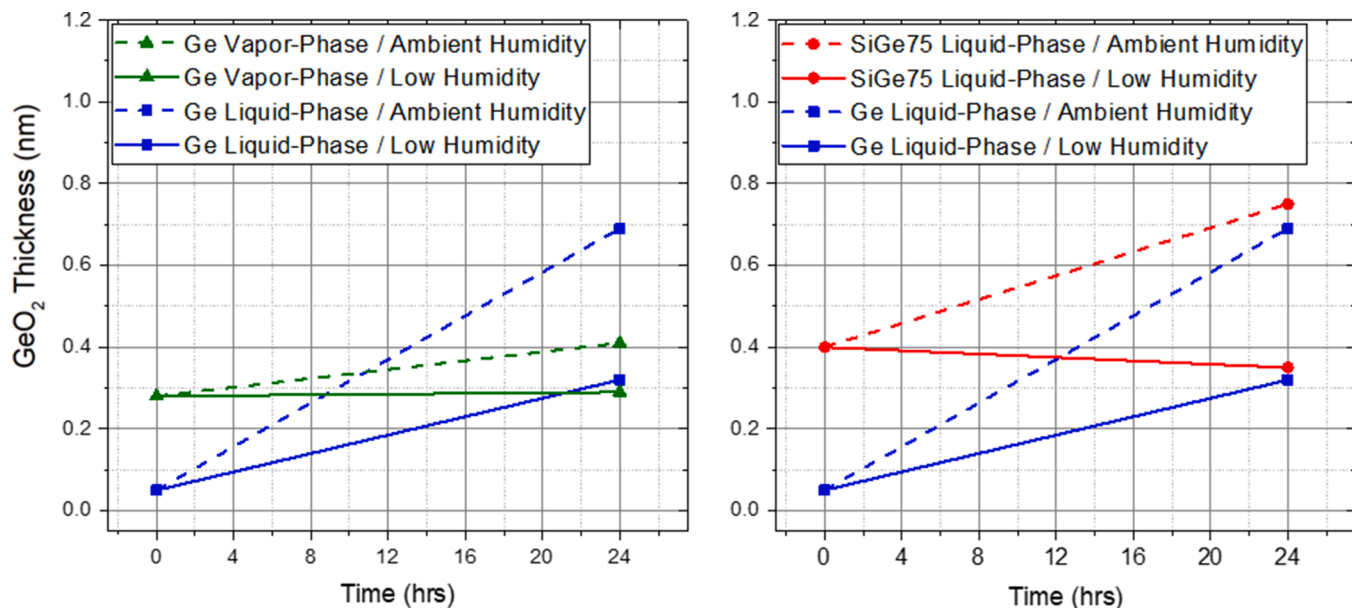
Fig. 8. GeO 2 thicknesses of (left) Ge samples passivated by vapor-phase deposited OT and solution-phase deposited DDT and (right) DDT-passivated SiGe75 exposed to low and ambient RH for 0 and 24 h. Values extracted from Ge 2p spectra.
