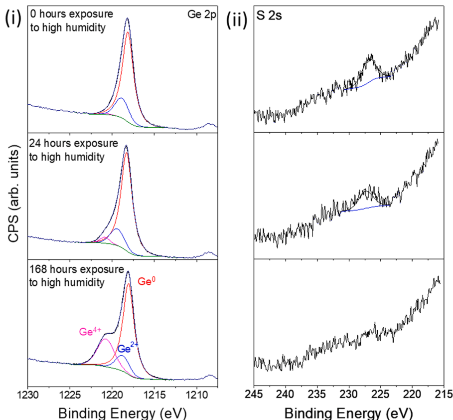
Fig. 2. (i) Ge 2p and (ii) S 2s spectra for HT-passivated Ge showing increasing in intensity of GeO 2 peak and decrease in intensity of sulfur peak for the sample exposed to 90% RH over 168 h.
