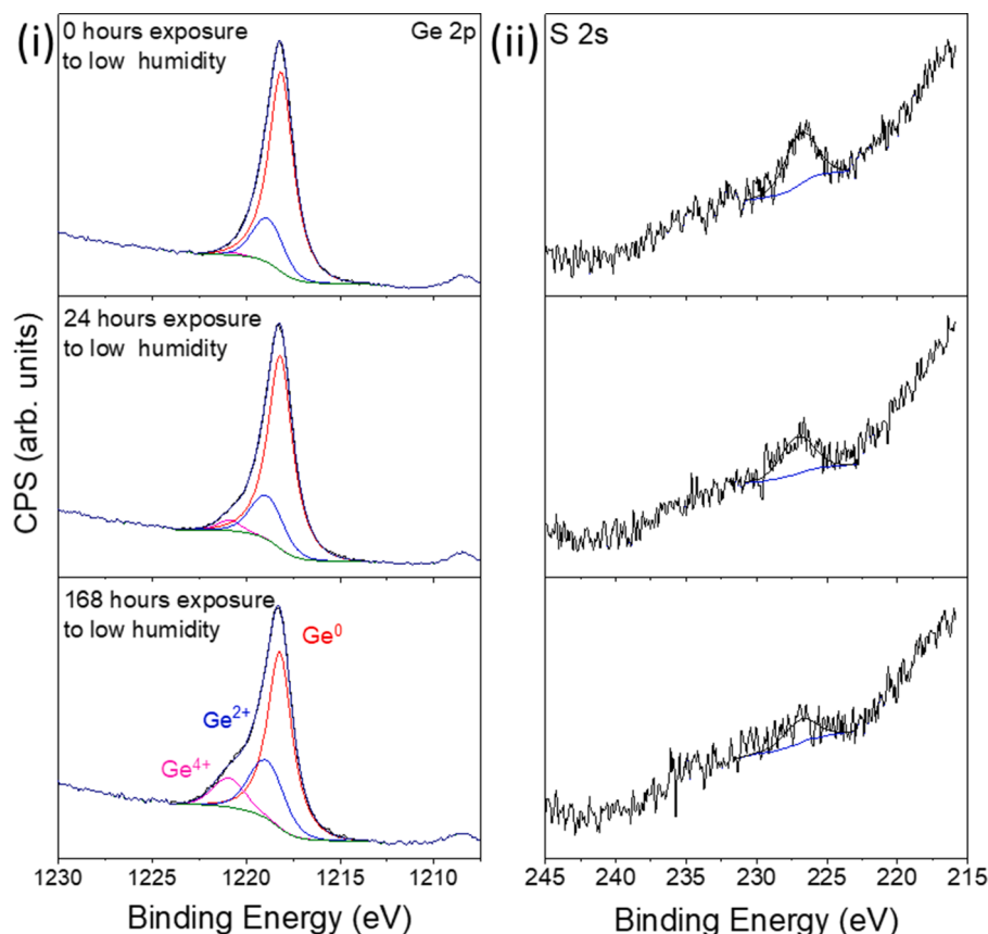
Fig. 4. (i) Ge 2p and (ii) S 2s spectra for HT-passivated Ge showing increase in intensity of GeO 2 peak and decrease in intensity of sulfur peak for sample exposed to 5% RH over 168 h.
