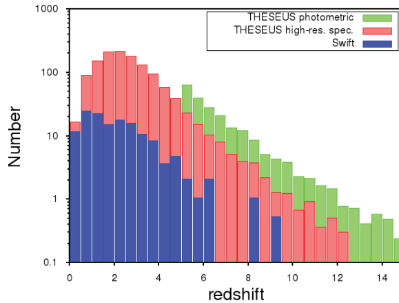
Figure 19: The redshift distribution of THESEUS GRBs during a 5 yr mission lifetime compared to the actual distribution of Swift GRBs (blue) during the same period. GRBs with a photometric redshift are in green, and those with a spectroscopic redshift are in red.
