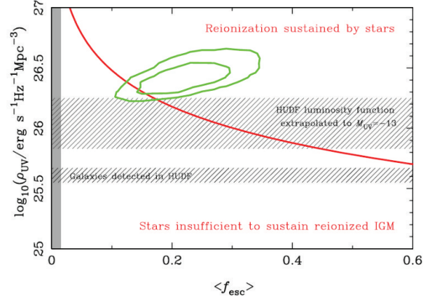
Figure 8: The UV luminosity density from stars at z \approx 8 and average escape fraction ( \langle f_{\text{esc}} \rangle ) are insufficient to sustain reionization unless the galaxy luminosity function steepens to magnitudes fainter than M_{\text{UV}} = -13 (grey hatched region), and/or \langle f_{\text{esc}} \rangle is much higher than that typically found at z \approx 3 (grey shaded region). Even in the late 2020s, \langle f_{\text{esc}} \rangle at these redshifts will be largely unconstrained by direct observations. The green contours show the 1 and 2- \sigma expectations for a sample of 25 GRBs at z \approx 7-9 for which deep spectroscopy provides the host neutral column and deep imaging constrains the fraction of star formation occurring in hosts below the JWST limit (Robertson et al., 2013). The input parameters were \log_{10}(\rho_{\text{UV}}) = 26.44 and \langle f_{\text{esc}} \rangle = 0.23 , close to the (red) borderline for maintaining reionization by stars.
