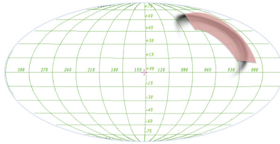
Figure 10: The plot shows the SXI field of view ( \sim 110 \times 30 deg 2 ) superimposed on a simulated probability skymap of a merger NS-NS system observed by aLIGO and advanced Virgo (Singer et al., 2016). The SXI coverage contains nearly 100% of the total probability.
