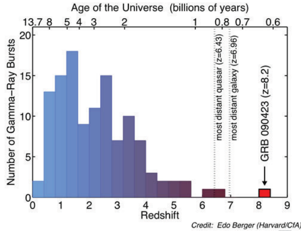
Figure 6: Redshift distribution of GRBs (credits Berger, Harvard/CfA).
