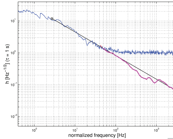
Figure 18: Broadband spectrum obtained as an average of 42 relatively bright bursts from the BeppoSAX catalog through butterfly filtering (purple curve) using a bank of 8.64 million chirp templates. The broadband Kolmogorov spectrum extends standard Fourier-based spectra (blue curve) up to a few kHz in the comoving frame. The absence of any high frequency bump favors inner engines harboring black holes rather than magnetars (from van Putten et al., 2014).
