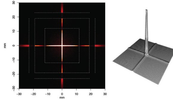
Figure 29: The point spread function of the SXI.
