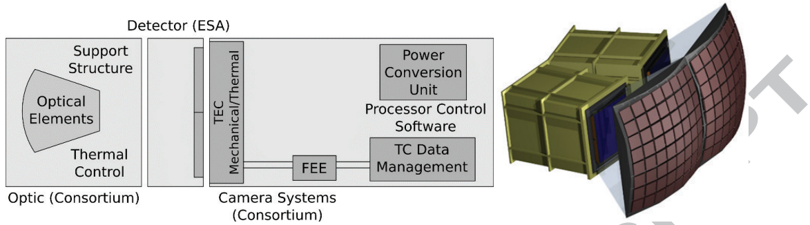
Figure 27: The SXI block diagram concept (left) and optical elements (right).
