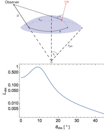
Figure 11: Top panel: possible geometry of the conical jet, in spherical coordinates with the origin at O. The observer is located at (D, \Theta_{\text{obs}}, 0) . The jet is moving with Lorentz factor \Gamma(\Theta) . Bottom panel: Luminosity fraction (normalized to peak emission) as a function of observer angle, L_{\text{obs}}(\Theta_{\text{obs}}) , from Kathirgamaraju et al. (2017). The jet luminosity at \sim 40 deg is a factor of 300 fainter than that of the jet core. Nevertheless, such a misaligned jet can be detected by a \gamma -ray instrument if it takes place within the Advanced LIGO detectability volume.
