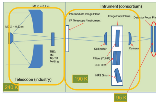
Figure 38: The IRT Telescope block diagram concept.
