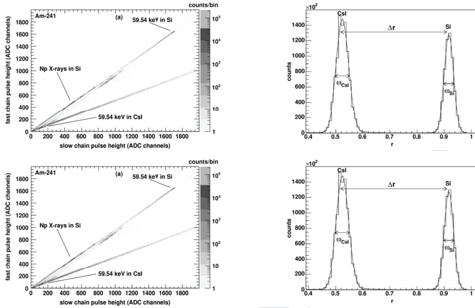
Figure 34: Left : bidimensional spectrum of a ^{241}\text{Am} source showing interaction in Silicon (top line) and in the scintillator (bottom line). Right : distribution of the ratio of the two processing chains for events in Silicon and in the scintillator. The large peak separation indicates the optimal discrimination performance.
