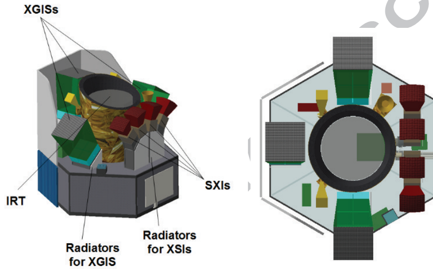
Figure 42: THESEUS Satellite Baseline Configuration and Instrument suite accommodation.
