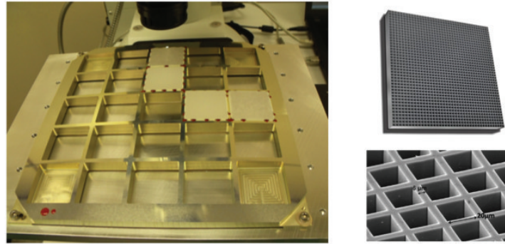
Figure 28: Left: The SVOM MXT lobster eye optic aperture frame. Top right: A schematic of a single square pore MCP. Bottom right: A micrograph of a square pore MCP showing the pore structure. This plate has a pore size d=20\ \mu\text{m} and a wall thickness w=6\ \mu\text{m} .
