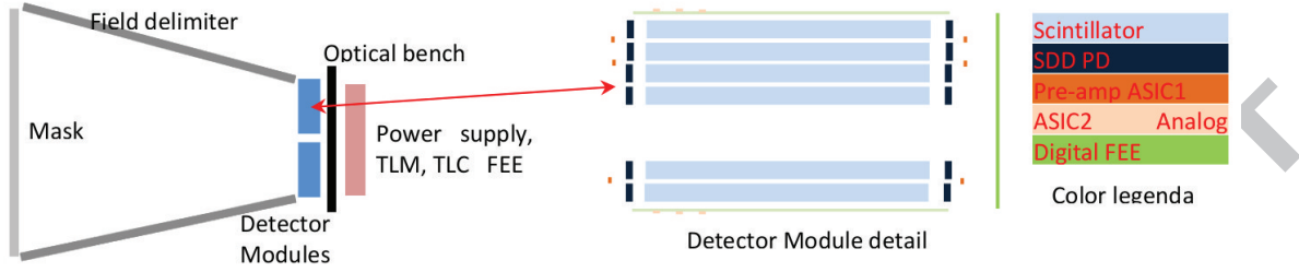
Figure 35: XGIS unit main building blocks.
