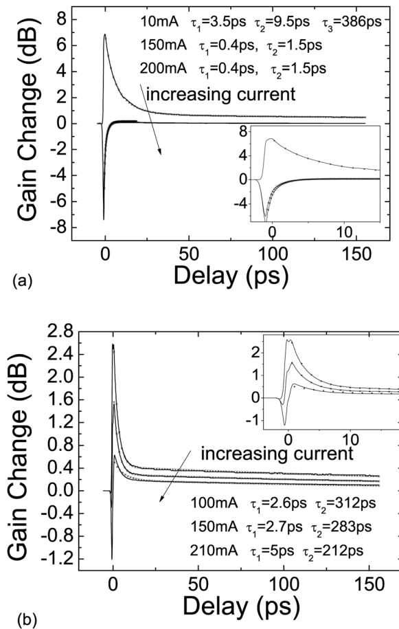
FIG. 2. Gain dynamics at GS (a) and ES (b) wavelengths with corresponding multiexponential fits and timescales. A zoom of the dynamics over the first 15 ps is shown in inset. GS injection levels were 10 mA, 80 mA, 150 mA, and 200 mA with transparency at \sim 70 mA (150, 200 mA overlapping). ES injection levels were 100 mA, 150 mA, and 210 mA.
