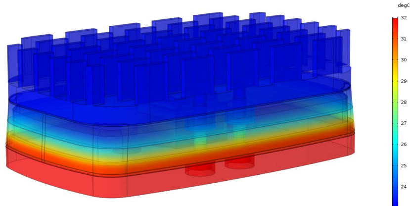
Figure 11 — Thermal Modelling of a Wireless Sensor Housing with Thermoelectric Power Supply ( 6.5 \times 4 \times 2.5 \text{ mm}^3 )
