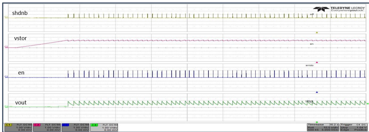
Figure 20 — System Signals
