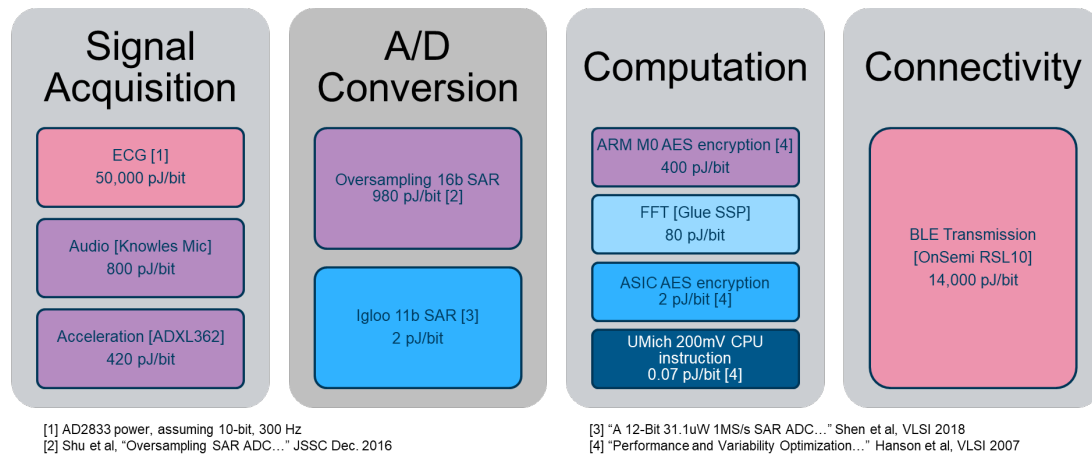
Figure 21 — Estimated Energy Consumed by Various IoT Sensor Functions (Blue = Low Energy; Red = High Energy)
