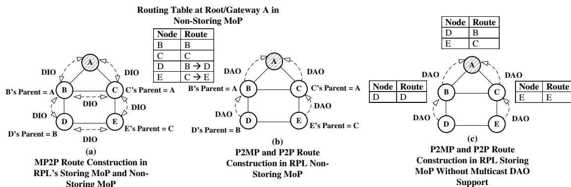
Figure 1. Routing Protocol for Low-Power and Lossy Networks (RPL) Operation with Storing and Non-Storing Modes of Operation (MoPs).
