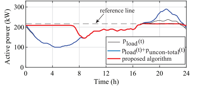
Fig. 11. Aggregated load profile with forecasting errors in number of PEVs and user choices.
