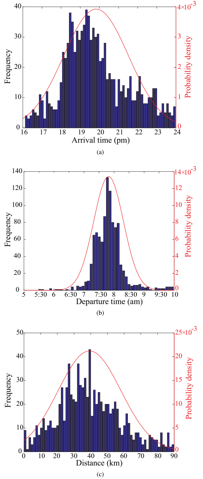
Fig. 2. Histogram of the collected data (bar) and corresponding Gaussian distribution fit (line) for (a) arrival time, (b) departure time, and (c) daily trip distances.
