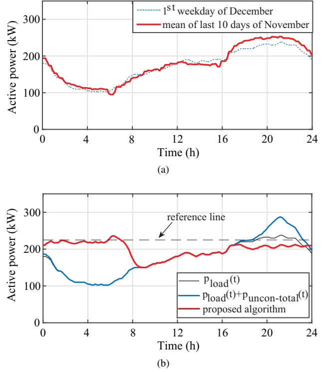
Fig. 10. Behavior of the algorithm in response to load forecasting error: (a) forecasted load and actual load profiles (b) load leveling performance.
