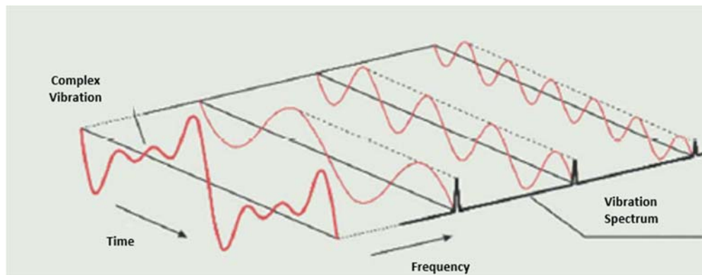
Figure 17 FFT processing of a complex vibration signal [81]
