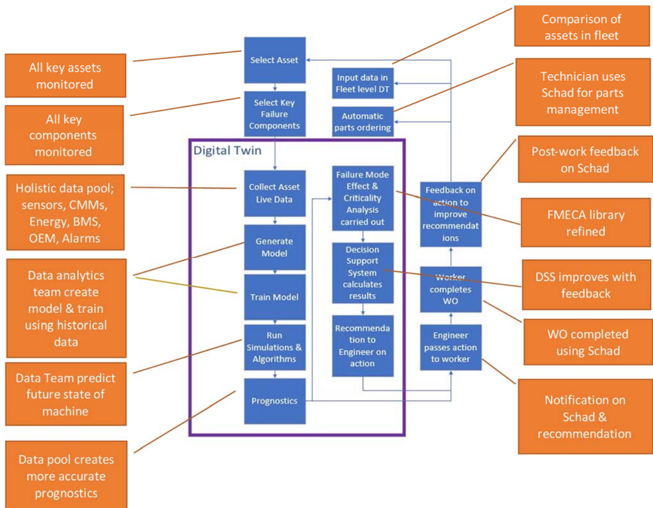
Figure 25 Digital Twin Framework Version 3
