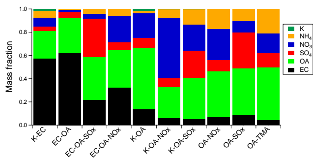
Fig. 6. Mass fractions of each chemical species determined for each ATOFMS class.
