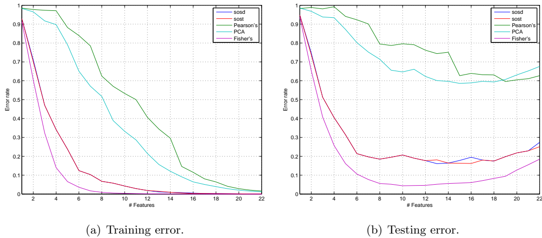
Figure 3.6: Effect of feature selection.
