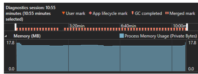
Figure 6. Memory profile for BMS archive ingestion
