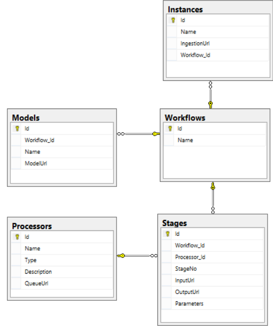
Figure 8. Database schema for workflow management
