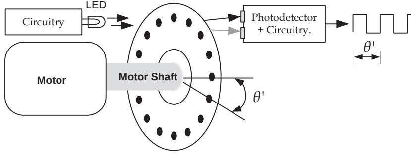
Figure 2.1 Minimum rotated angle.
