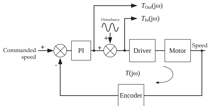
Figure 5.3 Open-loop measurement T(j\omega) of the speed control loop.
