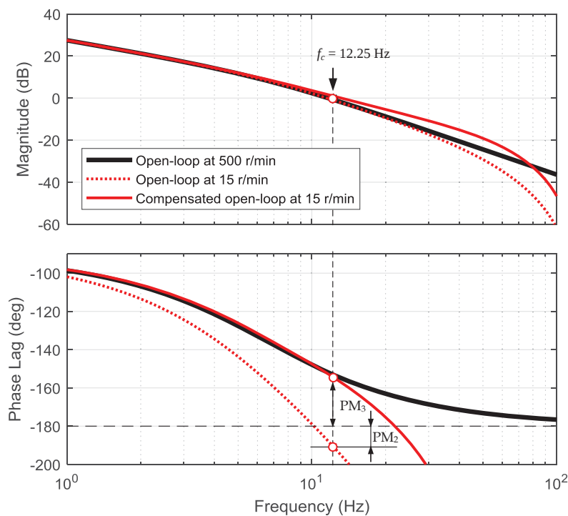
Figure 5.22 Bode plot of the open-loop compensated system.
