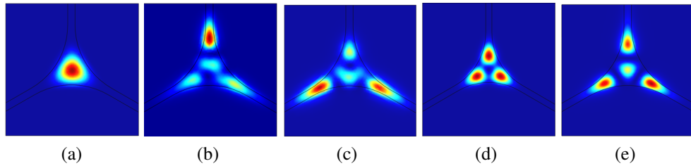
Figure 8.3: Field patterns for the suspended-core optical fibre
