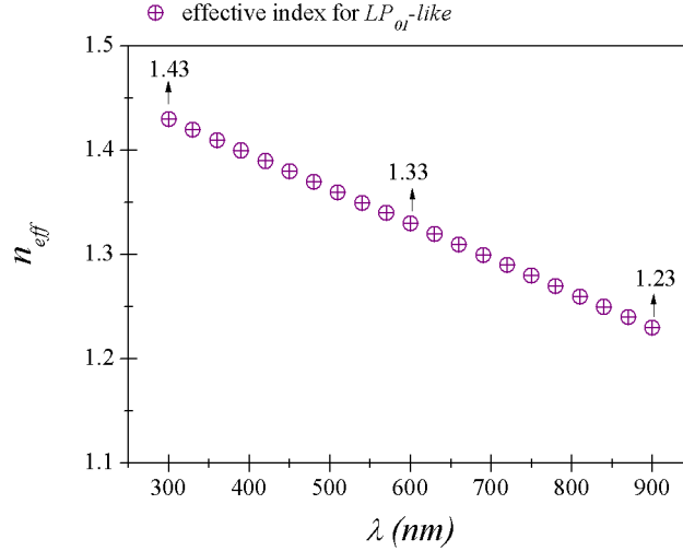
Figure 3.9: Graph of the effective index for the wavelength as a function of wavelengths (purple crossed circles)
