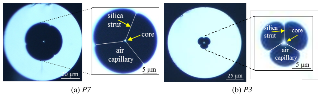
Figure 8.1: The suspended-core optical fibres with zoomed-in section of the microstructure cladding, where (a) is P7 and (b) is P3
