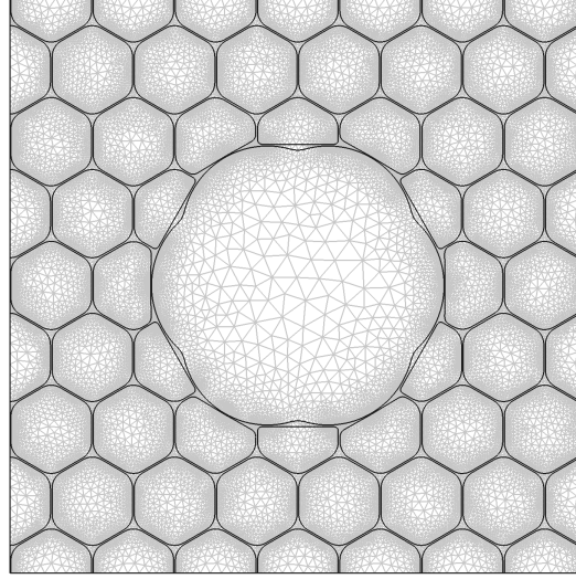
Figure 3.3: Applied mesh of the fibre structure
