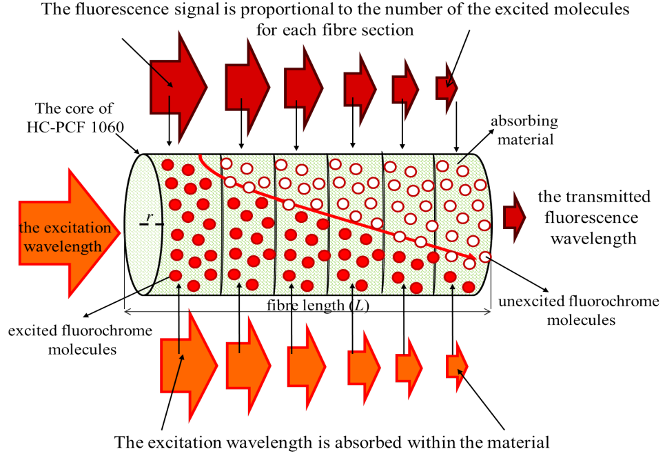
Figure 6.12: Schematic of fluorescence transmitted intensity for HC-PCF filled with an absorbing material with fluorochrome molecules
