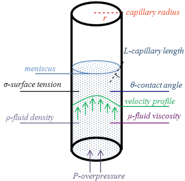
Figure 2.9: Fluid parameters in a capillary cross section
