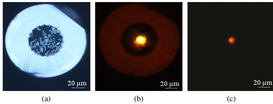
Figure 6.4: Examples of the fibre filled with the hydrogel and (b) near-field images with supercontinuum propagation in the core with a neutral density filter OD 2.0 and (c) OD 3.0
