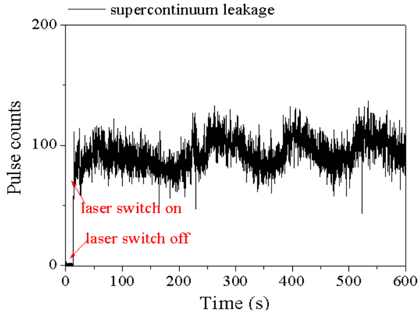
Figure 7.11: Graph of peak counts for a leaked supercontinuum signal (black line)
