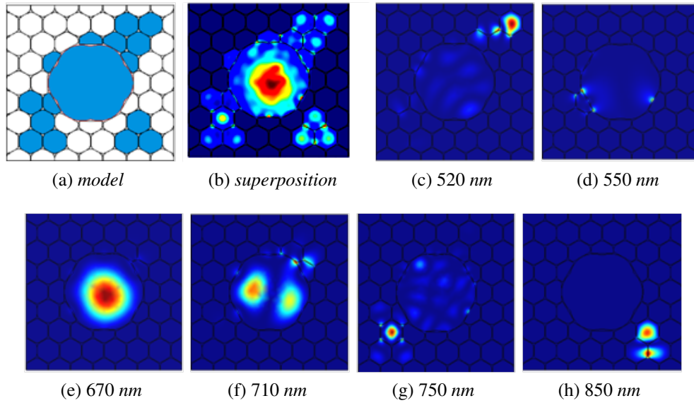
Figure 6.9: (a) refractive index mapping for Comsol simulations, with shaded blue fillings ( n=1.33 ) and white empty holes ( n=1.00 ), (b) Matlab superposition of all simulated frames in the range of 520 \text{ nm} \leq \lambda \leq 870 \text{ nm} ; light observed at: (c) 520 nm , (d) 550 nm , (e) 670 nm , (f) 710 nm , (g) 750 nm , (h) 850 nm
