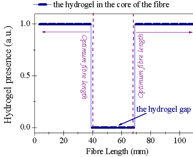
Figure 5.18: Graph of the hydrogel distribution in the fibre core achieved with the side view scanning method
