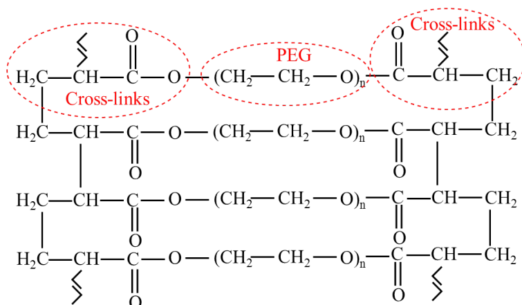
Figure 2.23: Idealised representation of PEGDA network [111]
