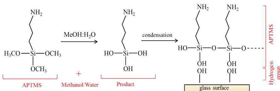
Figure 2.16: The attaching process of the silanising agent APTMS to a glass surface (part 1)
