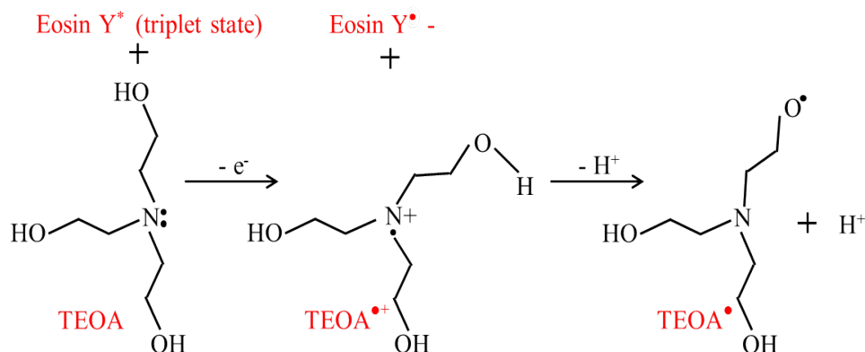
Figure 2.25: Scheme of proton loss from TEOA^{\bullet+} to neutral radical TEOA^{\bullet} , that allows polymerisation
