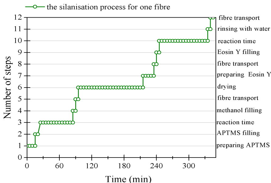
Figure 5.6: Graph of the silanisation process for one fibre as a function of time (min) with twelve described steps; the green circle symbol shows the time period for each step
