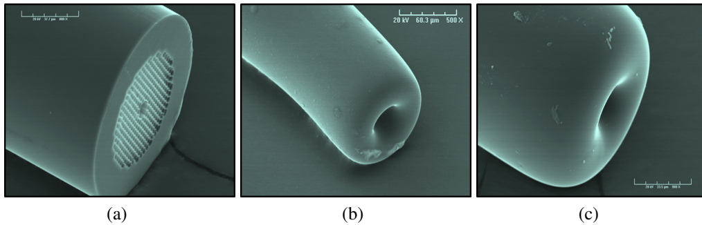
Figure 4.2: SEM images of the tip of HC-PCF 1550 fibre, where (a) shows an example before collapsing, (b) an example of the fibre after collapsing, and (c) the same fibre output after collapsing with higher magnification
