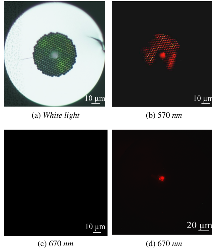
Figure 7.3: The images of the fibre cross-section, with hydrogel grown in the core, for (a) the optical microscope, and (b,c,d) fluorescence microscope with the integration times: (b) 2 ms, (c) 10 s (the hydrogel without the Cy-5 DNA probe), and (d) 1 s (the hydrogel with the Cy-5 DNA probe) [195]
