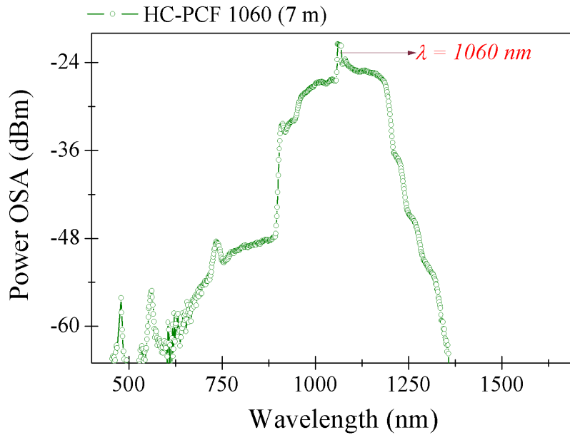
Figure 3.18: The transmitted spectrum for HC-PCF 1060 with a resolution 5 nm for the fibre length of 7 m
