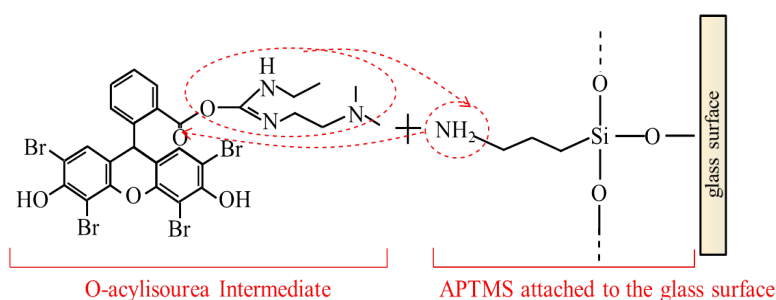
Figure 2.20: Scheme of bonding O-acylisourea intermediate and amine group of APTMS
