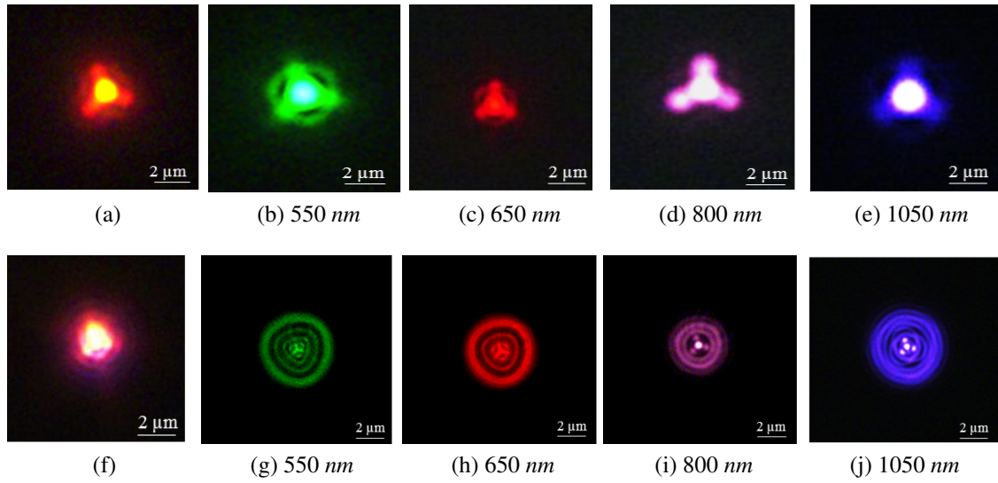
Figure 8.7: Near-field images for supercontinuum propagation for the P7 (upper row) and P3 (lower row) suspended-core fibres
