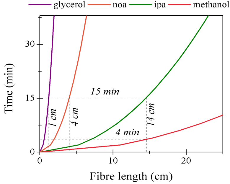
Figure 2.12: Graph of simulated time of filling the core with different liquids: pink line is for methanol, green line is for IPA, orange line is for NOA 73, and purple line is for glycerol
