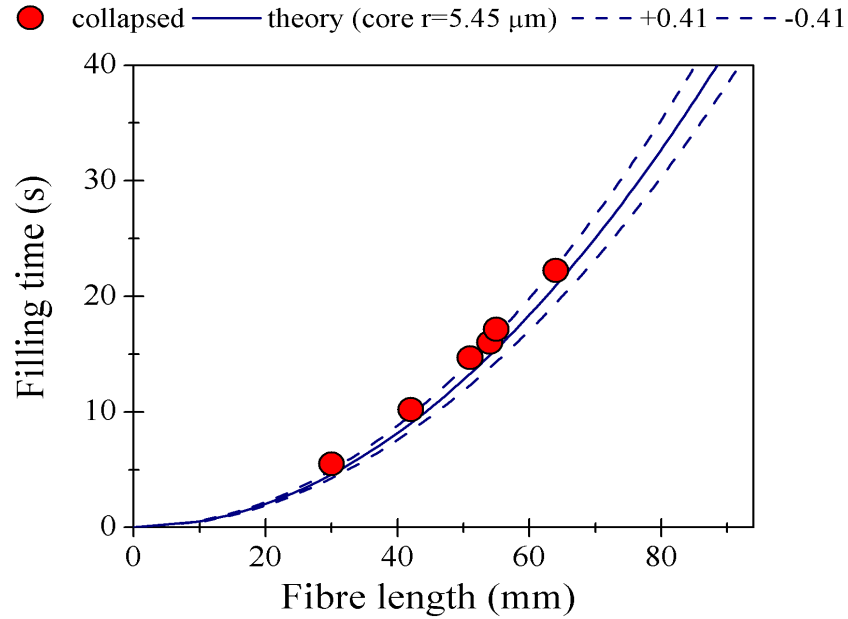
Figure 4.11: Graph of comparison between the theory of filling (solid line) with error range for theory line (dashed lines) dictated by the core diameter variations. The experimental results for average time for number of fillings for selectively filled fibres indicated by red circles
