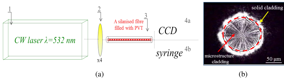
Figure 5.11: (a) Scheme of the optical setup for the photo-initiation process, and (b) the image of the output of the fibre during the polymerisation process
