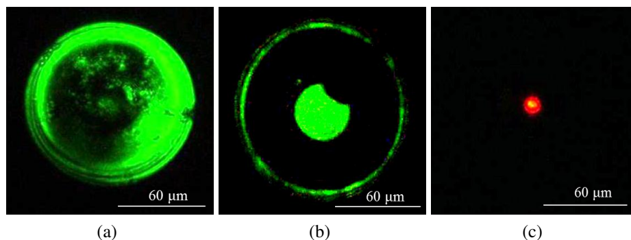
Figure 7.8: The images of collapsed fibres, where the first two images present the fibre during the alignment, where (a) shows the poor light interaction of light and sample, (b) the good interaction, and (c) shows the fibre near field during the fluorescence measurement
