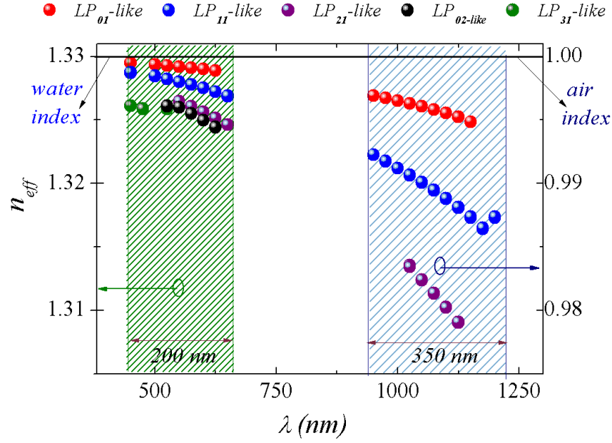
Figure 3.6: Graph of modes analysis for HC-PCF 1060, where the left y-axis shows the first layer and results for the changed refractive index for 1.33 within all air channels, the green dashed area shows a new shifted band. The right y show the second layer and results for the unchanged refractive index with the blue dashed area as the propagation band. Dots for both layers indicate optical modes as: red- LP_{01} -like, blue- LP_{11} -like, purple- LP_{21} -like, black- LP_{02} -like, green- LP_{31} -like
