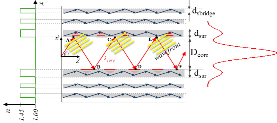
Figure 2.4: Schematic drawing of optical rays' path in the hollow-core PCF, where rays with a navy blue colour indicate wavelengths, which are not propagated in the air-core (resonant wavelengths), and the wavelengths which propagate within the core (red rays) (antiresonant wavelengths)
