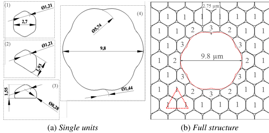
Figure 3.2: Scheme of the fibre drawing for a simulations, where in (a) are shown individual units: (1) is a base unit, (2) is one of two units of the first hole's ring, (3) is the other unit of the first ring, and (4) is the core, (b) complete created fibre structure
