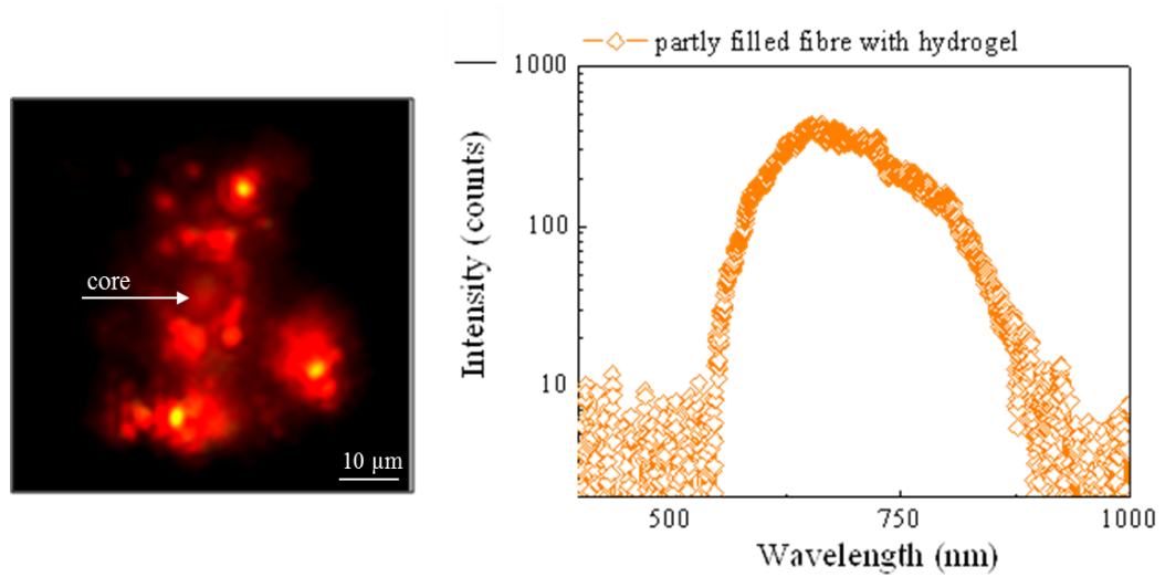
Figure 6.8: The near field image of HC-PCF with corresponding transmitted spectrum
