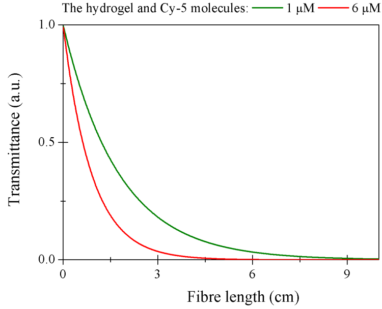
Figure 6.13: Graph of the output intensity for the hydrogel sample with two concentrations of Cy-5 fluorochrome: 1 \mu\text{M} (green line) and 6 \mu\text{M} (red line)
