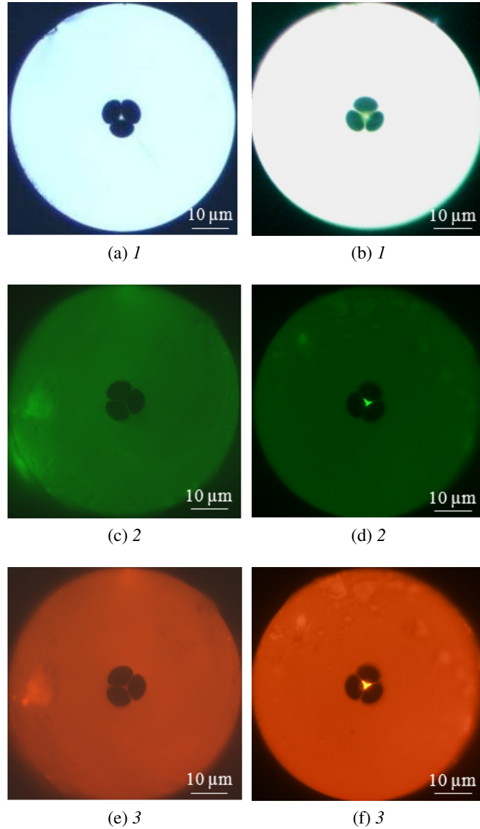
Figure 8.13: The suspended-core fibre with the grown hydrogel in the cladding holes and around the core, the first (1) row are imaged in an optical microscope, in the second (2) row are images for a fluorescence microscope using FITC dichroic filter, and the third (3) row are images for a fluorescence microscope using a Cy-3 dichroic filter
