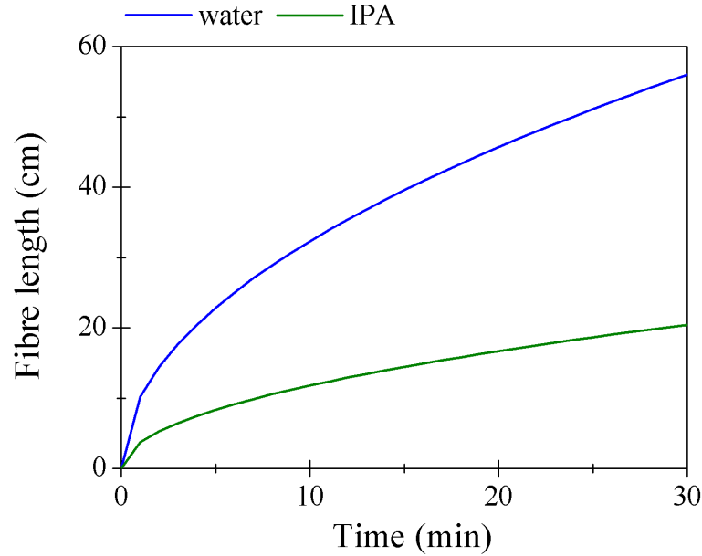
Figure 2.10: Graph of simulated time of filling the core of HC-PCF 1060 with water (blue line) and IPA (green line)
