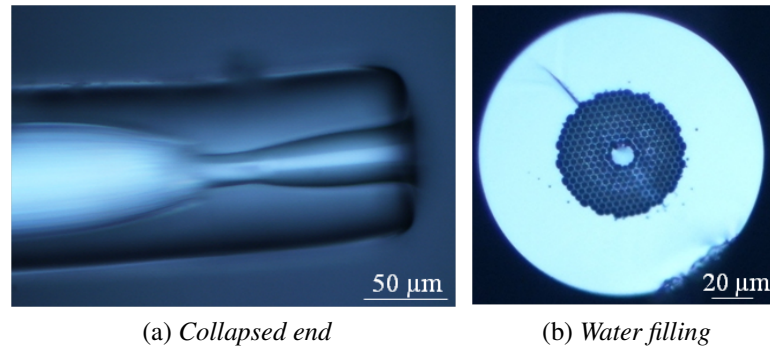
Figure 6.1: The water-core fibre, where (a) is preparation for a selective filling, (b) the core filled with water
