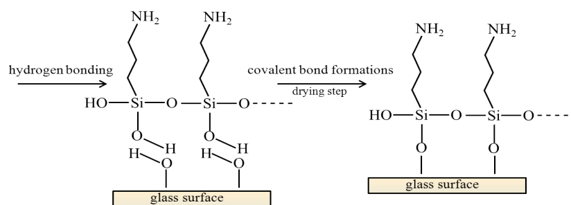
Figure 2.17: Scheme of an attaching silanising agent APTMS to a glass surface (part 2)
