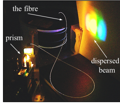
Figure 3.11: The supercontinuum fibre in a spool, with example of the fibre glow
