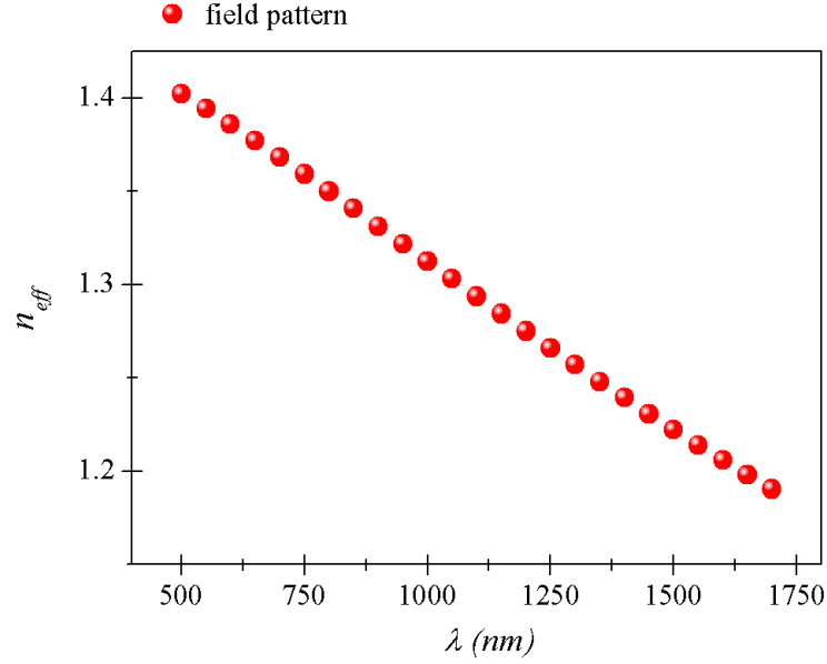
Figure 8.5: Graph of effective index against wavelength, for the field pattern with the highest intensity centred at the core
