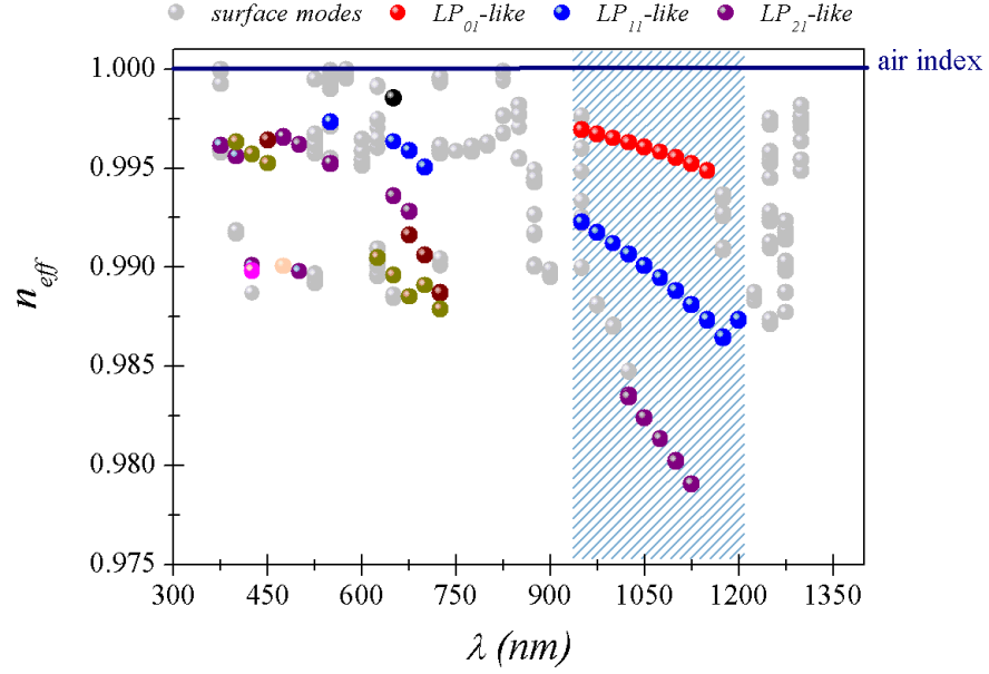
Figure 3.5: Graph of the effective index and wavelength for hollow-core PCF 1060, where dots show the field pattern which resembles optical modes for standard optical fibre as dots: red LP_{01} -like, blue LP_{11} -like, purple LP_{21} -like, violet LP_{12} -like, dark yellow LP_{31} -like, yellow LP_{51} -like, magenta LP_{61} -like and light-grey dots are surface and leaky modes, the dashed area represents the propagation band
