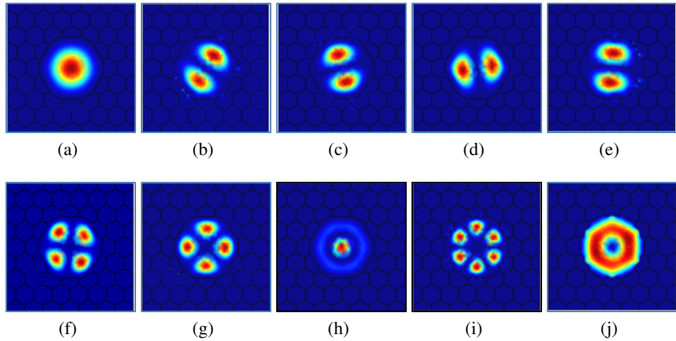
Figure 3.4: Generated field patterns with the aid of the numerical modelling (Comsol): (a) is the fundamental-like mode LP_{01} -like, and higher order modes: (b-e) is LP_{11} -like for a different geometric orientation of the electric field as: (b) right-elliptical, (c) left-elliptical, (d) vertical, (e) horizontal, (f-g) LP_{21} -like, (h) LP_{02} -like, (i) LP_{31} -like, and (j) donut shape
