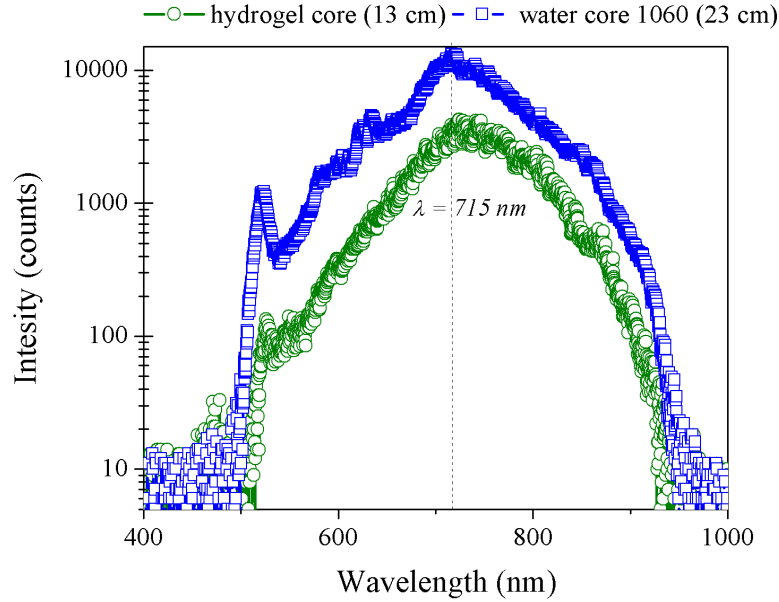
Figure 6.5: Supercontinuum propagation through the core filled with hydrogel (green open circle line) and through water (blue open square line)
