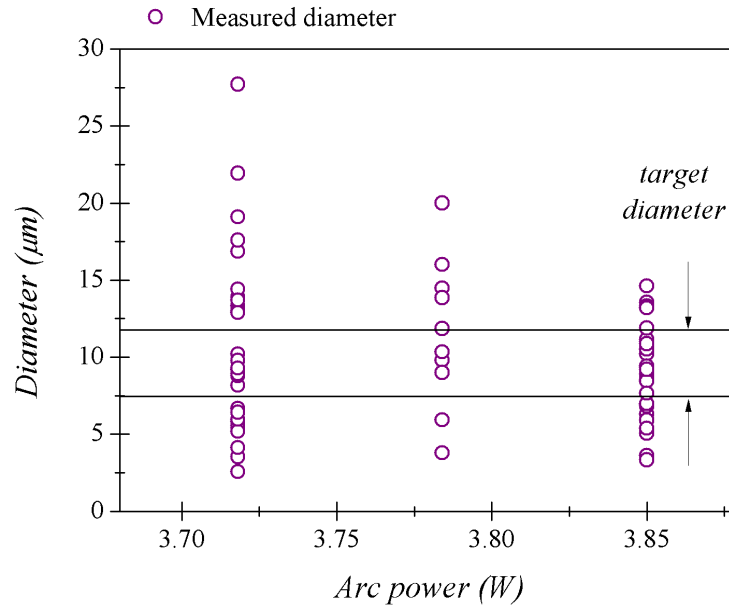
Figure 4.4: Graph of data for collapsing fibre channels as a function of arc power
