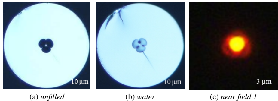
Figure 8.11: The cross-section of P3 suspended-core fibre, (a) unfilled and (b) filled with water, (c) near-field image for supercontinuum propagation
