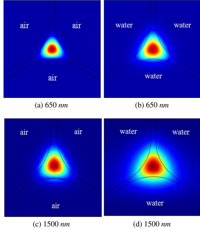
Figure 8.4: Field patterns distribution generated for wavelengths: (a-b) 650 nm and (c-d) 1550 nm - unfilled and filled with water, respectively
