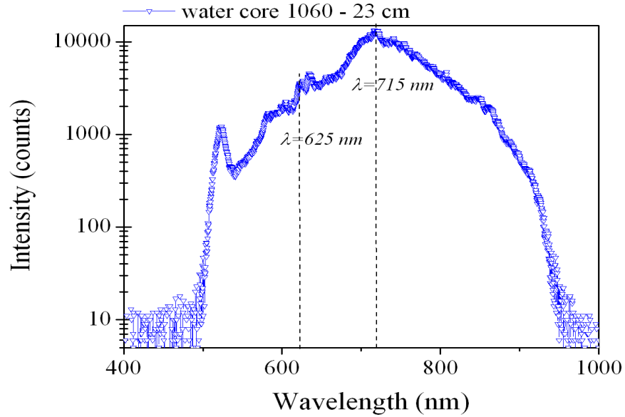
Figure 6.3: The supercontinuum propagation through the fibre selectively filled with water, the intensity of light was reduced with a neutral density filter with OD 2.0
