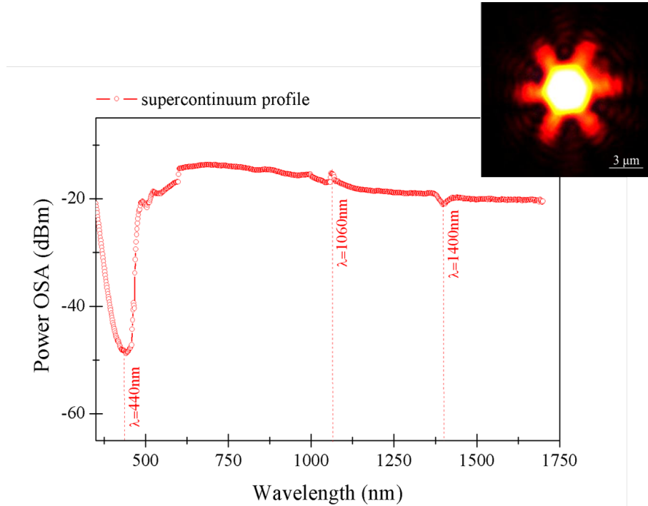
Figure 3.12: The supercontinuum profile detected with OSA, with a resolution 10 nm and inset near-field image of the HNL-PCF fibre
