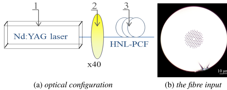
Figure 3.10: (a) The schematic optical setup to generate the supercontinuum signal, where: (1) indicates the Nd:YAG laser, (2) is the focusing lens, (3) is highly-nonlinear PCF (b) the cross-section of HNL-PCF
