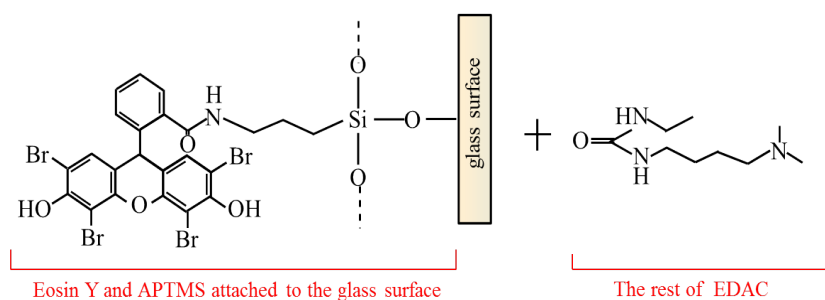
Figure 2.21: Scheme of the silanised glass surface and the rest of EDAC
