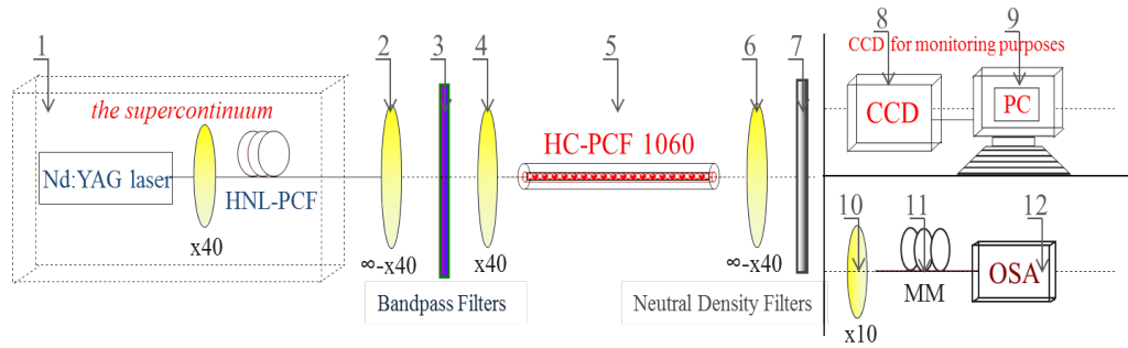
Figure 3.15: The experiment setup to detect transmission spectra, where: (1) shows the supercontinuum source, (2) is a collimating lens, (3) is a bandpass filter, (4) is a focusing lens, (5) is the fibre sample (HC-PCF 1060), (6) is a collimating lens (7) neutral density filters, (8) a CCD camera, (9) computer and software, (10) a collimating lens, (11) a multimode fibre, and (12) indicates an optical spectroanalyser
