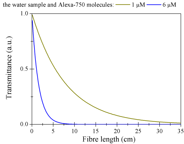
Figure 6.14: Graph of the output intensity for the fibre filled with water solution of Alexa-750 fluorochrome with two concentrations of 1 \mu\text{M} (dark-yellow line) and 6 \mu\text{M} (blue line)
