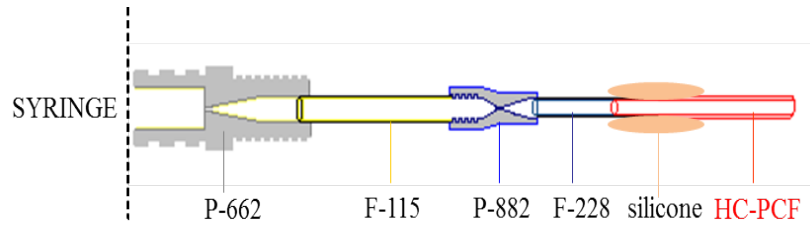
Figure 4.12: The scheme of a syringe setup with joins between the syringe and the fibre
