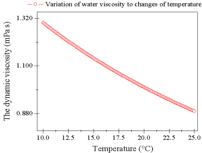
Figure 2.13: Graph of dynamic viscosity of water with temperature changes
