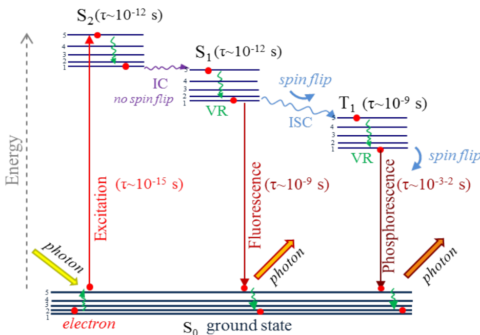
Figure 2.29: Jabłoński's diagram for fluorescence excitation, with VR-vibrational relaxation, IC-internal conversion, and ISC-internal system crossing
