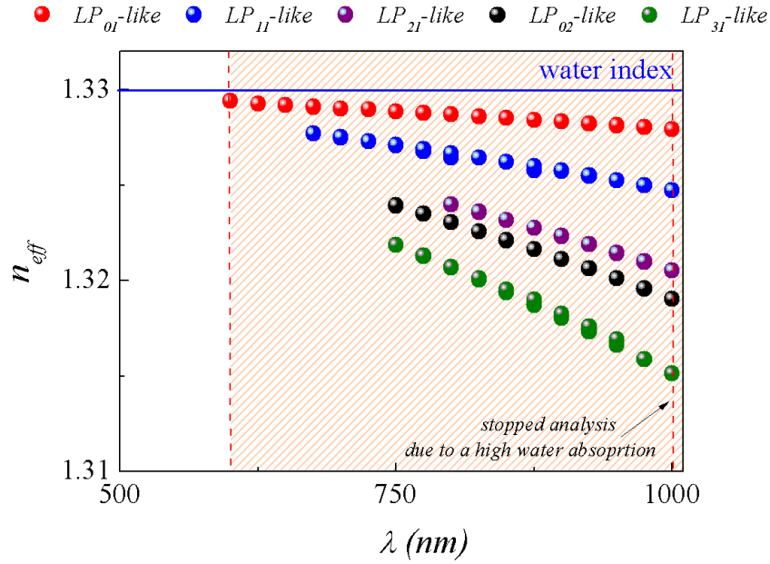
Figure 3.7: Graph of mode analysis for hollow-core PCF 1060 with changed refractive index for 1.33 only within the core of the fibre; dots show the modes as: red- LP_{01} -like, blue- LP_{11} -like, violet- LP_{21} -like, black- LP_{02} -like, green- LP_{31} -like, the dashed area represents the transmission windows
