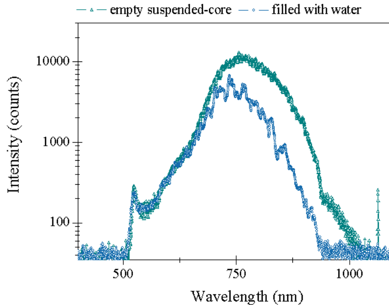
Figure 8.12: The supercontinuum propagation profile in suspended-core optical fibre, where a dark cyan line represents unfilled fibre, a blue line that filled with water
