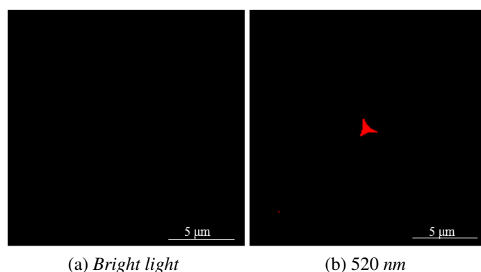
Figure 8.15: The suspended-core fibre with the grown hydrogel, (a) no evidence of DNA probe, (b) Cy-5 labelled DNA are trapped in the core of fibre
