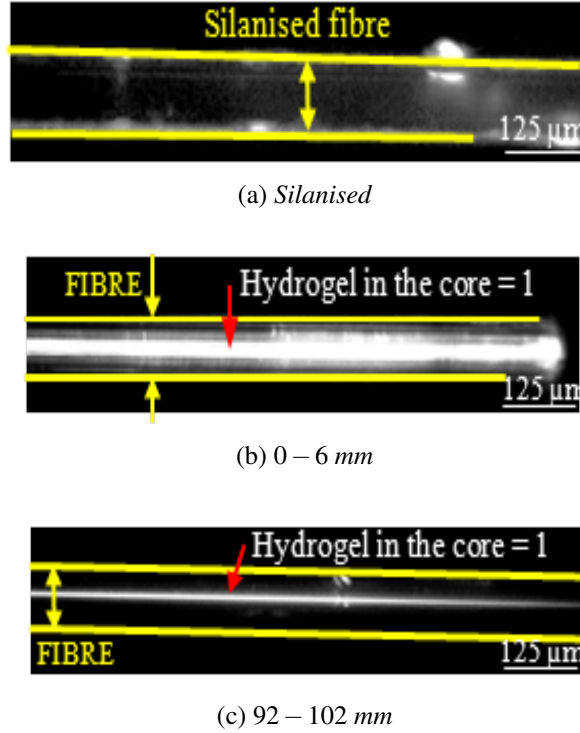
Figure 5.17: The images of the side view of the fibre (between the yellow lines), when (a) the fibre was silanised, (b) the hydrogel emits the light from the cladding and the core, (c) the hydrogel is in the core
