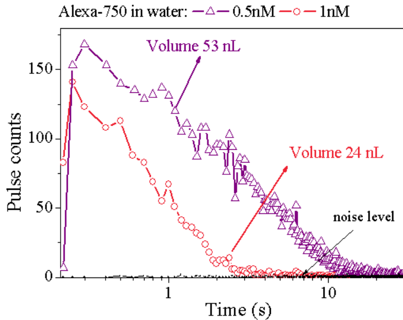
Figure 7.6: The fluorescence detection for 1 nM filled core (red circles line) and 0.5 nM filled core and surrounding 18 holes (purple triangles line)
