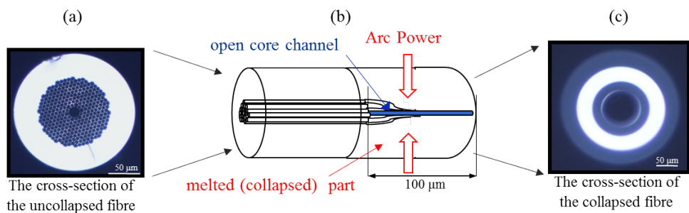
Figure 4.1: The scheme of the collapsing process, (a) end-facet of the fibre before collapsing, (b) schematic drawing of a cross-section of the fibre during collapsing, (c) end-facet of the fibre after the collapsing process
