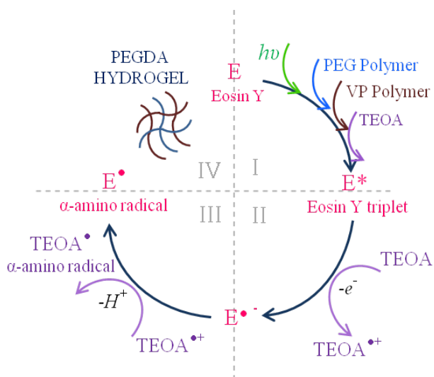
Figure 2.24: Complete process of the PEGDA hydrogel polymerisation
