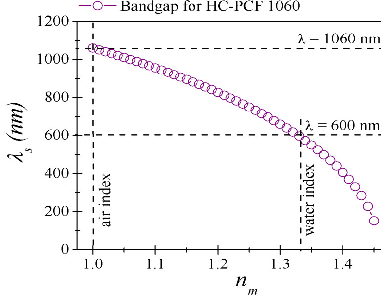
Figure 2.5: Graph of photonic bandgap shift guidance in HC-PCFs, due to changes in the refractive index within the fibre
