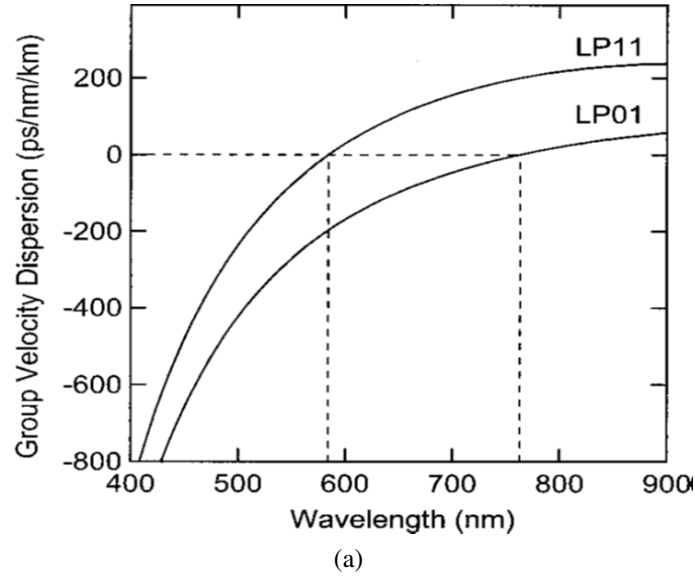
Figure 3.13: Dispersion graph for HNL-PCF fibre according to [154]
