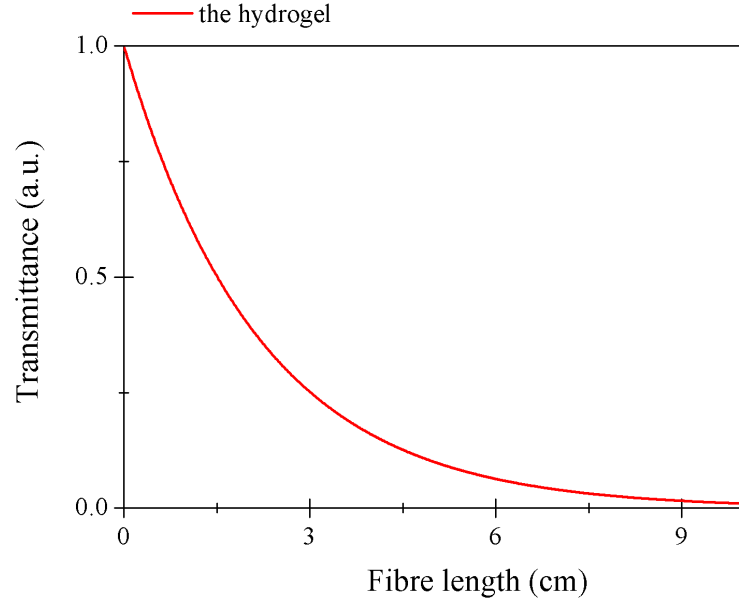
Figure 6.10: The fibre length against the transmitted light for the fibre filled with the 25% PEGDA hydrogel (red line)
