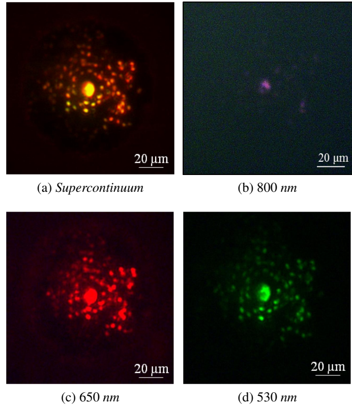
Figure 6.7: The near-field images for the hydrogel-filled fibre, when (a) the entire supercontinuum was propagated, and filtered spectrum using the bandpass filters centred at (b) 800 nm, (c) 650 nm, and (d) 530 nm
