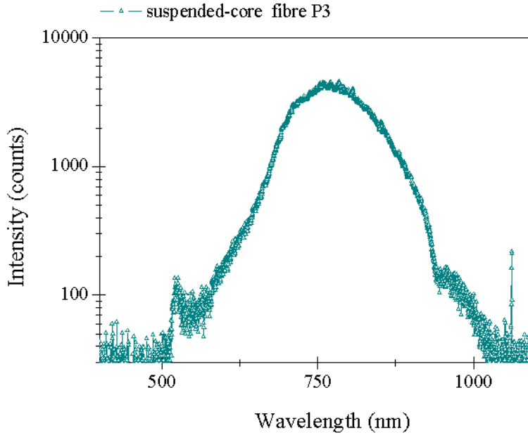
Figure 8.9: The supercontinuum propagation profile for the P3 suspended-core optical fibre
