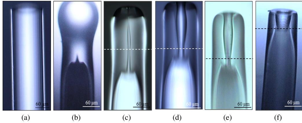
Figure 4.3: (a) the side-view of the fibre before collapsing; the side images of collapsed fibres, where different arc time and arc power were applied for: (b) 6.16 W/2.5 ms, (c) 4.18 W/500 ms, (d) 3.85 W/480 ms, (e) 3.71 W/460 ms, (f) 3.25 W/70 ms, and a dashed line indicates where the core diameter was measured
