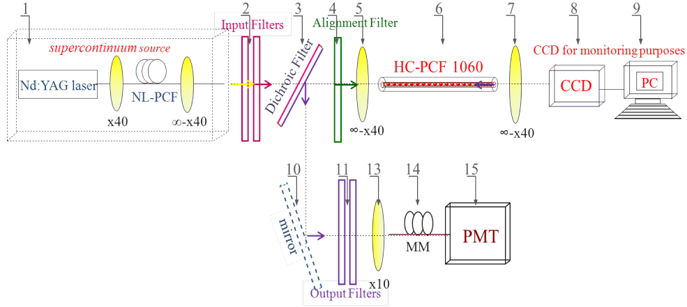
Figure 7.4: The scheme of the optical setup where: HNL-PCF=highly nonlinear PCF, IF =input filters, DF=dichroic filter, AF=alignment filter, OF= output filters, PMT = Photomultiplier tube, MM=multimode fibre. The HC-PCF output was connected a CCD for monitoring purposes
