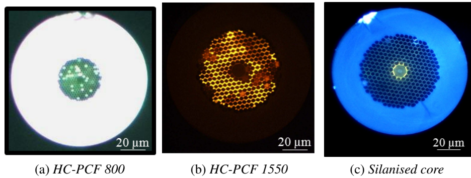
Figure C.2: The cross-section of fibre: HC-PCF 1550 and HC-PCF 800 with examples of non-uniform surface coverage, (a,b) in the optical microscope; (c) when only core is silanised
