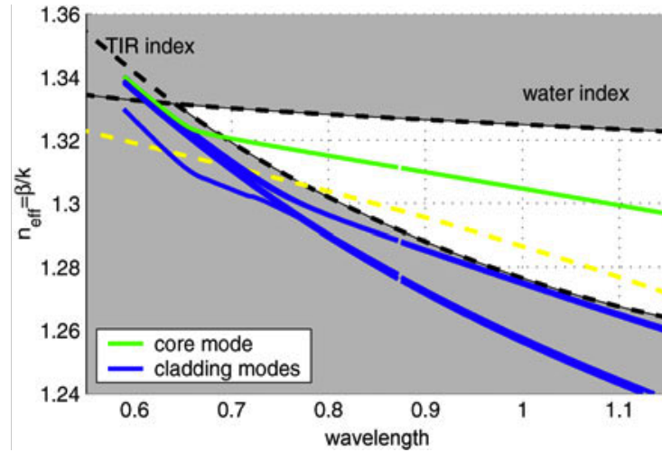
Figure 2.6: Graph of index-guiding, with a green line indicating a core-mode guidance within the region between the water index and the total-internal reflections (TIR) edge - shown with black-dashed lines. The blue lines (in the dark area) illustrate the guidance in the fibre cladding, courtesy of [17]
