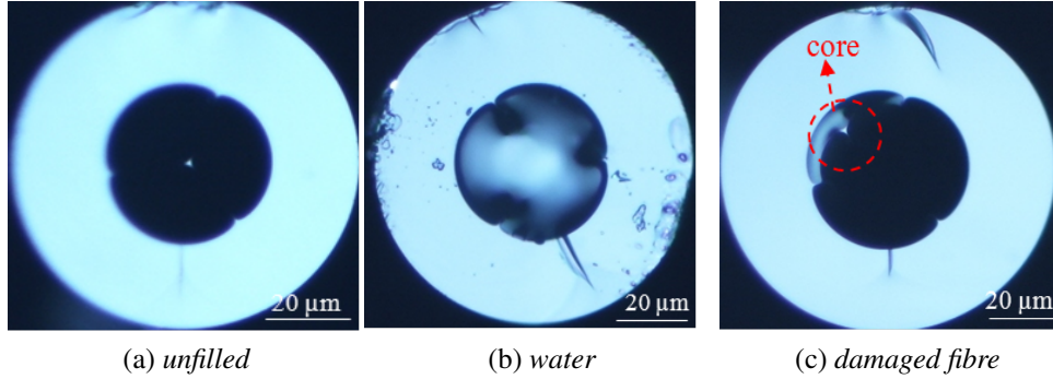
Figure 8.10: The cross-section of P7 suspended-core fibre during a filling with water
