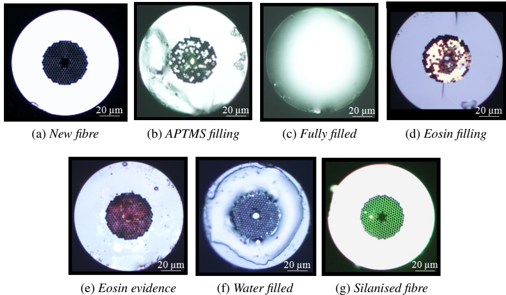
Figure 5.5: The cross-section of HC-PCF 1060 for the silanisation process
