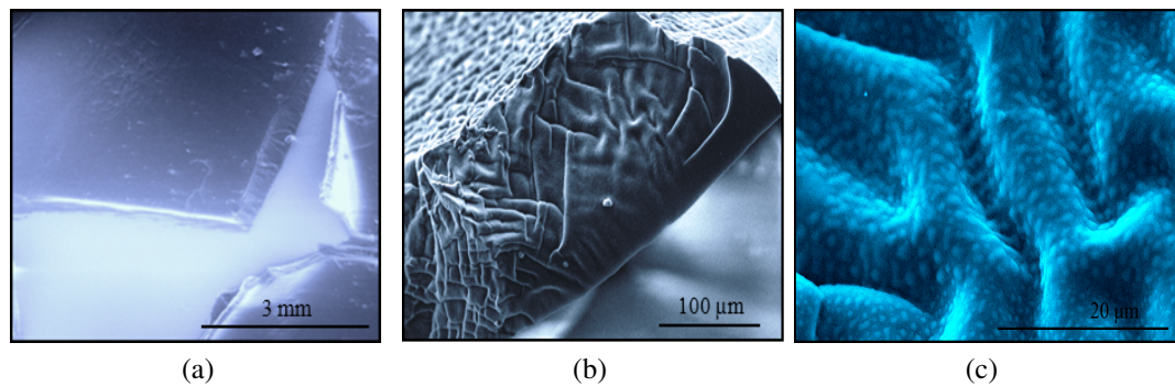
Figure 5.1: The SEM images of the PEGDA hydrogel with (a,b) 25% of concentration and (c) 65%. These hydrogel samples are grown on glass
