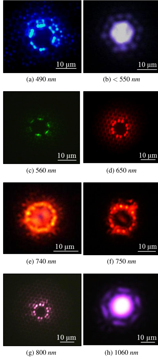
Figure 3.19: The near field images for a different band pass filters (a, c-f), where (b) is for a low-pass filter
