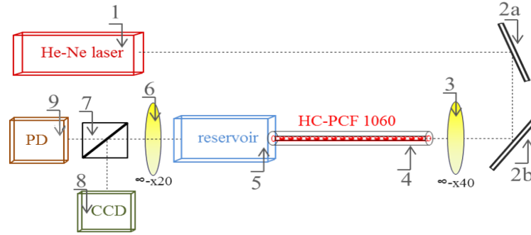
Figure 4.13: The optical setup for nano-litre fibre-viscometer, where He-Ne is a helium-neon laser at 632 nm, HC-PCF 1060 is the fibre sample, CCD camera and PD indicates a photo-diode
