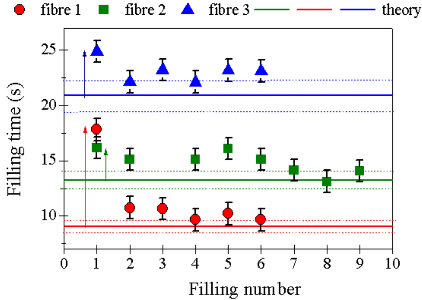
Figure 4.9: Graph of time delays for the first filling for three fibres: blue triangles indicate 64 mm fibre length, green squares indicate 51 mm fibre length, and red circles indicate 42 mm fibre length with black lines, which display the error bars. The solid lines show the theory line and dashed lines display the error range for the theory line
