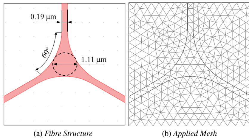
Figure 8.2: The fibre structure (a) applied in a numerical modelling (b) applied mesh for the fibre structure
