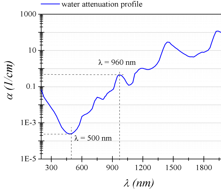
Figure 2.7: The water attenuation profile adapted from reference [86]
