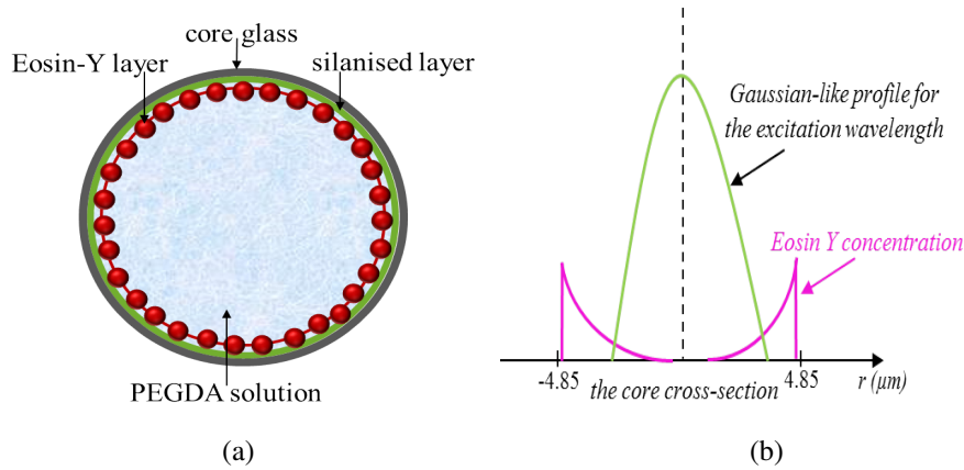
Figure 5.9: (a) Illustration of the fibre cross-section with red circles indicating Eosin Y molecules, (b) the profile of the Gaussian-like profile in the core cross-section
