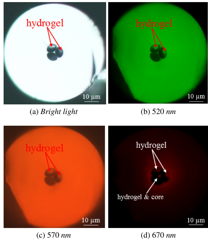
Figure 8.14: The suspended-core fibre with the hydrogel grown in the cladding holes and around the core, observed through (a) optical microscope, (b,c,d) fluorescence microscope, with (b) FITC dichroic filter, (c) Cy-3 filter, (d) Cy-5 filter
