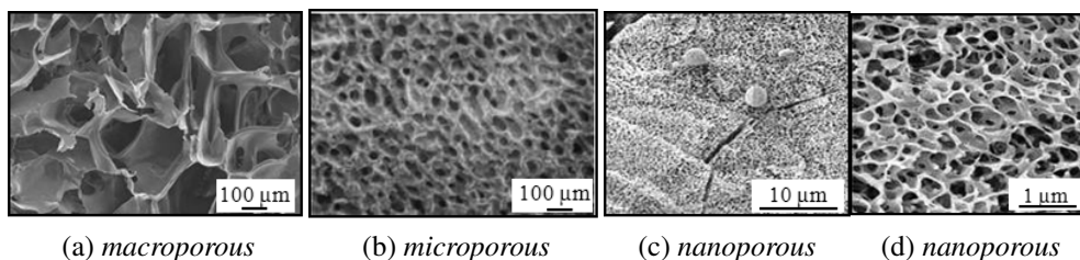
Figure 2.15: The SEM images of porous hydrogel, where (a) is macroporous hydrogel [112], (b) is microporous hydrogel [113], (c) and (d) are nanoporous hydrogel shown in [114]
