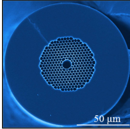
Figure 3.1: Cross-section of HC-PCF 1060, courtesy of NKT Photonics A/S
