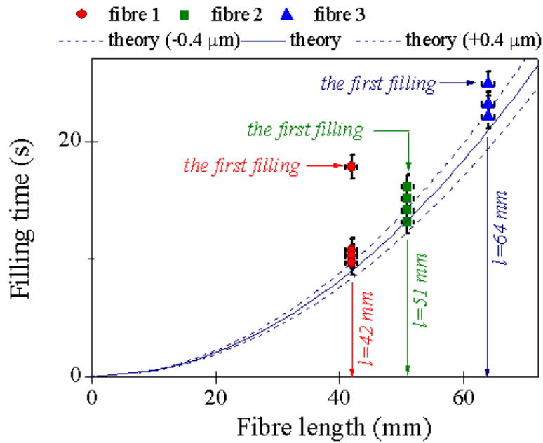
Figure 4.8: Graph of the filling process of three fibres with water, where: blue triangles indicate 64 mm fibre length, green squares indicate 51 mm fibre length, and red circles indicate 42 mm fibre length with black lines, which display the error bars. The solid lines show the theory line and dashed lines display the error range for the theory line
