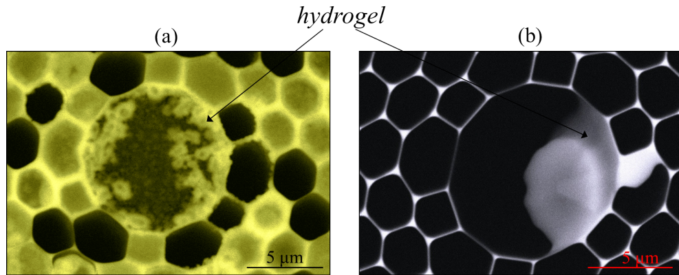
Figure 5.12: SEM images of the fibre core with a growing hydrogel inside, (a) with a yellow hue, and (b) in black and white
