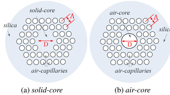
Figure 2.2: The scheme of the fibre structure, where the pitch is shown for a) solid-core and b) air-core fibre
