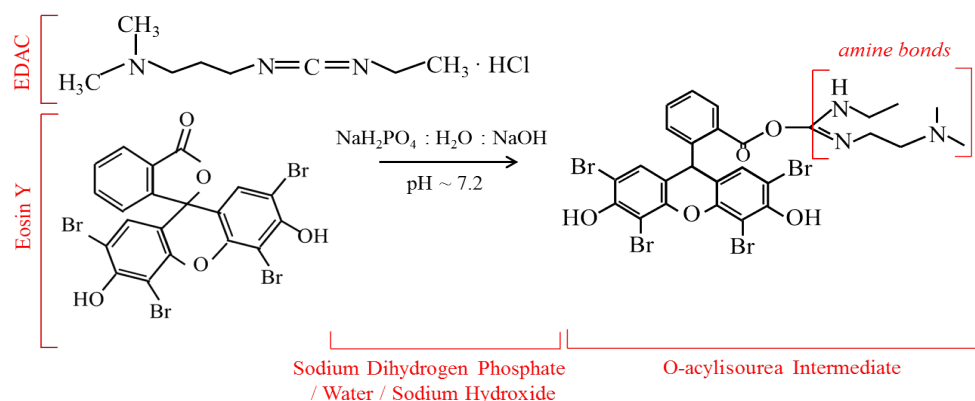
Figure 2.19: Scheme of EDAC and Eosin Y reaction within a lower pH solution, to form a O-acylisourea intermediate
