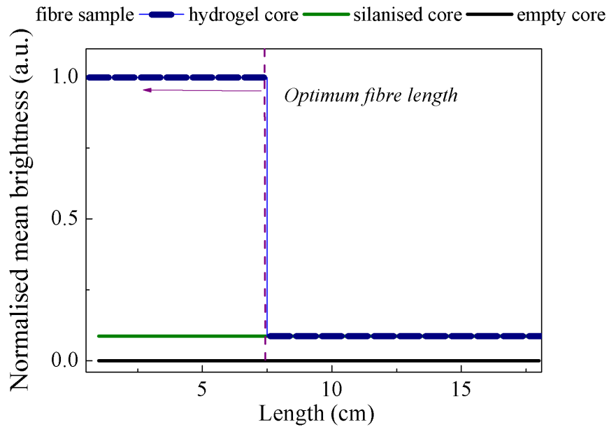
Figure 5.15: Graph of the hydrogel distribution in the fibre, due to the cleaving method
