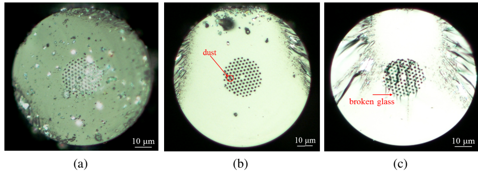
Figure 3.14: The cross-section images of HNL-PCF (a) with dusts on the fibre surface, (b) other example of the fibre contamination, (c) example of broken silica bridges in the microstructure cladding
