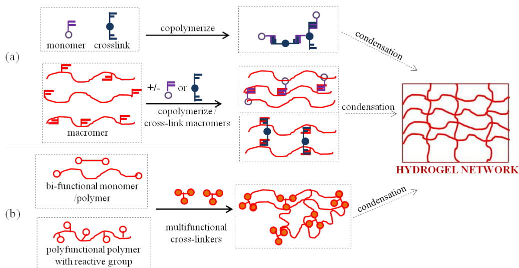
Figure 2.14: The schematic illustration of two methods for forming cross-linked hydrogel by (a) free radical reactions or (b) condensation reaction of multifunctional cross-links
