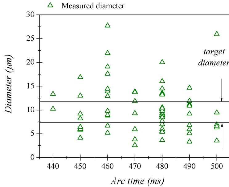
Figure 4.5: Graph of data for collapsing fibre channels as a function of arc time
