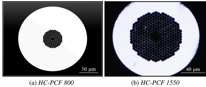
Figure A.1: The cross-section images of (a) HC-PCF 800 and (b) HC-PCF 1550 courtesy of NKT Photonics A/S
