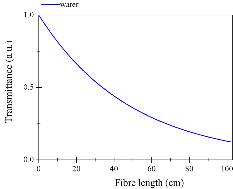
Figure 6.11: The fibre length against the transmitted light for the fibre filled with water (blue line)
