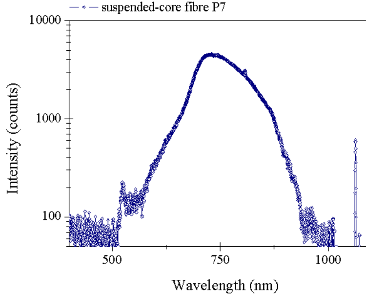
Figure 8.8: The supercontinuum propagation profile for the P7 suspended-core optical fibre
