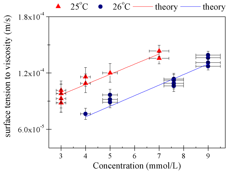
Figure 4.15: The graph of surface to viscosity measurements for glucose solution at different concentrations for two different temperatures: red triangles display 25^\circ Celsius, and blue circles show results for 26^\circ Celsius
