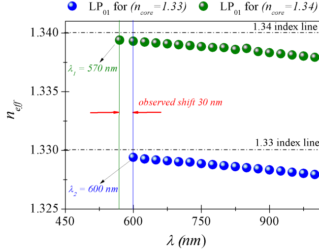
Figure 3.8: Graph of the fundamental-like mode analysis for the filling core with a refractive index material: for n=1.33 (blue dots) and n=1.34 (green dots)
