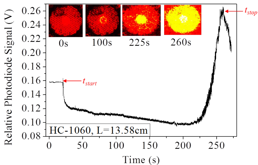
Figure 4.14: The fibre core filling process with attached images from CCD camera during filling process
