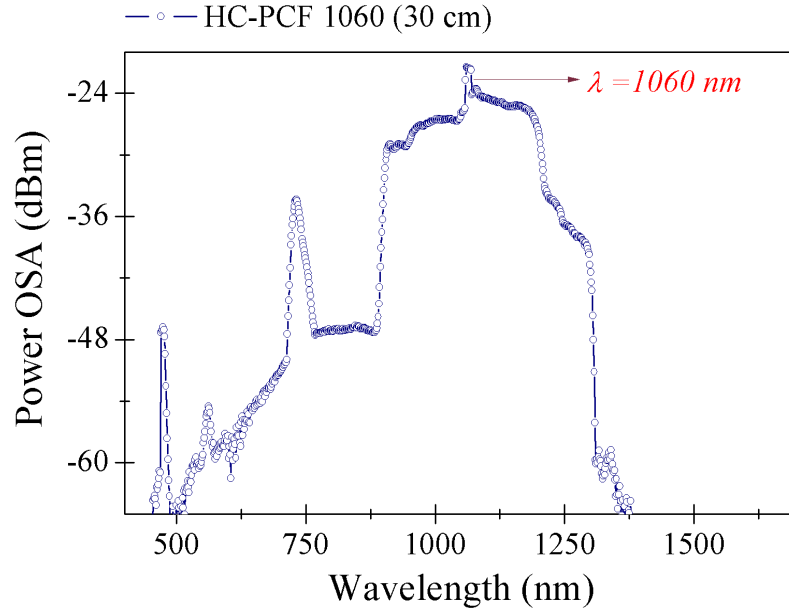
Figure 3.17: The transmitted spectrum for HC-PCF 1060 with a resolution 5 nm for the fibre length of 0.3 m
