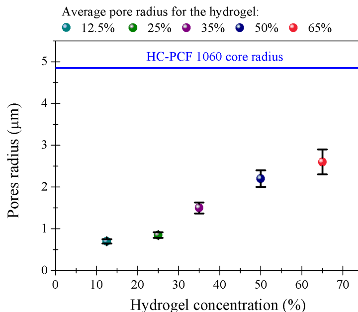
Figure 5.4: Graph of the PEGDA hydrogel concentration as a function of average pore radii for: 12.5% is shown as a dark-cyan dot, 25% as a green dot, 35% as a purple dot, 50% as a navy-blue dot, and 65% is a pink dot; the blue solid line indicates the core radius of HC-PCF 1060, error bars are shown with black lines
