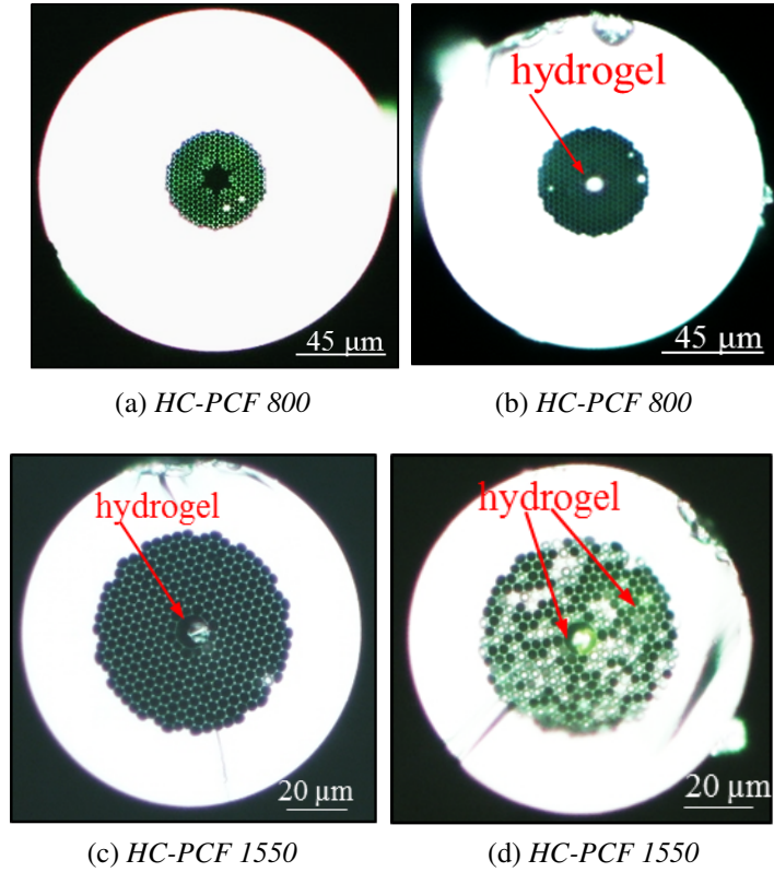
Figure C.3: The cross-section of fibre: HC-PCF 800 (a) the silanised fibre, (b) hydrogel in the fibre core, (c) example of hydrogel grown in the core of HC-PCF 1550 and (d) hydrogel evidence in the fibre cladding channels and in the core
