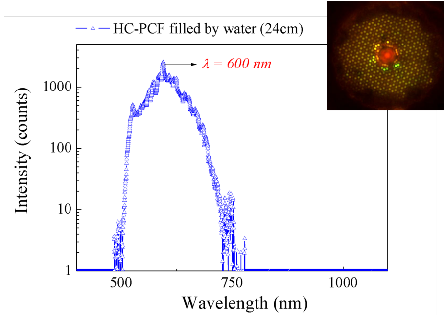
Figure 3.20: The transmitted spectrum of 24 cm HC-PCF filled with water, with attached near-field image at the upper corner
