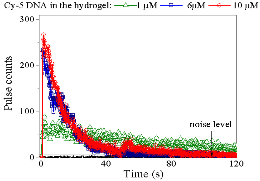
Figure 7.14: Fluorescence measurements as a function of concentration for a Cy-5 DNA probe incorporated into a fibre filled with hydrogel for concentrations: 1\ \mu\text{M} green triangles line, 6\ \mu\text{M} blue squares line, and 10\ \mu\text{M} red circles line
