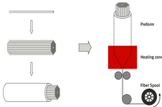
Figure 2.3: Schematic illustration of PCFs fabrication process, courtesy of NKT Photonics A/S
