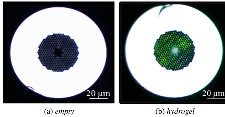
Figure 5.13: The images of HC-PCF 1060, when (a) there is no hydrogel and (b) hydrogel was grown in the core of fibre
