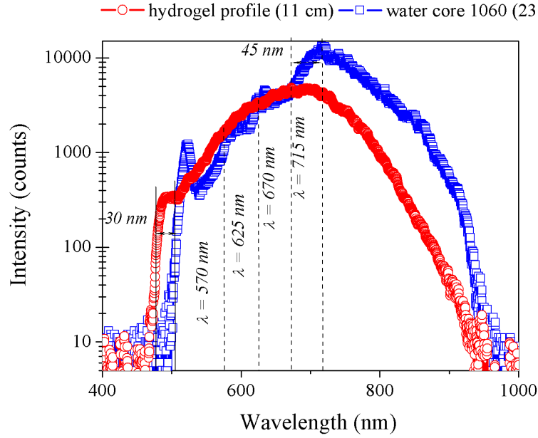
Figure 6.6: Supercontinuum propagation through the core filled with hydrogel (red open circle line) and water (blue open square line)
