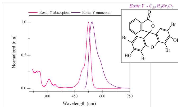
Figure 2.18: Graph of the absorption and emission profile as a function of wavelength, and inset shows the Eosin Y chemical structure
