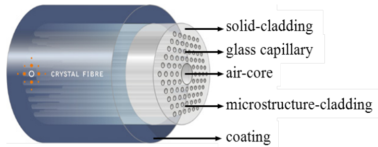
Figure 2.1: Holey fibre, courtesy of NKT Photonics A/S
