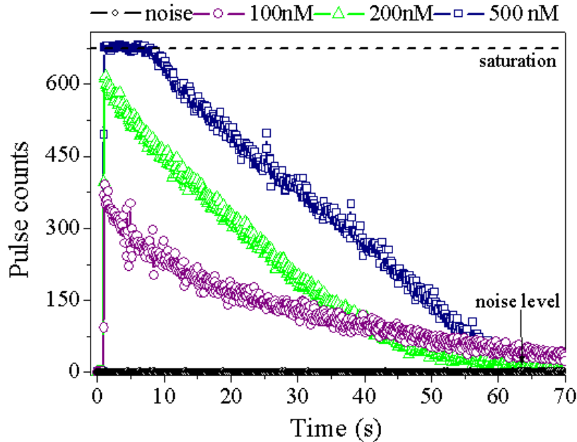
Figure 7.5: Fluorescence curves as a function of concentration for Alexa-750 in a fibre filled with water: purple circles indicate 100 nM, green triangles display 200 nM, blue squares are for 500 nM, and black diamonds are noise level
