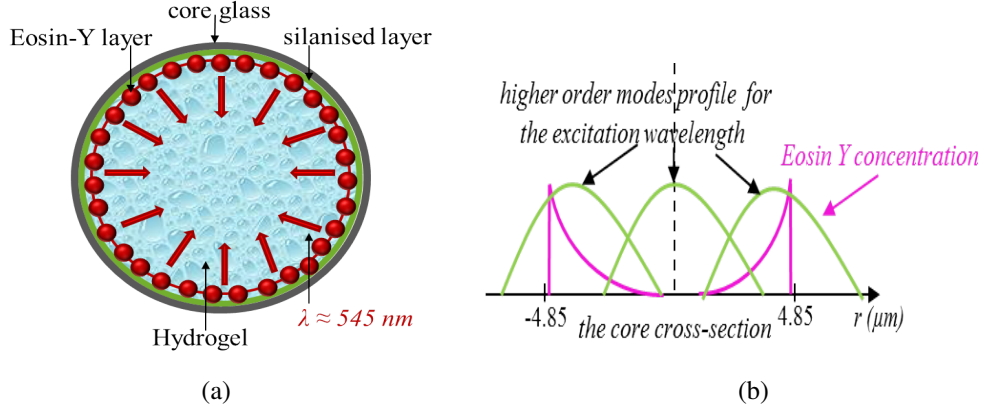
Figure 5.10: Illustration of the polymerisation process inside the fibre core with red circles indicating Eosin Y molecules, where (a) shows the hydrogel growing, and (b) is the intensity profile of higher order mode in the core cross-section
