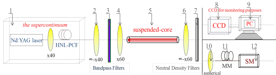
Figure 8.6: The optical setup to detect transmission spectra, with the suspended-core optical fibre, and CCD-camera, PC-desktop, SM-spectrometer, MM-multimode fibre
