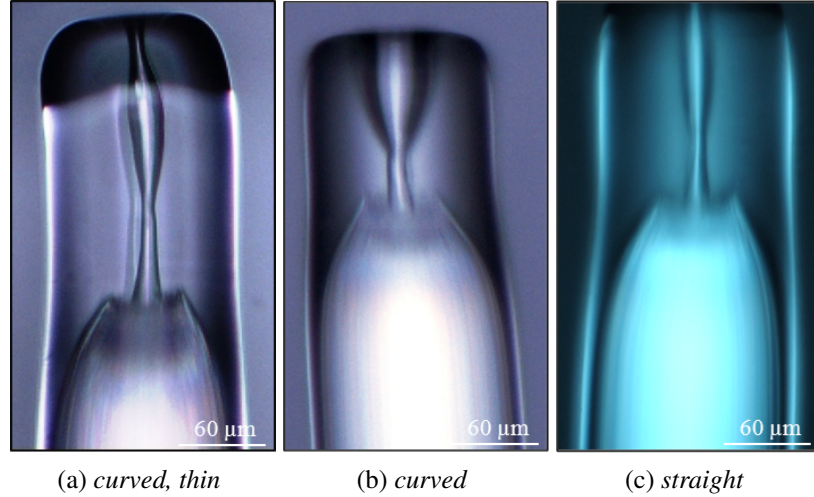
Figure 7.7: The side images of collapsed fibres, where the first two images present the curvature in the core line, the last ideal shape of the opening channel
