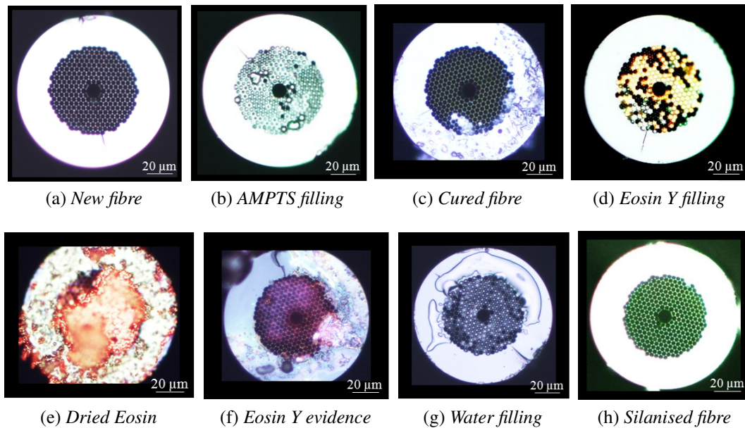
Figure C.1: The array of cross section portrays of HC-PCF 1550 for a silanisation process
