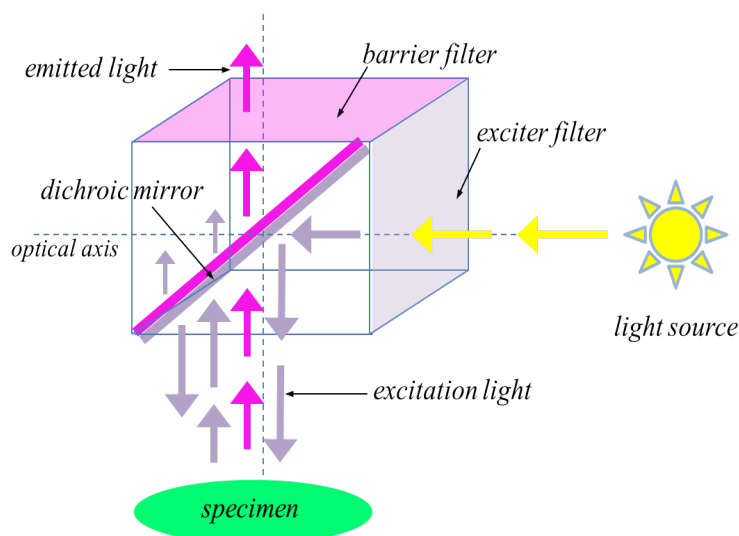
Figure 7.1: Schematic of the cube filter used in the epi-fluorescence microscope
