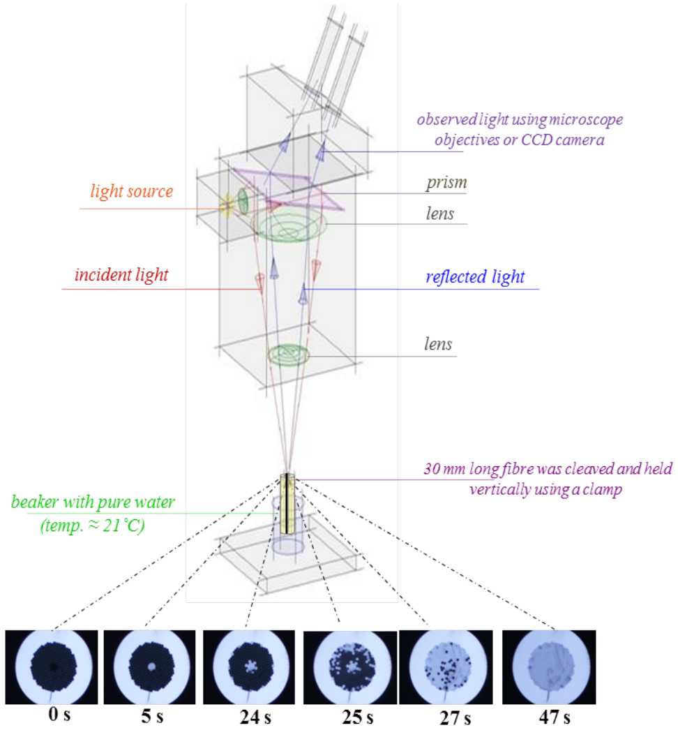
Figure 4.7: The schematic drawing of a microscope setup to record a fibre filling process; at bottom is an array of images of the fibre end-facet recorded during filling of 3 cm of the fibre
