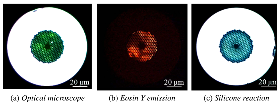
Figure 5.7: The fibre's cross-section images of non-uniform surface coverage: by (a) an optical microscope, (b) a fluorescence microscope, (c) on optical microscope with silicone rubber contamination
