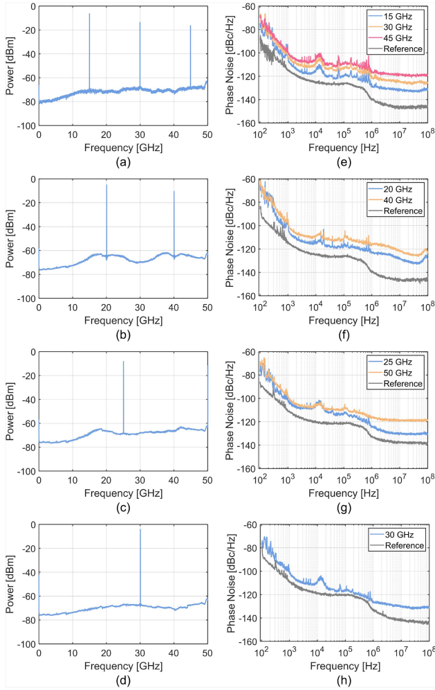
Fig. 9. RF spectrum measured at the photodiode output after feeding it with a gain-switched comb at repetition rates of 15 GHz (a), 20 GHz (b), 25 GHz (c) and 30 GHz (d), respectively. Phase noise measurements for each of the RF lines of the electrical combs (e–h). Grey curve represents the baseline performance of the RF signal source at each fundamental frequency.
