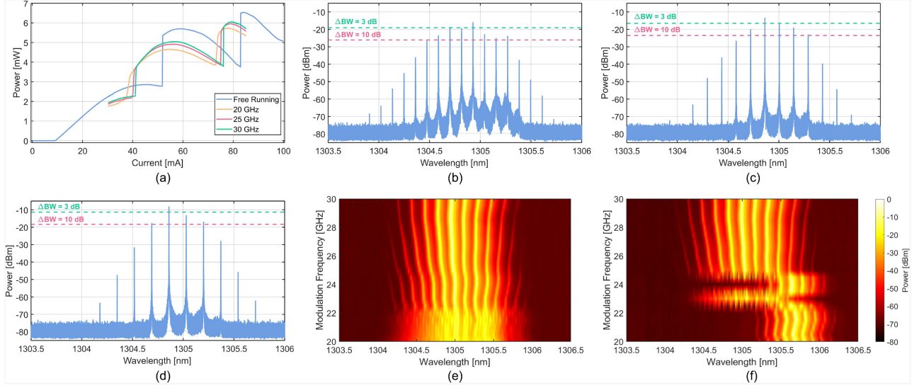
Fig. 8. L-I curves for different modulation amplitudes (a). Comb generation at 20 GHz for I_{bias} = 69 mA and P_{mod} = 19 dBm (b), 25 GHz for I_{bias} = 73 mA and P_{mod} = 19 dBm (c) and 30 GHz for I_{bias} = 74 mA and P_{mod} = 18 dBm (d). Evolution of the generated frequency combs as a function of the modulation frequency at 72 mA (e) and 74 mA (f).
