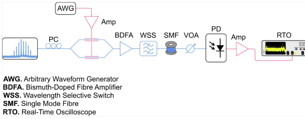
Fig. 12. Frequency upconversion system.
