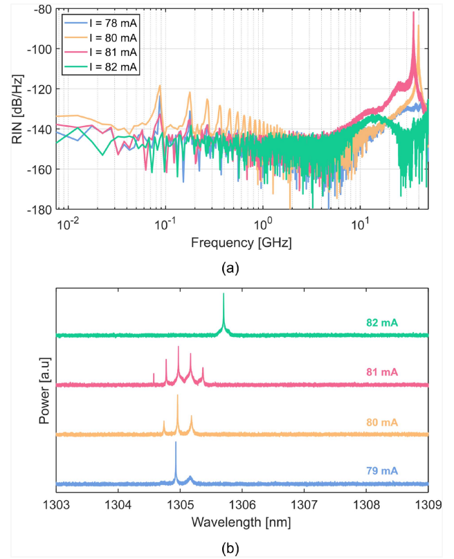
Fig. 5. RIN measurements at 20 °C for different bias currents (a) and their corresponding optical spectra (b).
