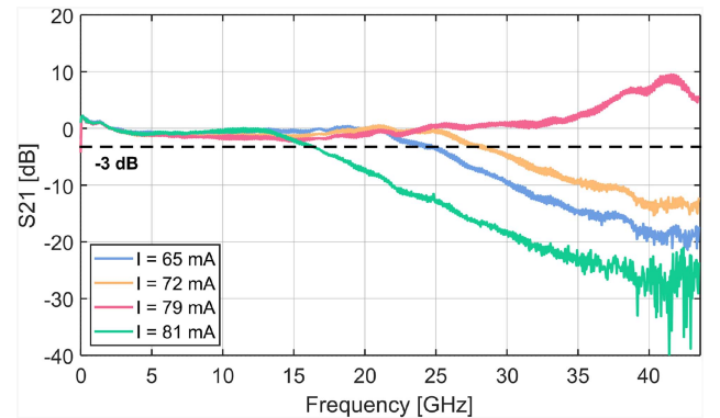
Fig. 7. Laser modulation responses at 20 °C for different bias currents around the second mode hop region. As current increases, the modulation response is enhanced due to a stronger PPR, until the laser mode hops (81 mA), showing a usual single-mode laser behaviour response.
