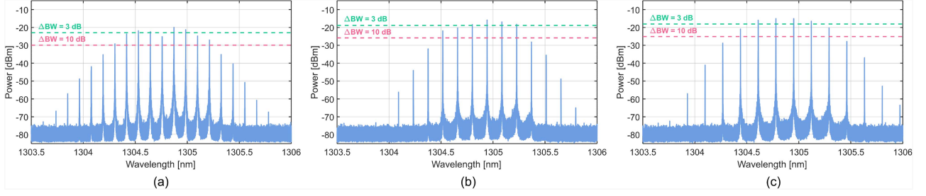
Fig. 11. Expanded comb generation at 20 GHz for I_{bias} = 71 mA and P_{mod} = 21 dBm (a), 25 GHz for I_{bias} = 74 mA and P_{mod} = 21 dBm (b) and 30 GHz for I_{bias} = 74 mA and P_{mod} = 21 dBm (c).
