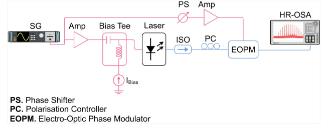
Fig. 10. Comb expansion setup through electro-optic phase modulation.
