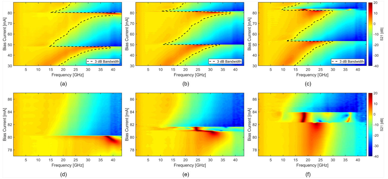
Fig. 6. Measured S21 maps at 20 °C (a), 30 °C (b) and 40 °C (c), and the corresponding detailed views of the second mode hopping point (d)-(f).
