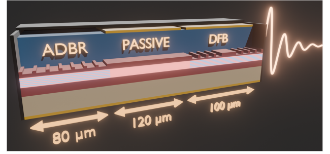
Fig. 1. Illustration of the 300 \mu\text{m} long multi-section laser. From left to right, laser is composed by an 80 \mu\text{m} active distributed Bragg reflector (ADBR), followed by a 120 \mu\text{m} passive waveguide and a 100 \mu\text{m} distributed feedback laser (DFB).
