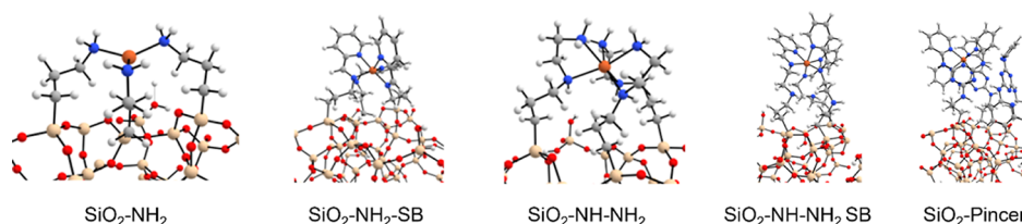
Figure 6. Optimized geometries for the different SiO_2 /ligands coordinating the Fe^{3+} ion. Color scheme: gray (C), white (H), blue (N), orange (Fe), red (O), and beige (Si).
