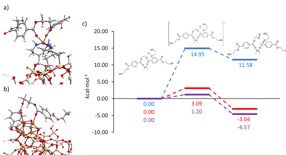
Figure 7. (a) Optimized geometry of the adsorbed PET molecular cluster over the \text{Fe}^{3+} ion. (b) Optimized geometry of the adsorbed PET over the iron oxide NC. Color scheme: gray (C), white (H), blue (N), orange (Fe), red (O), and beige (Si). (c) Relative Gibbs energy profiles at 190 °C (in \text{kcal}\cdot\text{mol}^{-1} ) for PET glycolysis considering EG as a solvent, via uncatalyzed (blue color), catalyzed by a single atom \text{Fe}^{3+} (red color), and catalyzed by the iron oxide nanocluster (purple color).
