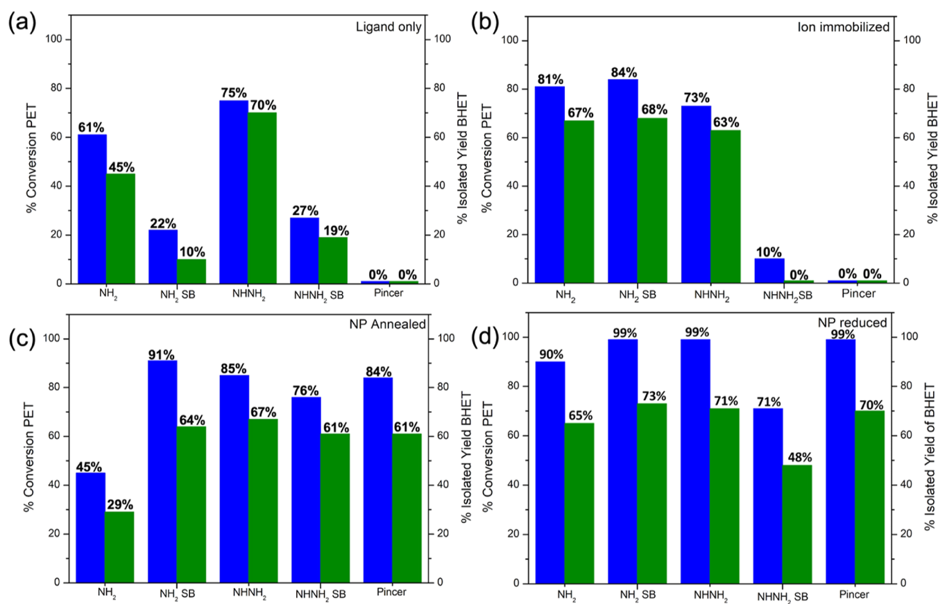
Figure 5. Percentage conversion of PET (blue) and isolated yield of BHET (green) obtained from glycolysis reaction catalyzed by (a) organic ligand modified \text{SiO}_2 (before metal loading), (b) iron-ion-immobilized \text{SiO}_2 , (c) \text{Fe}_2\text{O}_3\text{-NP} \text{SiO}_2 via calcination, and (d) \text{Fe}_2\text{O}_3\text{-NP} \text{SiO}_2 prepared by chemical reduction.
