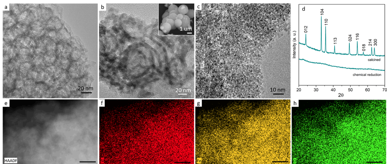
Figure 3. TEM images of \text{SiO}_2 support (a) before Fe-ion immobilized, (b) after calcinations, and (c) after chemical reduction. (d) XRD of \text{SiO}_2 catalysts prepared by calcination and chemical reduction, (e) high angle angular dark field image of \text{SiO}_2 catalyst after chemical reduction, and associated (f) Si, (g) Fe, and (h) O EDX maps. Scale bars in (e,f) are 100 nm.
