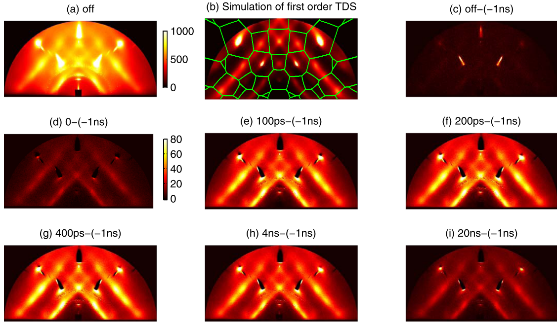
FIG. 1. (a) Room temperature TDS images of Bi at 13 keV oriented with (11-2) nearly parallel to the x-ray direction (grazing angle = 1.5°) with no laser illumination. (b) Calculated first order TDS, on top of which displayed the Brillouin zone boundaries. (c) Difference between laser-off and laser-late frame for comparison. (d)-(i) Differences between a few laser-early frames and laser-late frame, I(t_i) - I(t < 0) , showing the evolution of phonon distribution. ((c)-(i) use the same scale.)
