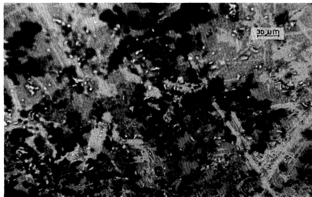
FIG. 4. Optical micrograph of electrodeposited silver in glass A2 ion exchanged for 8 h \times 330 .
