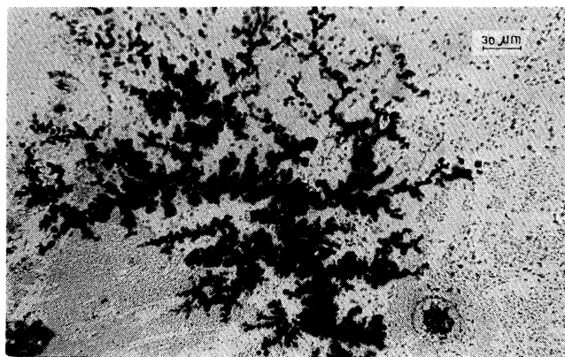
FIG. 3. Optical micrograph of silver deposit in glass A1 ion exchanged for 8 h \times 330 .
