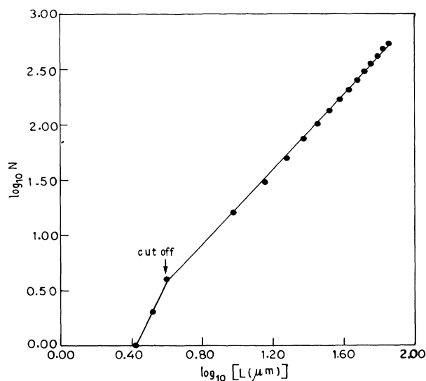
FIG. 12. \log_{10}N vs \log_{10}L for electrodeposited silver in glass no. B1 ion exchanged for 8 h.
