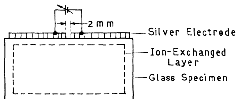
FIG. 1. Sample configuration for electrodeposition experiments.
