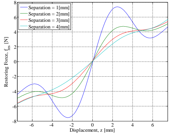
Figure 5: Restoring force as a function of displacement
