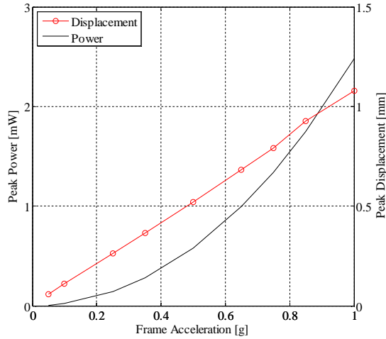
Figure 14: Frame acceleration vs peak power and corresponding peak displacement.
