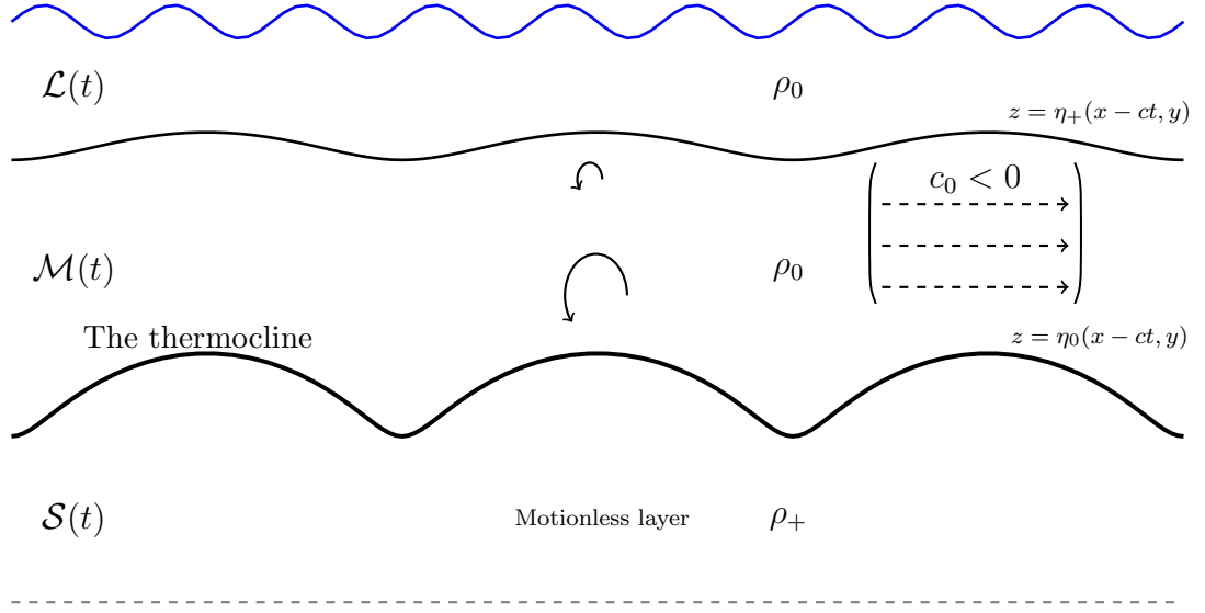
Figure 4.1: Depiction of the different flow regions for a fixed latitude y and a negative constant value of the underlying current c_0 in the layer \mathcal{M}(t) . In the absence of the current, the thermocline is specified by a trochoid propagating eastward at constant speed. The thermocline separates two layer of different densities \rho_0 < \rho_+ in a stable stratification with the denser fluid below.
