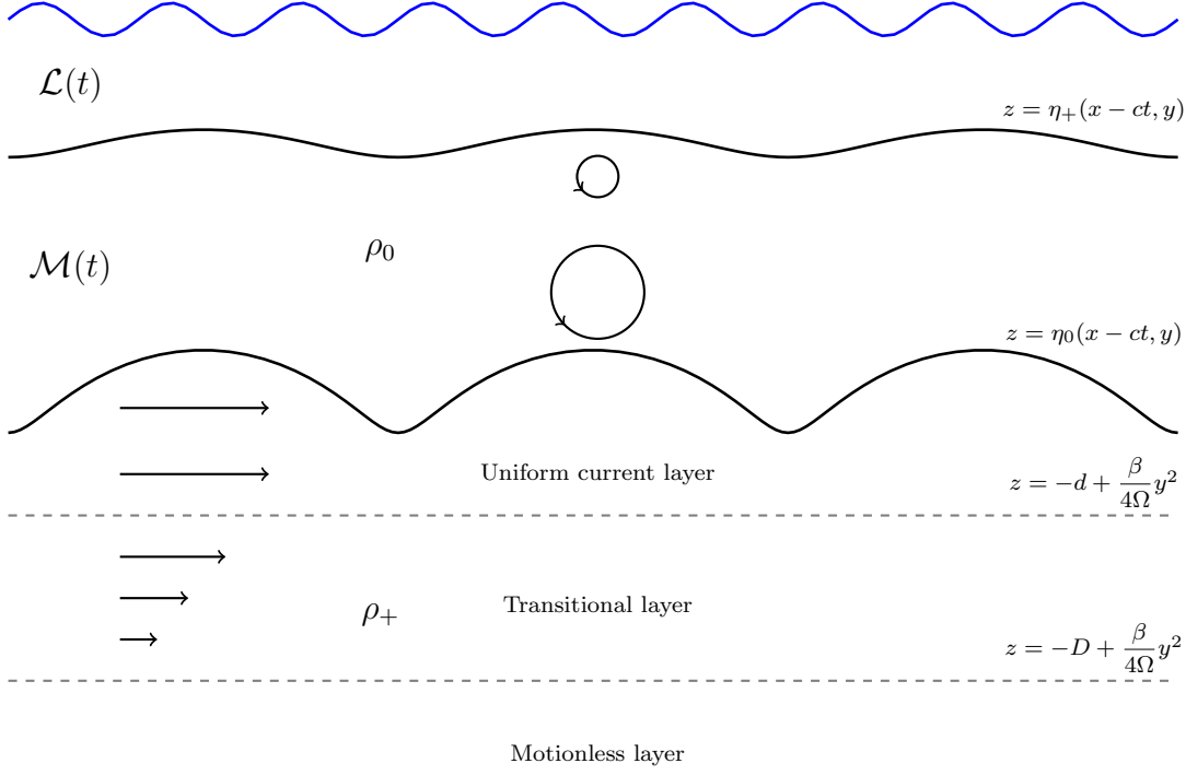
Figure 2.1: Depiction of the different flow regions for a fixed latitude y . \mathcal{L}(t) denotes the region where the wind waves take place and for which the motion is not addressed. The thermocline z = \eta_0(x - ct, y) is specified by an inverted trochoid propagating eastward at constant speed c . Above it, we have the region \mathcal{M}(t) where the oscillations of the thermocline are important and which flow motion constitutes the analysis of this chapter. The two regions below \mathcal{M}(t) accommodate the nonhydrostatic condition by means of a current decaying towards the motionless bed.
