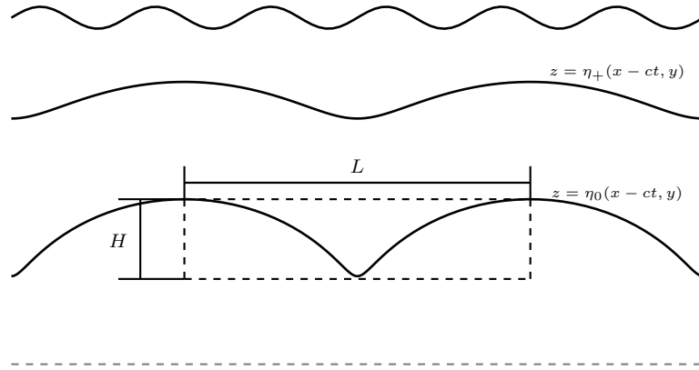
Figure 5.2: At the Equator, the internal wave height is H = \frac{2}{k}e^{-kr_0} and the steepness of the internal wave is given by \tau = e^{-kr_0} , where k = \frac{2\pi}{L} .
