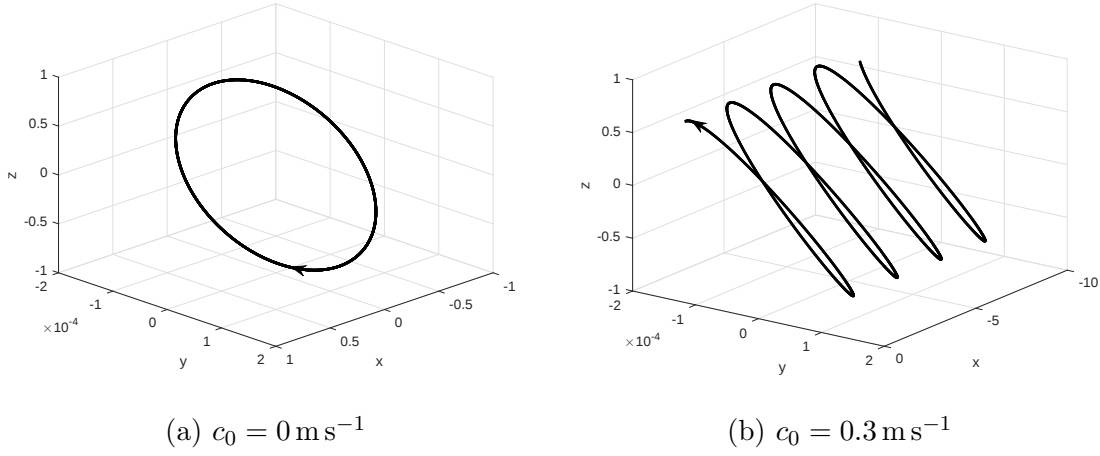
Figure 6.1: Particle paths on the free surface at a latitude \phi = 60^\circ\text{N} for a = 2 \text{ m} and L = 100 \text{ m} .
