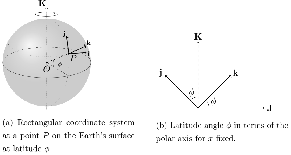
Figure 1.4: Rotational framework of reference.
