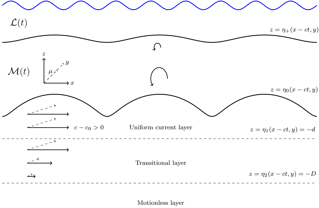
Figure 3.1: Depiction of the different layers in which the fluid motion is divided. The assumption of a two-dimensional flow will not be valid; therefore, this representation should be taken as an approximated sketch of the real situation for a fixed latitude. For both, a positive phase speed c and a positive current c_0 such that c - c_0 > 0 , there is an underlying current in the upper part of \mathcal{M}(t) which flows westward in the longitudinal direction, whereas close to the thermocline z = \eta_0 , there is an uniform eastward current which fades out towards the motionless layer. The flow in the meridional direction will be determined by the current term \mu .
