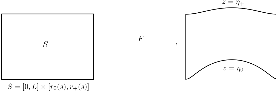
Figure 2.2: Mapping from the labelling domain corresponding to a fixed latitude y = s , a whole period L = 2\pi/k for r \in [r_0, r_+] to the fluid region contained between the thermocline and the upper boundary of \mathcal{M}(t) .
