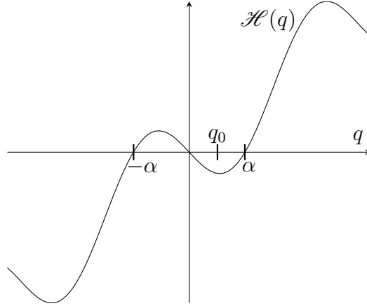
Figure 6.3: A Sketch of the graph of \mathcal{H} . Here q_0 is a local minimum for \mathcal{H} and \mathcal{H}(\alpha) = \mathcal{H}(-\alpha) = 0 .
