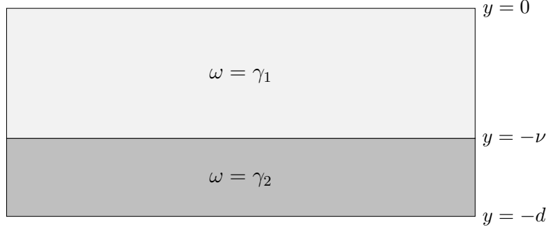
Figure 7.1: Depiction of the two-layer vorticity model for a period L
