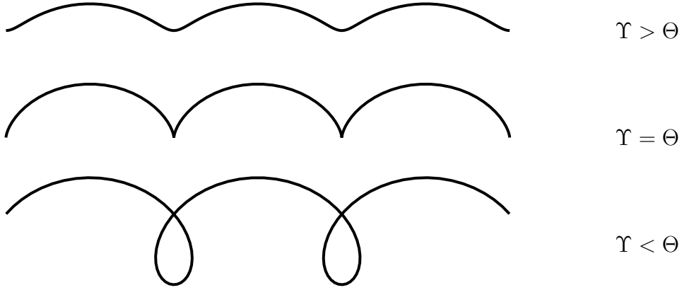
Figure 1.2: Types of trochoids: For the first case, the fixed point is inside the circle and the curve is smooth. In the second case \Upsilon = \Theta , the curve is known as a cycloid and presents peaks where the curve is not differentiable. The third curve results from situating the fixed point outside the circle and it intersects itself.
