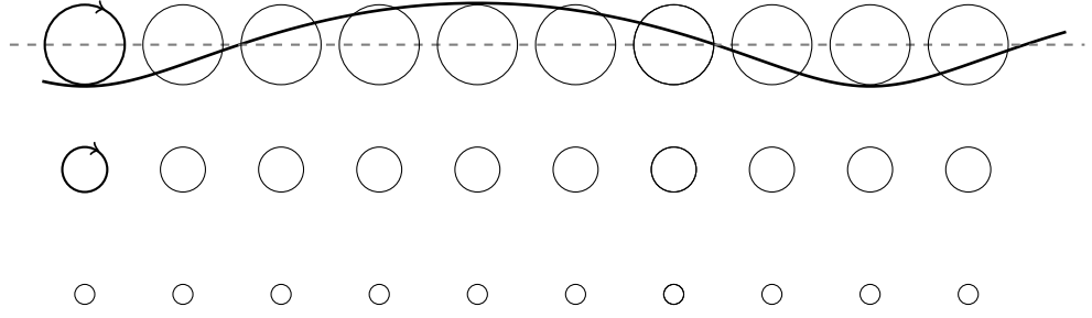
Figure 1.1: Circular paths of the particles in Gerstner's wave together with one of the possible profiles of the free surface
