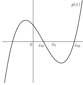
Figure 7.2: Sketch of the graph of the polynomial providing the dispersion relation for two negative vorticities under the condition (7.43). The root x_{01} does not satisfy the non-stagnation condition while the root x_{02} verifies it if and only if (7.47) is assumed.
