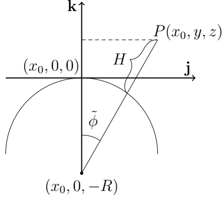
Figure 5.1: For a fixed x_0 , the height H corrects the deviation of the curved Earth's surface from the tangent plane considered in the \beta -plane approximation.
