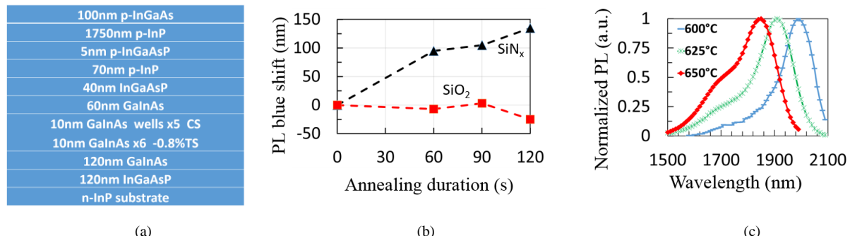
Fig. 1. (a) MQW structure under investigation, (b) PL blue shift at different anneal durations for different dielectric caps at annealing temperature of 650°C, and (c) Normalized PL spectra at different annealing temperatures for \text{SiN}_x capped samples for anneal duration of 120s.
