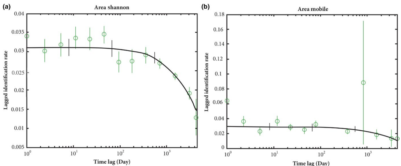
FIGURE 7 Lagged identification rate (LIR) for bottlenose dolphins encountered \geq 5 times (a) in the Shannon Estuary and (b) outside the Shannon Estuary in the coastal waters of Ireland during the study period 1996–2014. The graph describes the probability that a dolphin photographed at time 0 will be identified again at time X within the area. Data points are represented as green circles (with SE), and the best fitting model (see Supporting information Appendix S12) is displayed as the black solid line. Time lag (number of days) is given on logarithmic scale
