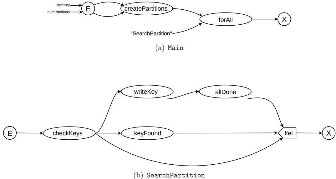
Figure 3.4: The graph definitions used in the RC5 key search ARC application.
