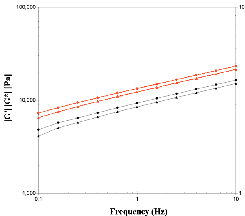
Figure 4-3: Frequency sweep of control batter and control with 5.5 % orange pomace batter (Black-control, orange-orange pomace). G' - \blacktriangle , G^* - \bullet .
