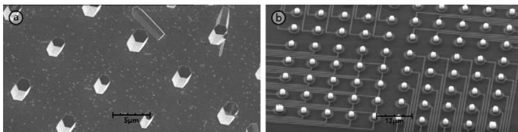
Fig. 1: a - array of single crystalline ZnO nanorods grown by hydrothermal method; b - array of singelly bottom contacted ZnO nanorod bunches before polymer encapsulation
