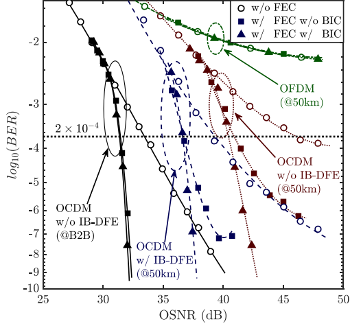
Fig. 2 Measured BER performance versus OSNR of the proposed BIC-IM/DD-OCDFM with IB-DFE and OFDM system.
