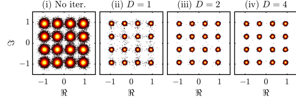
Fig. 4 Received constellation diagram of OCDFM signal 16-QAM (at 50-km, OSNR = 43 dB) recovered by IB-DFE with 0, 1, 2, and 4 iterations.
