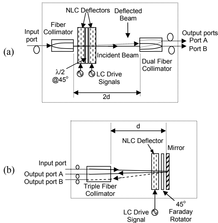
Fig. 7. Proposed NLC deflector based 1x2 switch designs using (a) a single fiber collimator, two parallel aligned NLC deflectors, a half wave plate and a dual fiber collimator, and (b) a triple fiber collimator and a single NLC deflector in a reflective mode.
