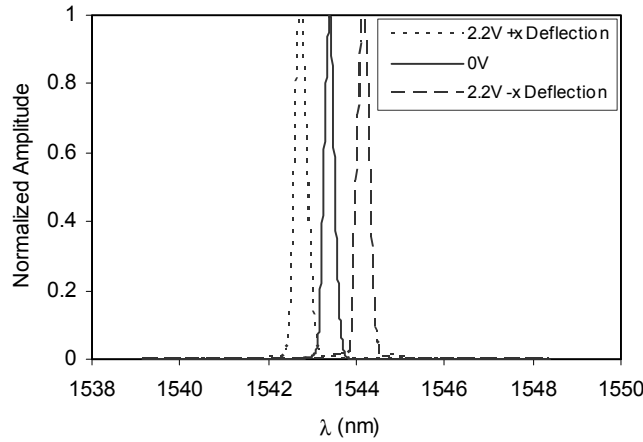
Fig. 6. Proposed Wavelength Tunable Variable Fiber-Optic Attenuator operating with precise fine wavelength selection using NLC deflector driven at three different operating states giving a 1.44 nm liquid crystal tuned fine wavelength range.
