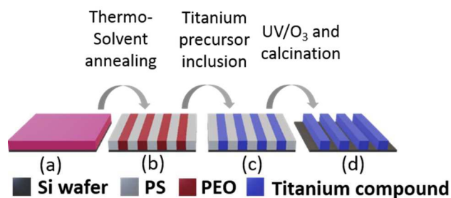
Scheme 1. Illustration of the formation of titanium dioxide nanowires. (a) As-cast thin film of PS- b -PEO solution on Si substrate; (b) self-assembled PS- b -PEO obtained after thermo-solvent annealing at 60°C in toluene vapors; (c) PS- b -PEO thin with SEO/TiO 2 hybrid and (d) titanium dioxide nanowires after UV/O 3 and calcination process.
