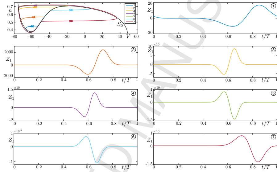
Figure 2: Top left panel: Canard orbits of the reduced HH system in the phase plane. Panels 1-7: time profile of the first component of the adjoint solution associated with each canard cycle shown in the phase plane (together with the critical manifold S_0 := \{\dot{V} = 0\} ), keeping the same color coding. A qualitative change in the adjoint solution occurs in between Orbit 4 and Orbit 5, corresponding to the passage through the maximal canard cycle.
