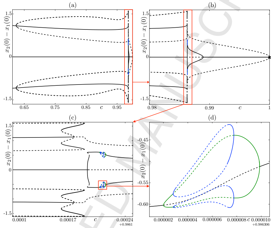
Figure 7: Bifurcation diagram of system (10) with respect to variations of c for \alpha = 10^{-5} , from the Hopf regime to the relaxation regime. The output solution measure is the difference between the first components of each oscillator at time t = 0 . The region of the maximal canard is enlarged from left to right and top to bottom panels. Black dots in panels (a) to (c) denote pitchfork bifurcation points; the black star in panel (b) corresponds to the double Hopf point that initiate the periodic regime in this coupled system; colored dots in panel (d) denote PD bifurcation points.
