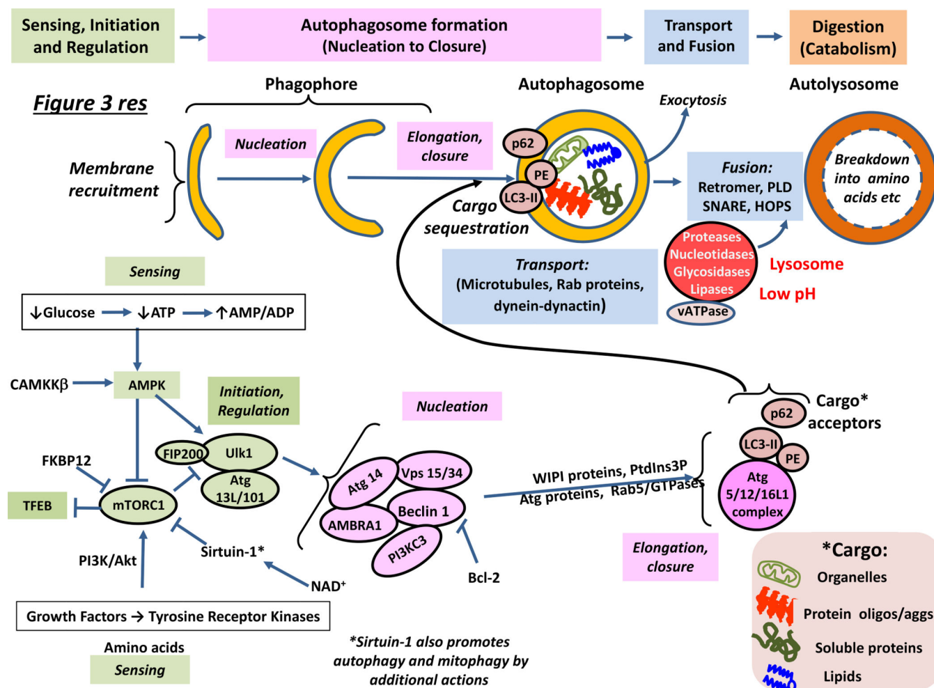
Figure 3 |. Organization, operation and regulation of the autophagic-lysosomal network. The top part of the figure illustrates the sequence of steps associated with operation of the ALN, while the bottom part shows the main regulatory proteins involved, focusing on potential targets for pharmacotherapy. ‘Sensing’ — both extrinsic (for example, glucose levels) and intrinsic ( e.g. for example, ATP/AMP levels) — can determine whether or not autophagy is initiated by activation of AMPK and/or inhibition of mTORC1, which leads to TFEB-driven transcription of ALN-requisite proteins. The pre-autophagosome (phagophore) structure first emerges from diverse membrane sources, and its formation is promoted by Atg9 (not shown). Nucleation is accomplished with the help of a complex cluster of proteins. Phosphatidylinositol-3-phosphate (PtdIns3P) is recognised by WIPI (WD-repeat-protein-interacting-with-phosphoInositides) proteins that help induce autophagosome elongation in association with several classes of Atg protein and small GTPases such as Rab5. With the aid of LC3 and cargo acceptors, autophagosomes take up cytoplasmic material such as aggregated proteins and dysfunctional mitochondria (Box 2). Autophagosomes and other autophagic vesicles are transported with the help of dynactin and dynein along microtubules towards acidic lysosomes. Autophagosomes fuse with lysosomes containing resident hydrolases that degrade their contents into amino acids, sugars and lipids for recycling. Exosomal release/secretion of neurotoxic proteins (“exocytosis”) may occur
