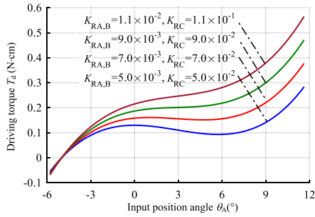
c Driving torque versus input position angle when K_R is great
