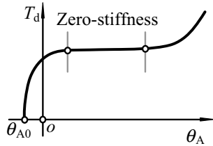
(c) Local zero-stiffness characteristic
