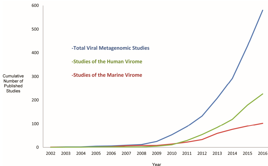
Figure 1. Graph illustrating the large increase in the publication of viral metagenomic studies from the initial study of Breitbart et al. [73] in 2002 to the end of 2016. The total cumulative number of studies is represented in blue. The number of metagenomic studies of the human virome is represented in green, and studies of the marine virome in red. The number of studies in each case was determined via Pubmed search.
