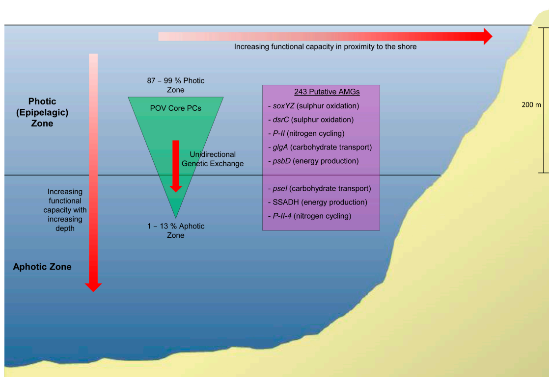
Figure 3. Functional richness of the ocean virome as determined by the Pacific Ocean Virome (POV) [106] and the Global Ocean Virome (GOV) [125] datasets. Analysis of functional diversity revealed that the functional richness of viral communities decreased in surface communities as distance from the coast increased and increased in the ocean as depth increased. It was also found that core PCs (protein clusters) of the POV (i.e., those present in all samples) are enriched in the photic zone relative to the aphotic zone, indicating unidirectional genetic exchange from surface waters to the deep ocean. Additionally, 243 putative auxiliary metabolic genes (AMGs) were identified, examples of which can be seen for each zone.
