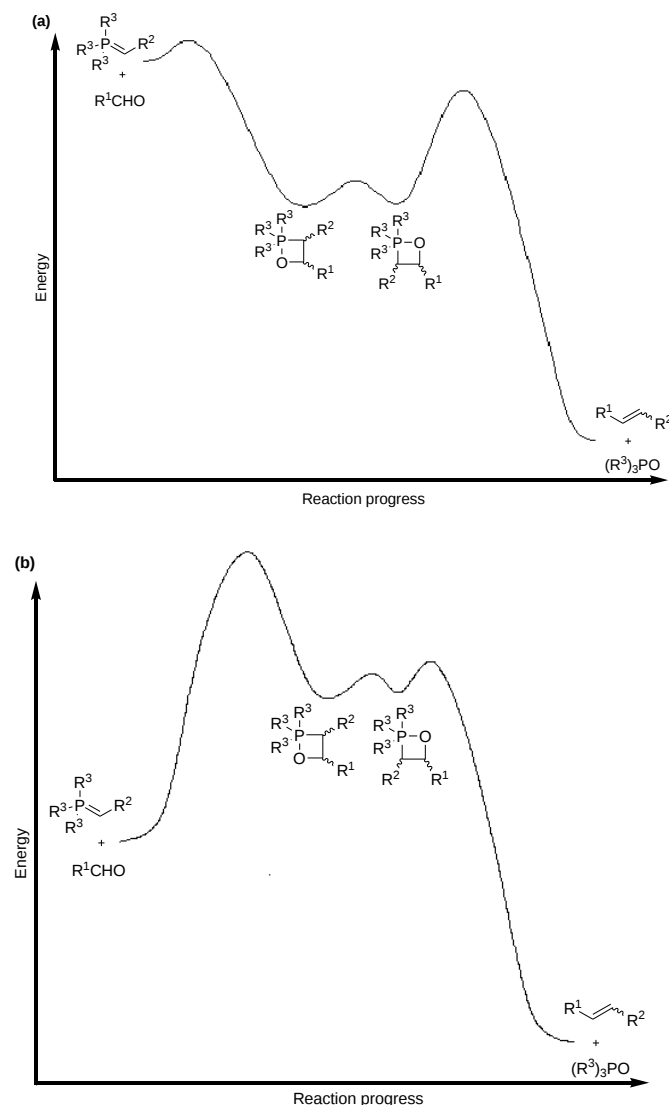
Figure 1. Reaction coordinate diagrams for Wittig reactions.
