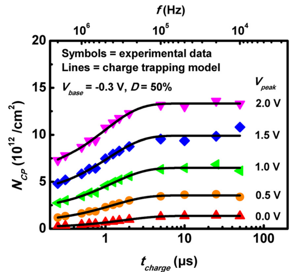
FIG. 6. N_{CP} plotted against f on the top x-axis and against t_{charge} = 1/(2f) on the bottom x-axis. The symbols show the experimental data obtained from the measurements performed on a 40- \mu\text{m} -channel-length device with V_{base} = -0.3 V and D = 50\% . The V_{peak} was varied from 0 V to 2 V. The lines represent the fitting of the data with the proposed charge trapping model (4).
