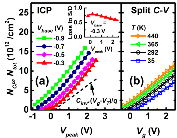
FIG. 4. (a) N_{CP} vs V_{peak} obtained from ICP performed on a 40- \mu\text{m} -channel-length device at f = 1 MHz and D = 50\% with V_{base} ranging from -0.3 V to -0.9 V. The D_{it} contribution to N_{CP} reduces as V_{base} is raised. The curves “curl up” and deviate from the theoretical C_{inv}(V_g - V_T)/q curve. (inset) Loss to S/D (1 - \alpha) vs V_{peak} obtained for V_{base} = -0.3 V. (b) N_{tot} vs V_g obtained by split C - V at f = 1 MHz over a range of T going from 440 K to 35 K. The D_{it} contribution to N_{tot} reduces as T is reduced.
