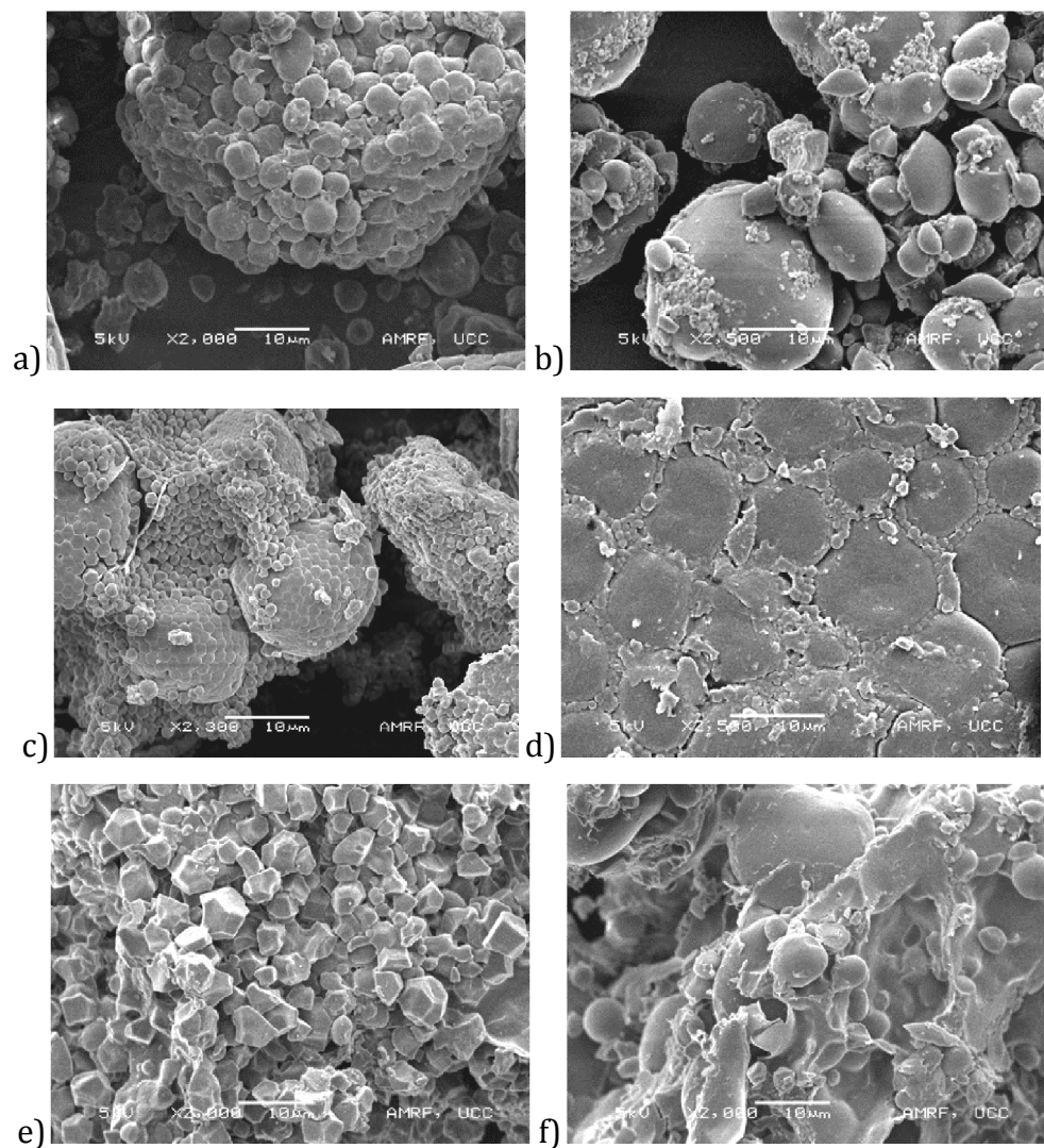
Figure 6-2 Scanning electron micrographs of flours from a) buckwheat, b) oat, c) quinoa , d) sorghum, e) teff and f) wheat. Scale bar represents 10 \mu\text{m} .
