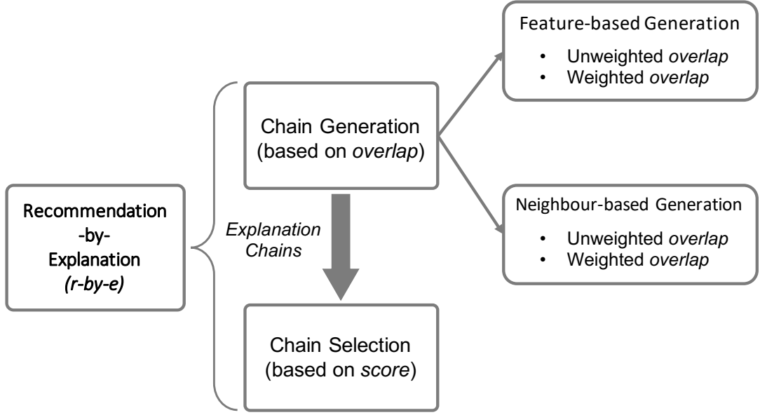
Figure 5.1: Extended Recommendation-by-Explanation
