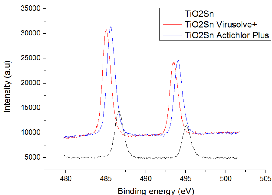
Figure 5.6: Sn 3d peak shifts for the unexposed Ti_{1-x}O_2:Sn_x (19:1) film, the Ti_{1-x}O_2:Sn_x (19:1) film exposed to Virusolve + TM and the Ti_{1-x}O_2:Sn_x (19:1) film exposed to Actichlor Plus TM .
