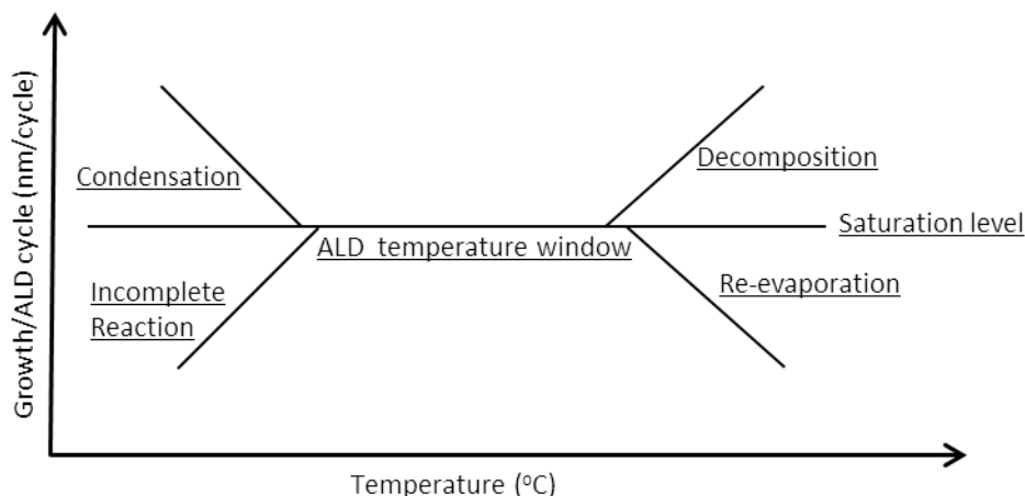
Figure 2.2: ALD temperature window [407]
