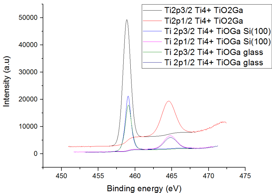
Figure 6.33: \text{Ti}^{4+} 2p 3/2 and 1/2 peaks shifts for the PEALD grown Ga-capped \text{Ti}_{1-x}\text{O}_2:\text{Ga}_x (99:1) films on glass and silicon as compared to thermal ALD grown \text{Ti}_{1-x}\text{O}_2:\text{Ga}_x (99:1).
