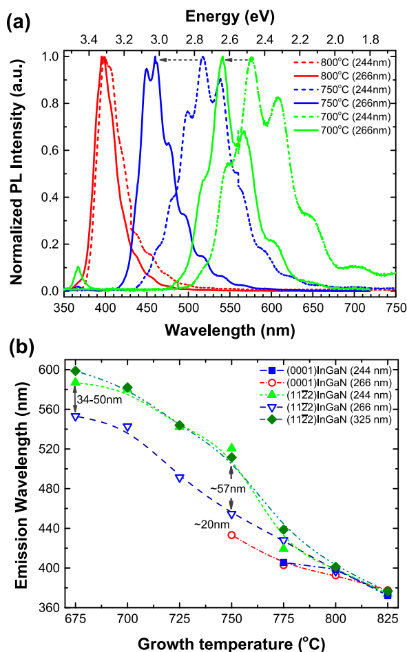
FIG. 4. (a) RT-PL spectra measured with 244 nm CW (dashed lines) and 266 nm (solid lines) pulsed excitation lasers of the (112 \bar{2} ) InGaN layers grown at different temperatures. (b) The RT-PL peak emission wavelength of the (0001) and (112 \bar{2} ) InGaN layers measured with 325, 244, and 266 nm excitation sources.
