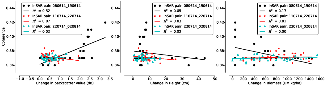
Figure 3: Relationship of calculated coherence with backscatter value, grass height and biomass of three SAR interferometric pairs with 11 days baseline (black = 080614_190614, red = 110714_220714 and cyan = 220714_020814).
