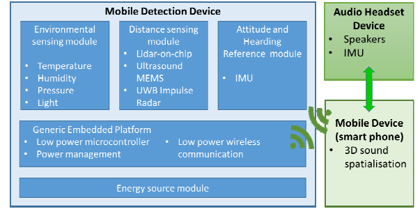
Fig. 5. INSPEX smart integrated system architecture (first attempt).
