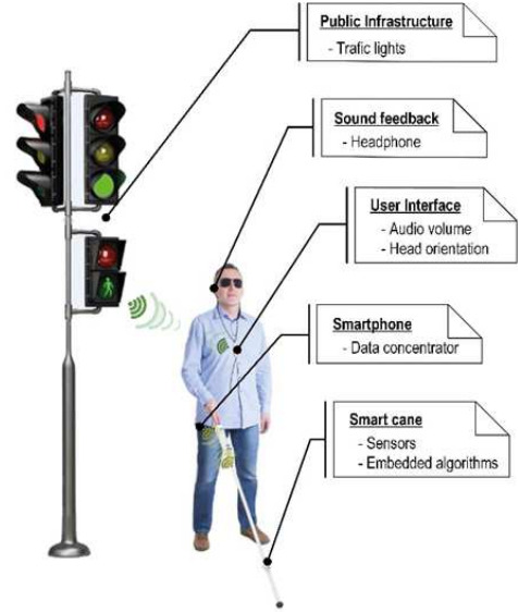
Fig. 2. INSPEX initial demonstrator.
