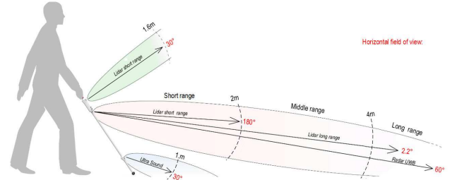
Fig. 6. Coverage of the different range sensors integrated in the white cane
