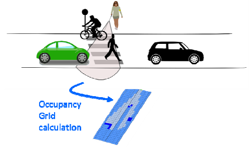
Fig. 3. Detection of obstacles with heterogeneous range sensors and Occupancy Grid obtained by data fusion.
