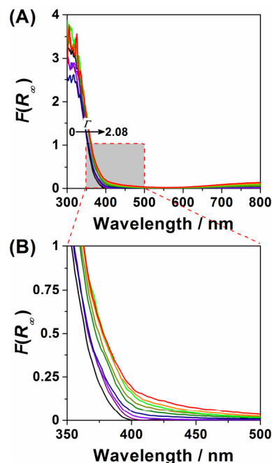
Figure 4. UV-visible absorption spectra of the samples prepared by the CCC technique: F(R_s) denotes the Kubelka-Munk function.
