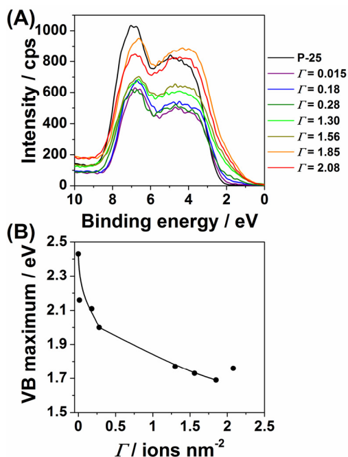
Figure 8. (A) VB-XP spectra for CuO/P-25. (B) Change in the position of the VB maximum level as a function of CuO loading ( \Gamma ).
